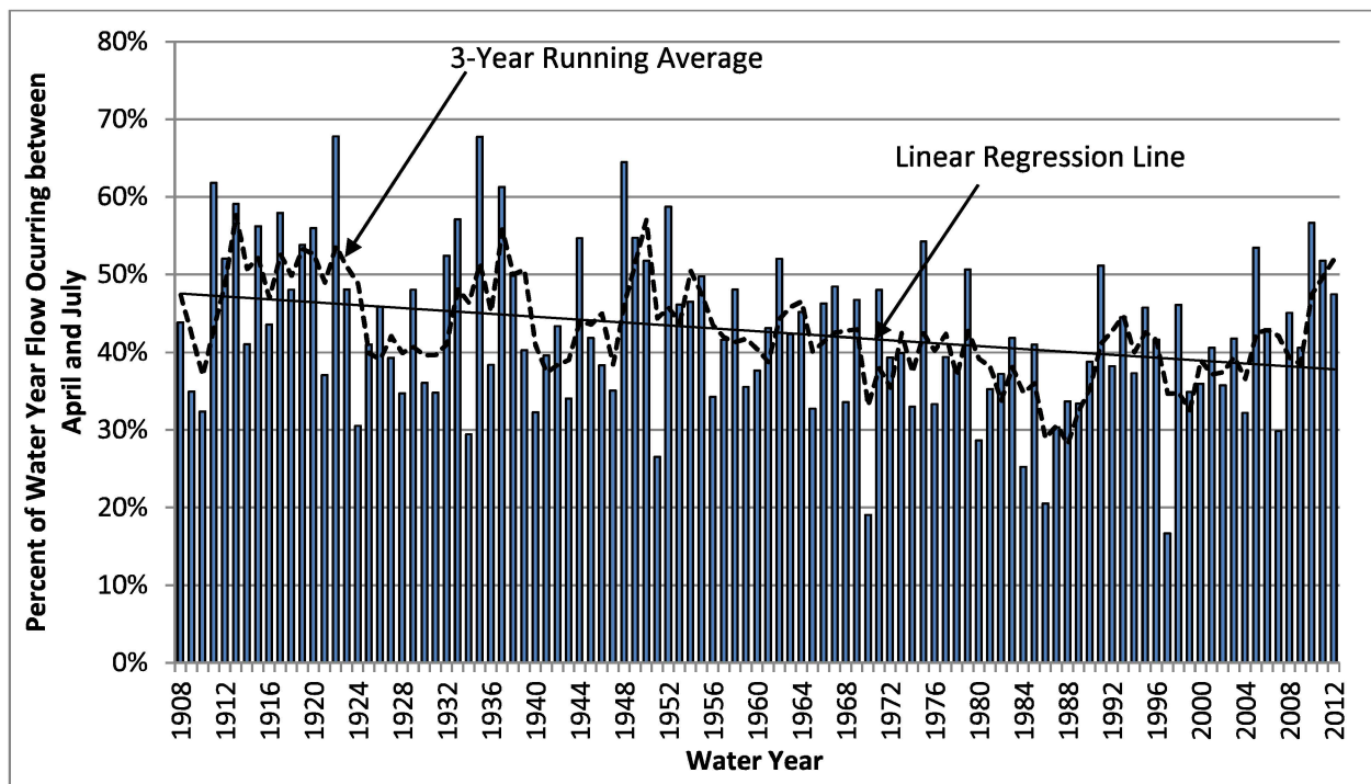
Figure 5.1. Annual April through July Full Natural Flow for Feather River at Oroville as Percentage of Water Year Full Natural Flow.
