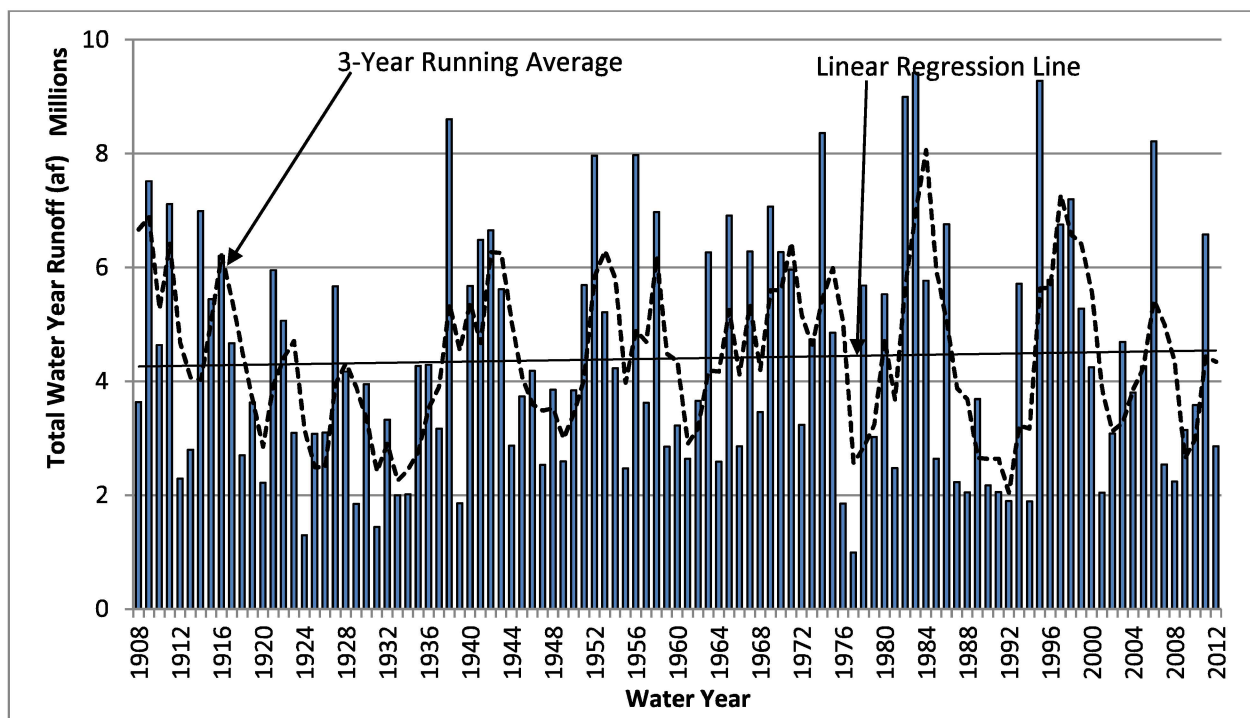
Figure 5.2. Water Year Full Natural Flow for Feather River at Oroville.
