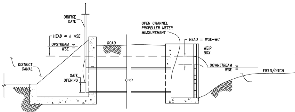
Figure 1. Typical Gravity Delivery Farm Turnout Configuration.
