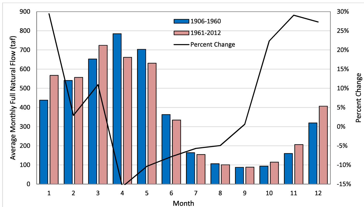
Figure 5.3. Mean Monthly Full Natural Flow and Percent Change, 1906-1960 and 1961-2012.
