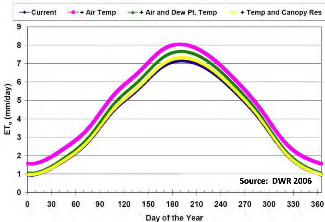
Figure 5.5. Sensitivity of Reference Evapotranspiration to Hypothetical Changes in Climate.
