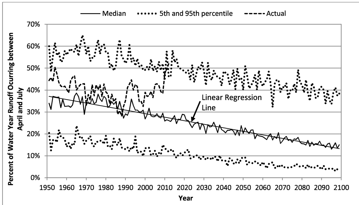
Figure 5.4. Projected (1950 - 2100) and Actual (1950 - 2012) Annual April through July Full Natural Flow for Feather River at Oroville as Percentage of Water Year Full Natural Flow (USBR 2011).
