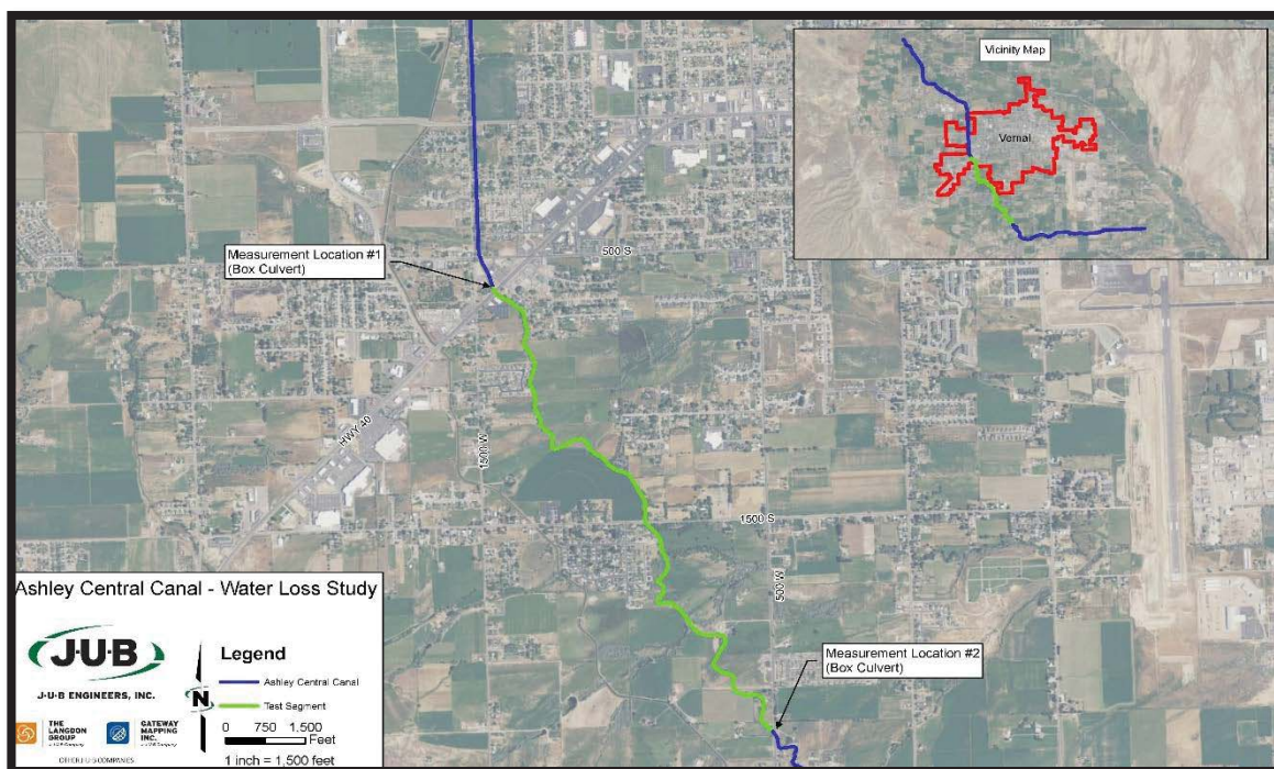
Figure 2 Measurement Locations for Water Loss Study
