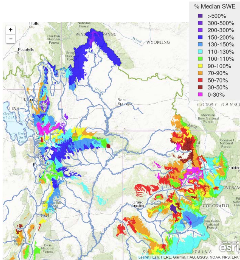
FIGURE 2. Upper Green River Basin modeled SWE significant areas as of March 27, 2017.
