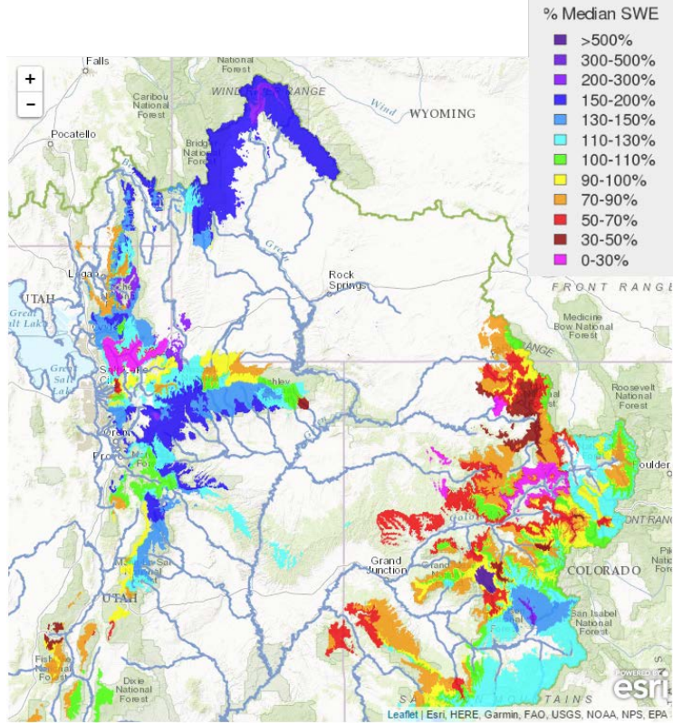
FIGURE 7. Yampa River Basin modeled SWE significant areas as of March 27, 2016.
