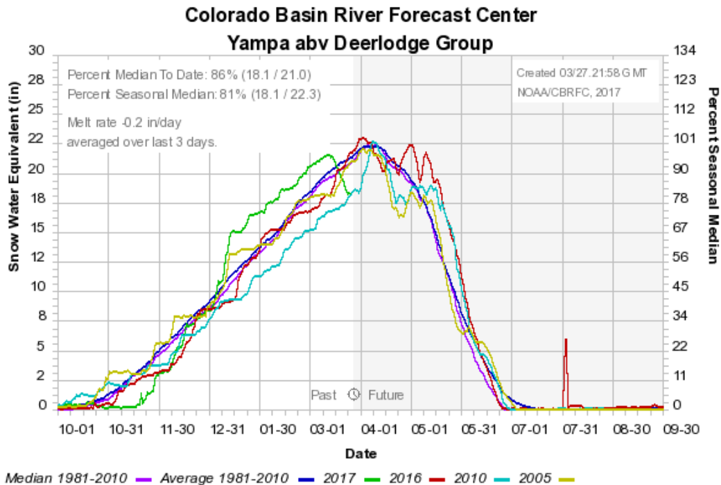
FIGURE 6. Yampa River above Deerlodge SNOTEL Group. 1981-2010 percent of average SWE compared against 2017 YTD, and analog years 2005, 2010, and 2016 percent of median SWE
