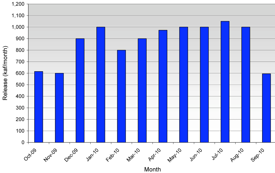
Figure 1. (Top) Proposed Water Year (WY) 2010 Lake Powell monthly release volumes in thousand acre feet (kaf/month) under most probable (median) inflow scenario). (Bottom) Proposed WY 2010 Glen Canyon Dam daily release regime in cubic feet per second (cfs) under most probable (median) inflow scenario. Projections from Bureau of Reclamation’s 24-month study as of July 10, 2009 (subject to revision).
