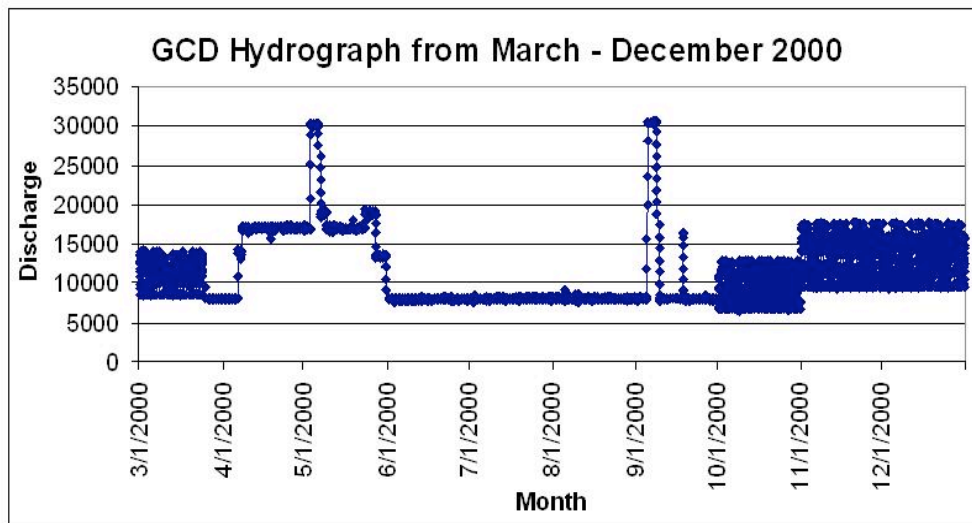
Figure 5. Hydrograph from March–December 2000 including discharge pattern associated with the LSSF experiment.
