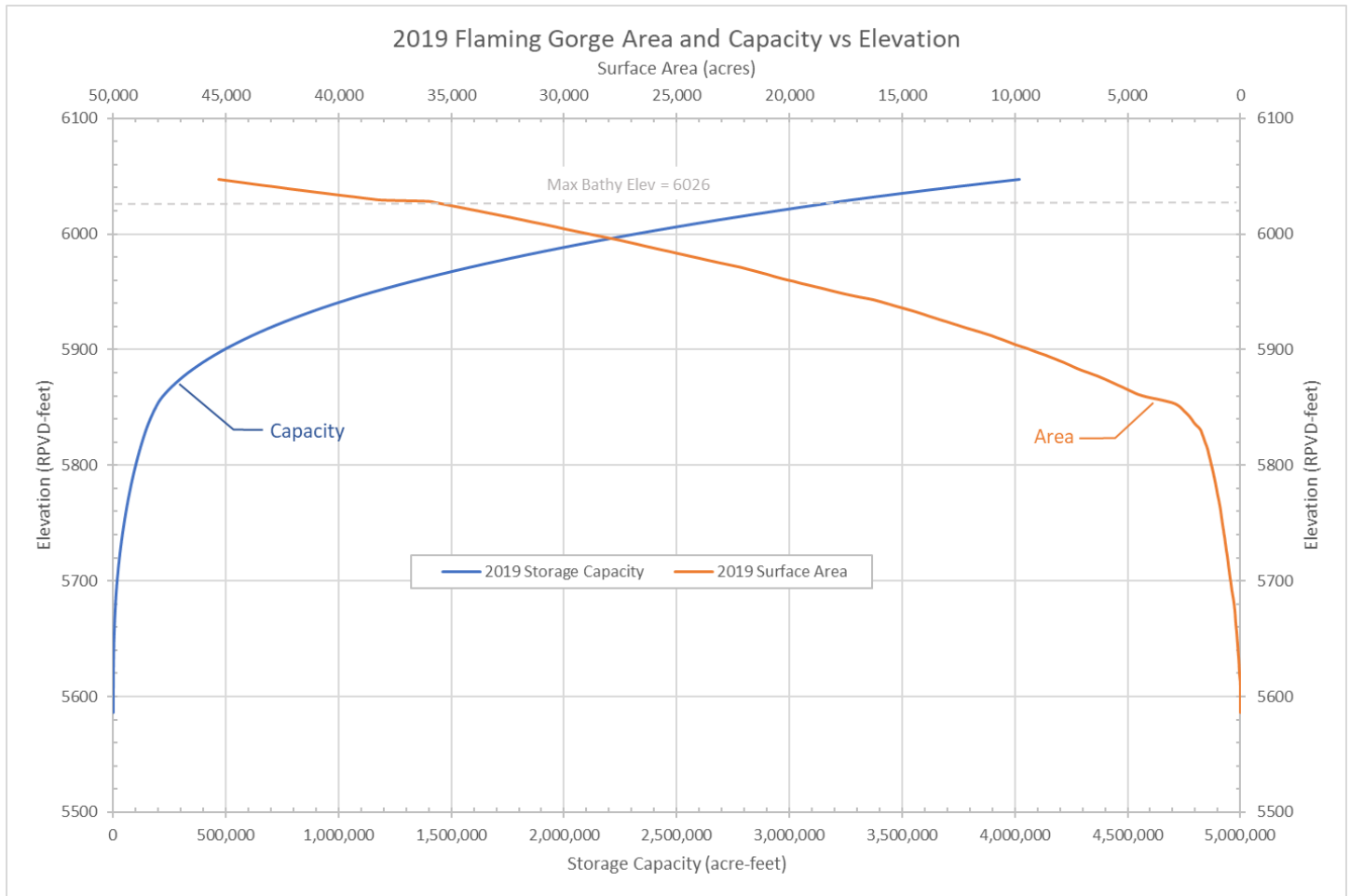
Figure 1. Flaming Gorge Reservoir surface area and storage capacity curves based on the 2019 survey. Use the elevation axes to find the storage capacity (blue curve, bottom axis) or surface area (orange curve, top axis) for a given reservoir elevation.
