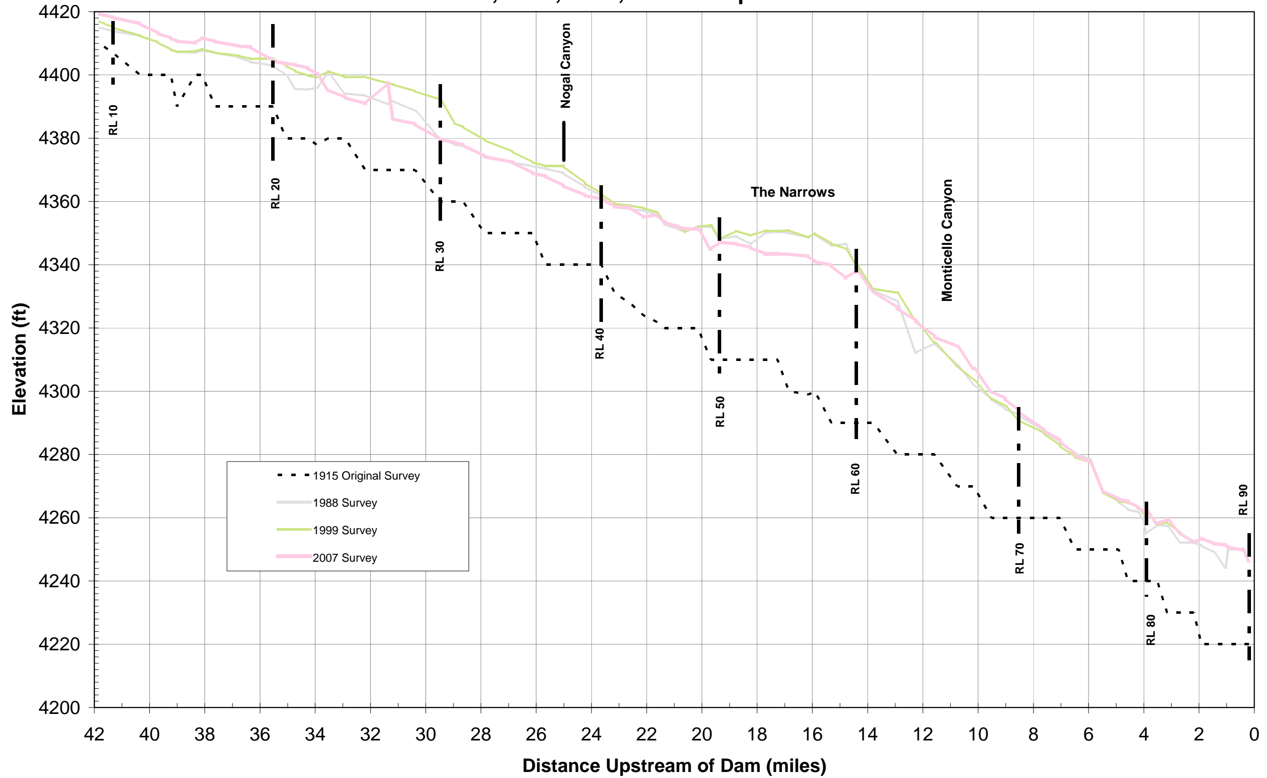
Figure 95 - Elephant Butte Reservoir Longitudinal Profiles.
