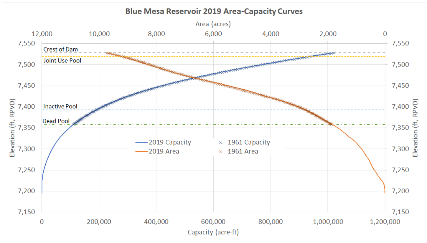
Figure 1. Blue Mesa Reservoir surface area and storage capacity curves based on the 2019 survey. Use the elevation axes to find the storage capacity (blue curve, bottom axis) or surface area (orange curve, top axis) for a given reservoir elevation.
