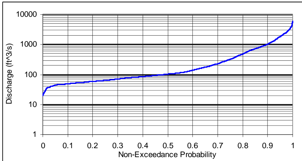
Figure 10-1 Site Specific Example of a Mean Daily Flow Duration Curve
