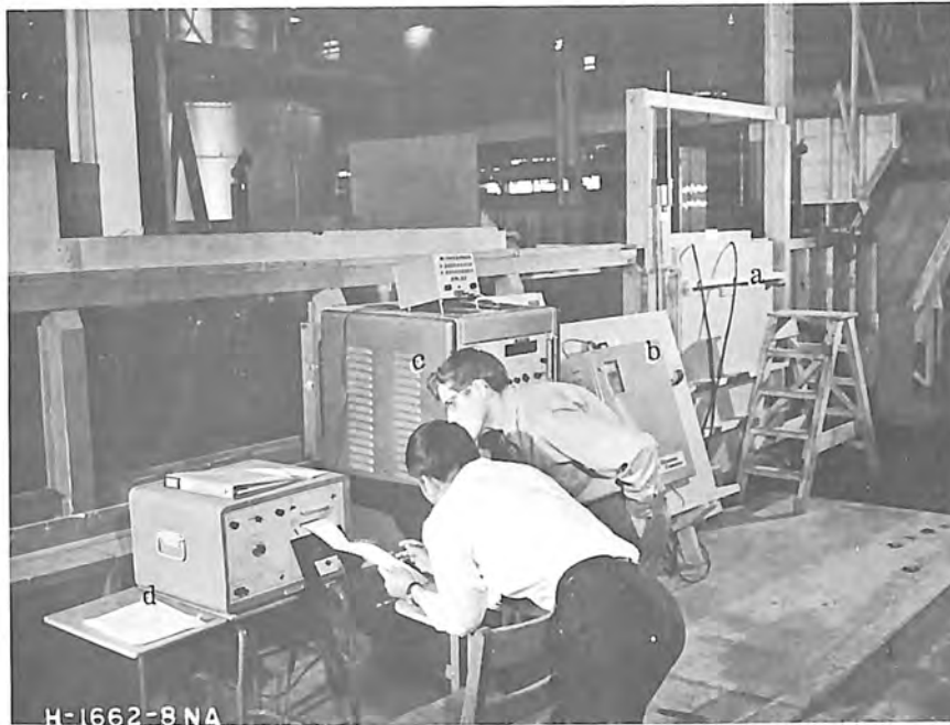
Figure 5. Ultrasonic flowmeter installation. (a). Transducer section (b). Flowmeter electronics. (c). Integrating digital voltmeter. (d). Tape printer. Photo PX-D-72009
