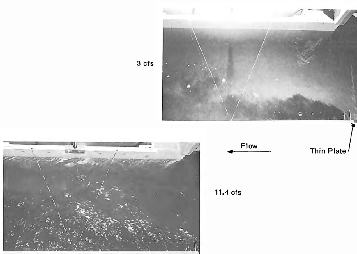
Figure 10. Ultrasonic path and wake behind plate normal to flow. Photos PX-D-72015 and PX-D-72014.
