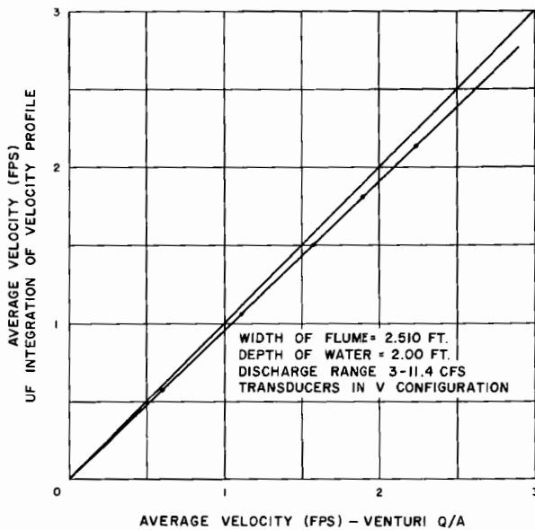
Figure 8. Average velocity-Ultrasonic flowmeter and venturi meter discharge.
