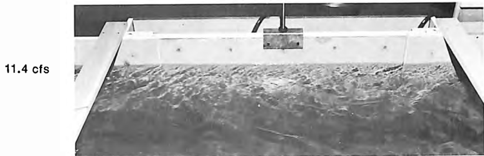
Figure 7. Increase in surface waves with increasing flow. Photos PX-D-72013 and PX-D-7212.
