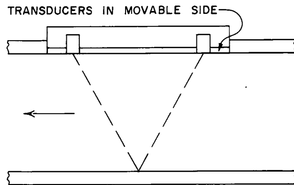
Figure 2. V installation form for laboratory
