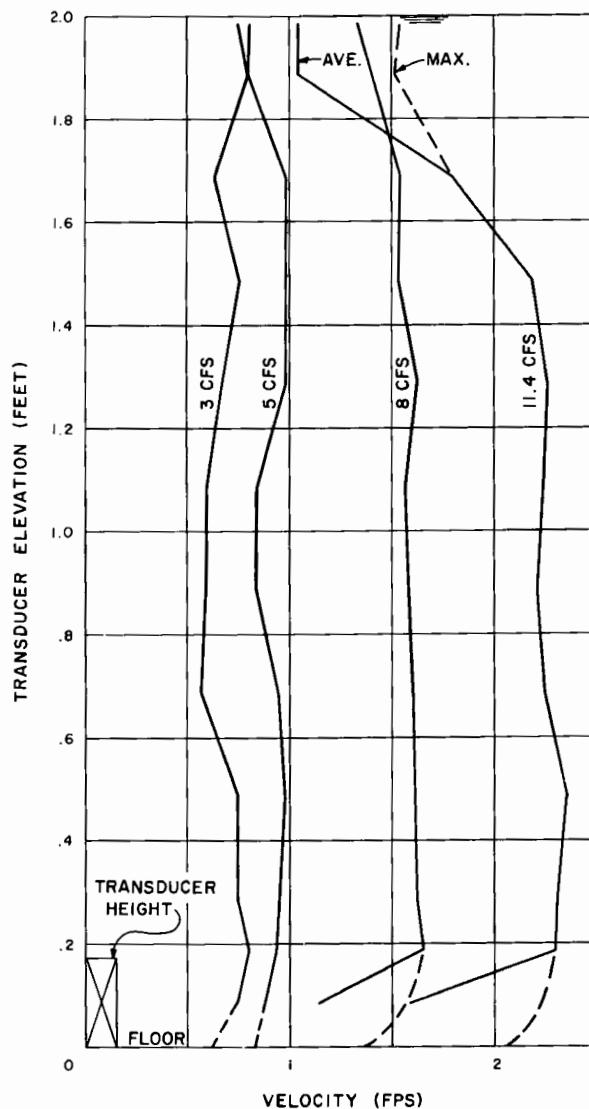
Figure 9. Ultrasonic flowmeter velocity profiles (unsymmetrical distribution).
