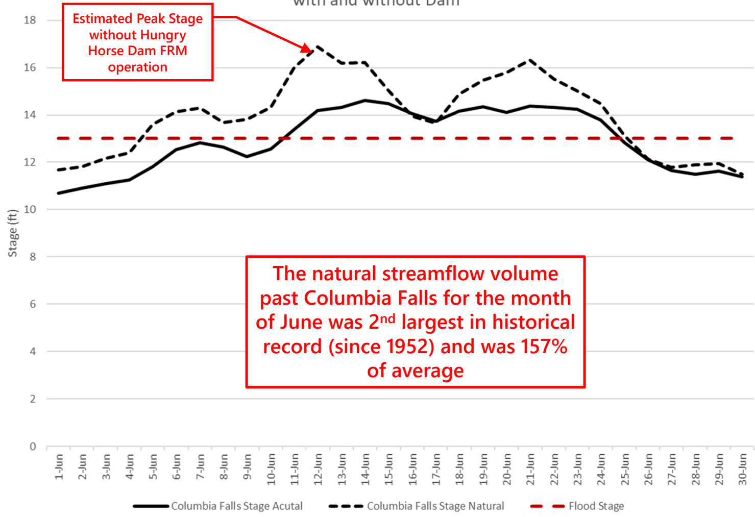
Daily Average Columbia Falls Stage Actual vs Natural (Estimated) with and without Dam
