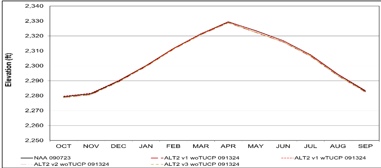
Figure S-15. Trinity Reservoir Alternative 2 Long-Term Average Water Level Elevation
