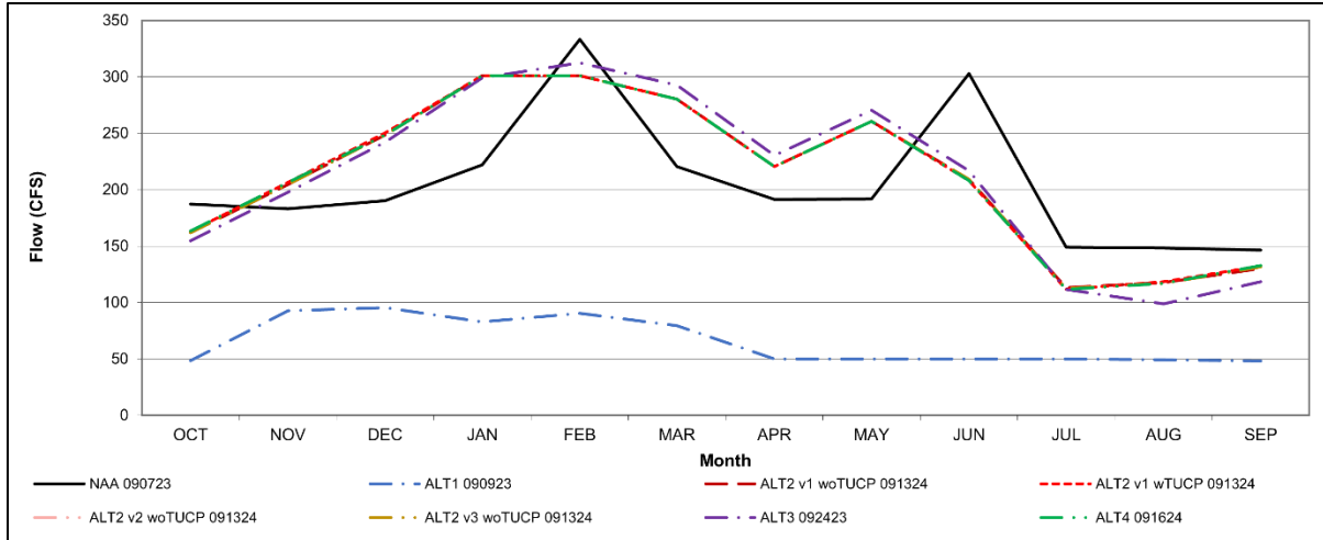
Figure S-6. Clear Creek Flow below Whiskeytown Dam Long-Term Average Flow
