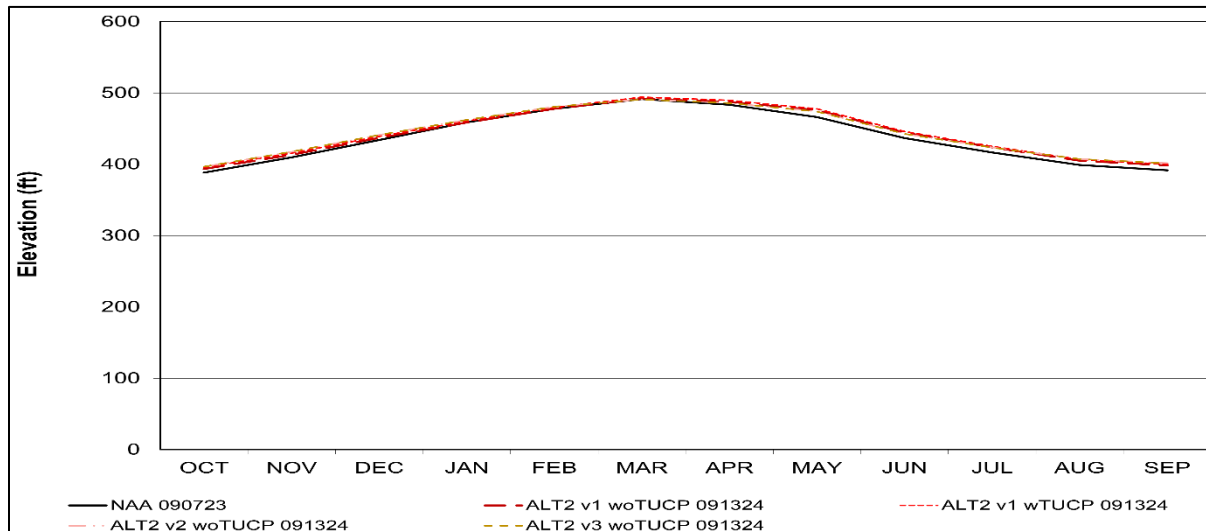
Figure S-29. San Luis Reservoir Alternative 2 Long-Term Average Water Level Elevation
