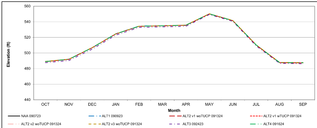
Figure S-12. Millerton Reservoir Long-Term Average Water Level Elevation
