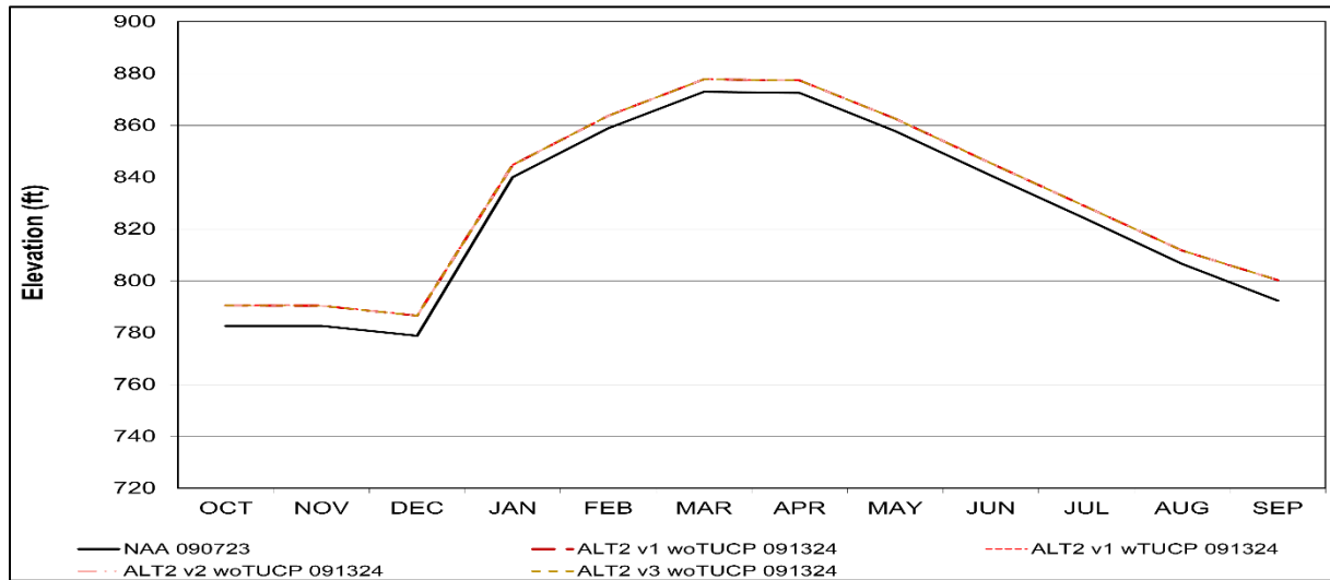
Figure S-26. New Melones Reservoir Alternative 2 Long-Term Average Minimum Water Level Elevation
