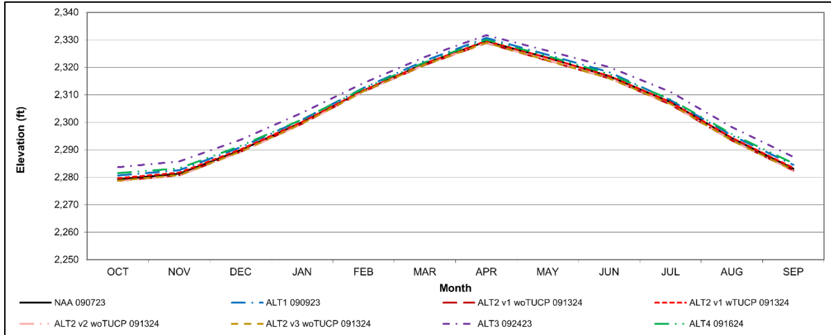
Figure S-1. Trinity Reservoir Long-Term Average Water Level Elevation
