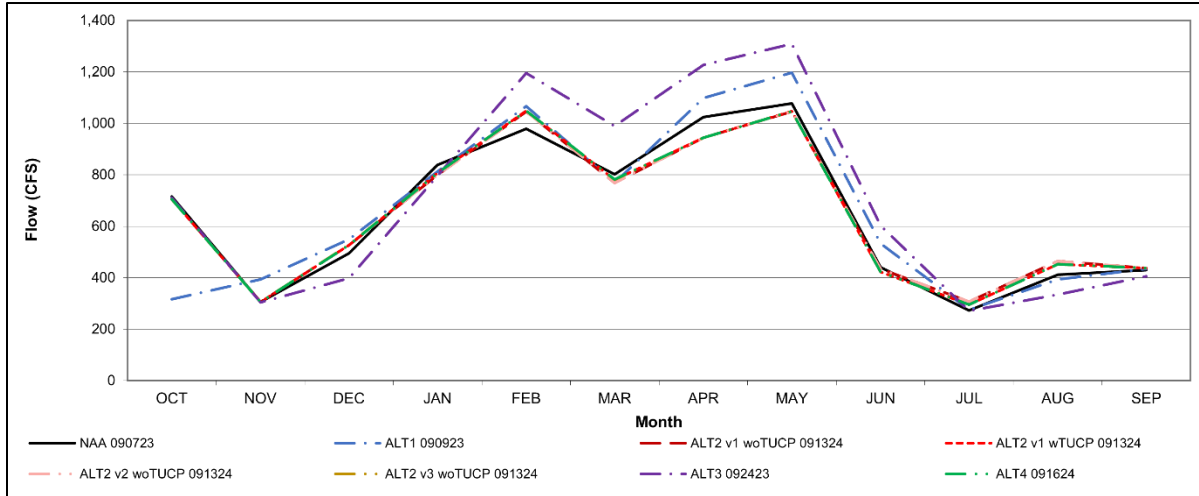
Figure S-11. Stanislaus River Flow below Goodwin Long-Term Average Flow
