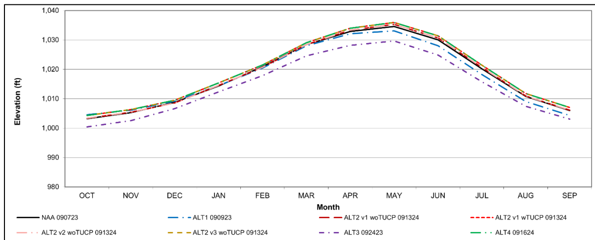
Figure S-10. New Melones Reservoir Long-Term Average Water Level Elevation
