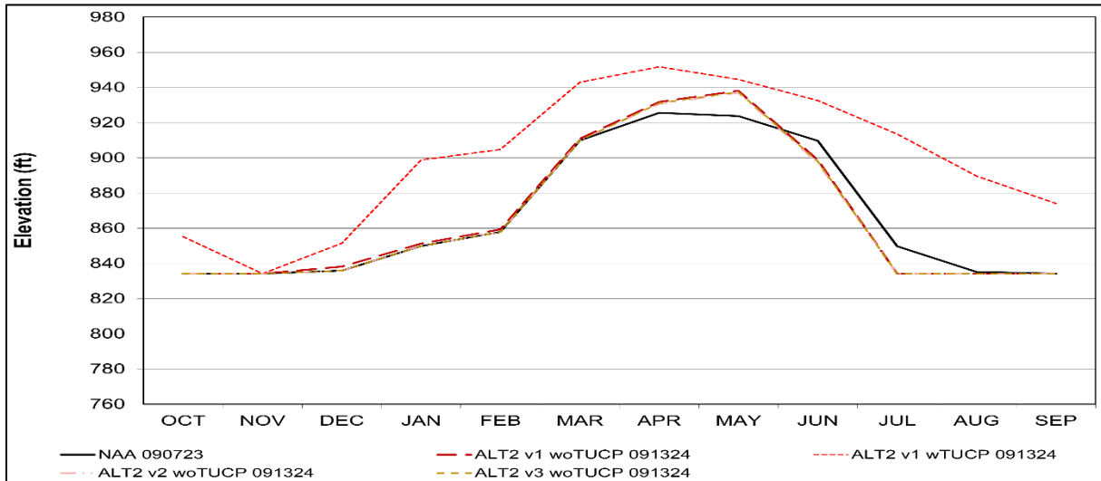
Figure S-19. Shasta Reservoir Alternative 2 Long-Term Average Minimum Water Level Elevation
