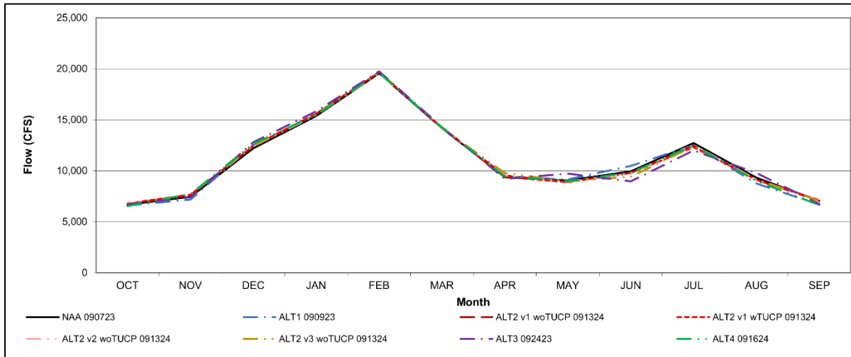
Figure S-5. Sacramento River Long-Term Average Flow Below Red Bluff Diversion Dam
