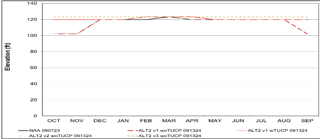
Figure S-24. Lake Natoma Alternative 2 Long-Term Average Minimum Water Level Elevation
