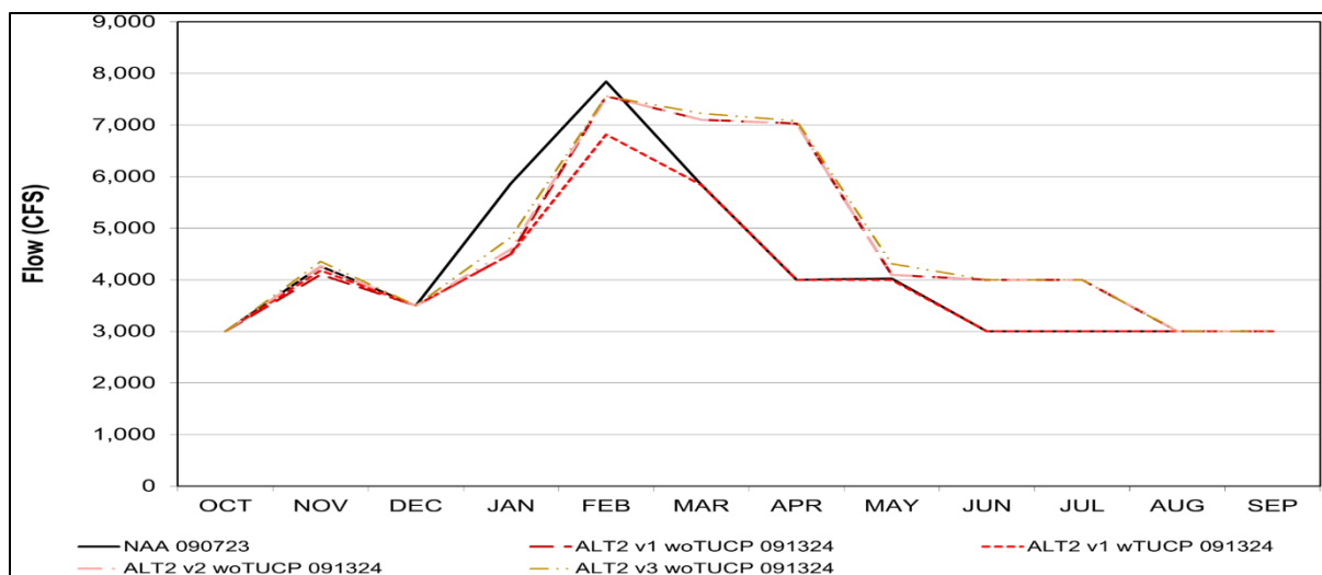
Figure S-28. Bay-Delta Alternative 2 Long-Term Average Minimum Outflow
