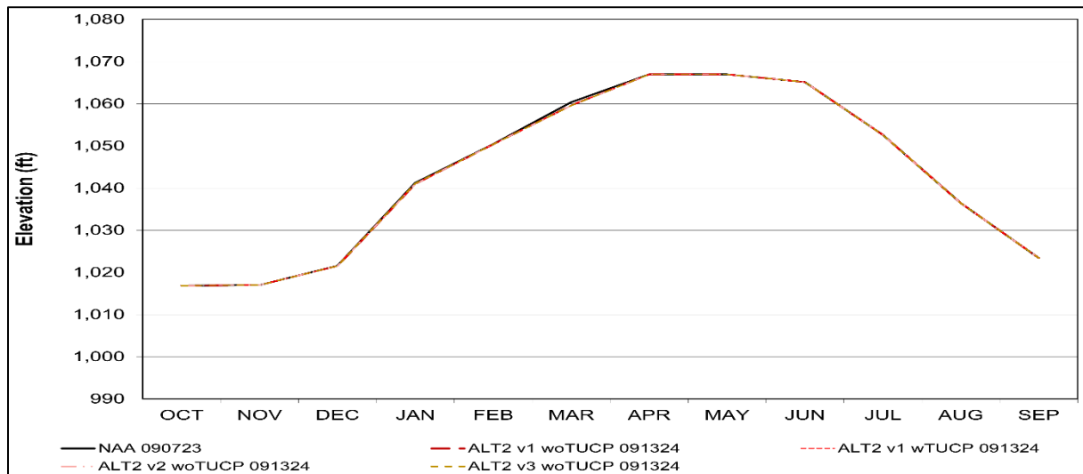
Figure S-20. Shasta Reservoir Alternative 2 Long-Term Average Maximum Water Level Elevation
