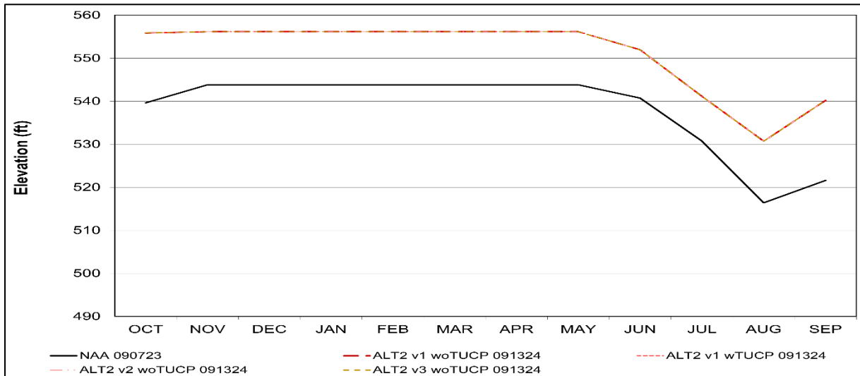
Figure S-31. San Luis Reservoir Alternative 2 Long-Term Average Maximum Water Level Elevation
