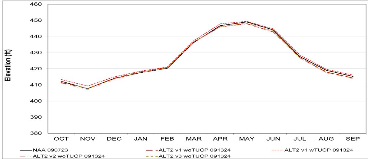
Figure S-21. Folsom Reservoir Alternative 2 Long-Term Average Water Level Elevation
