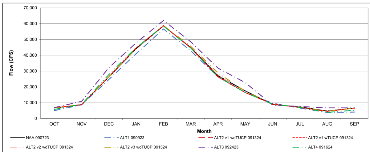
Figure S-13. Bay-Delta Long-Term Average Outflow
