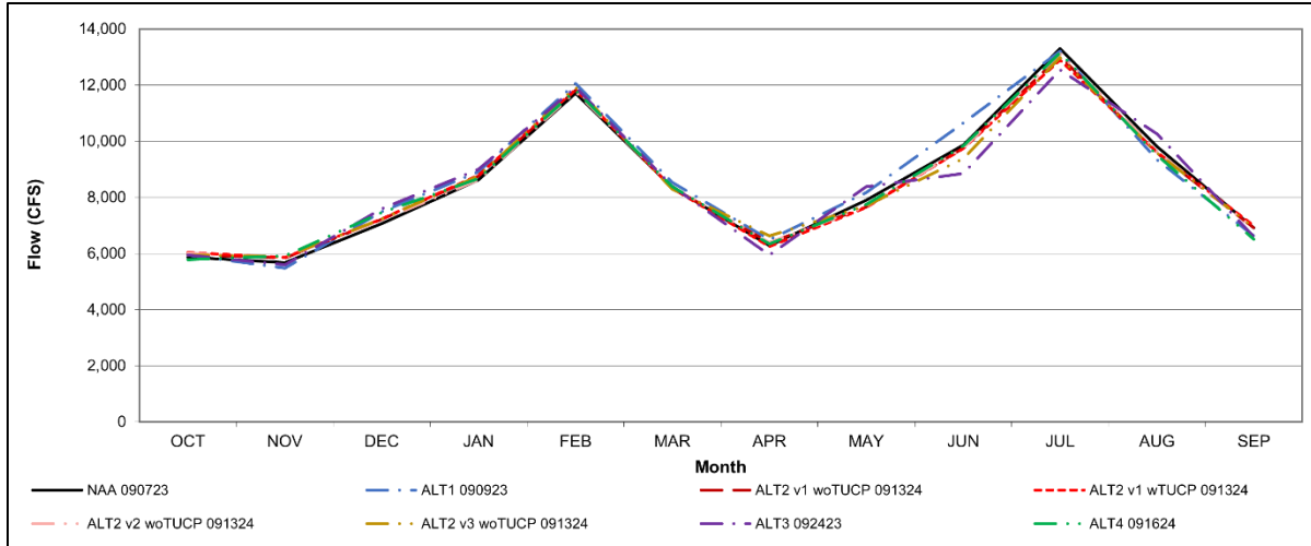
Figure S-4. Sacramento River Long-Term Average Flow Downstream of Keswick Reservoir
