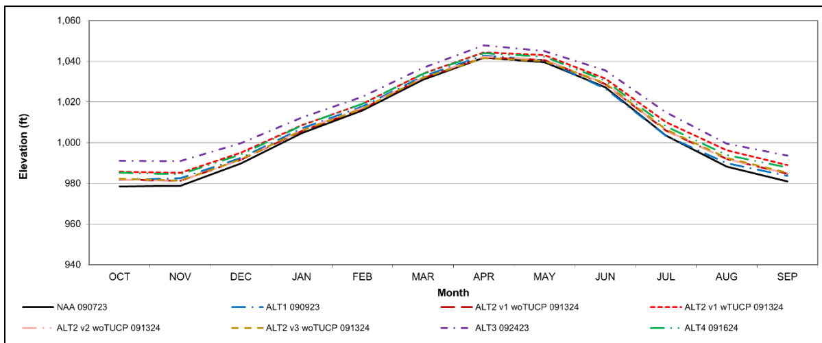
Figure S-2. Shasta Reservoir Long-Term Average Water Level Elevation
