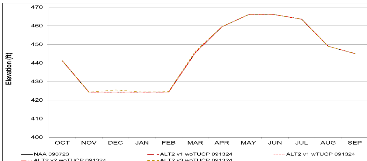
Figure S-23. Folsom Reservoir Alternative 2 Long-Term Average Maximum Water Level Elevation
