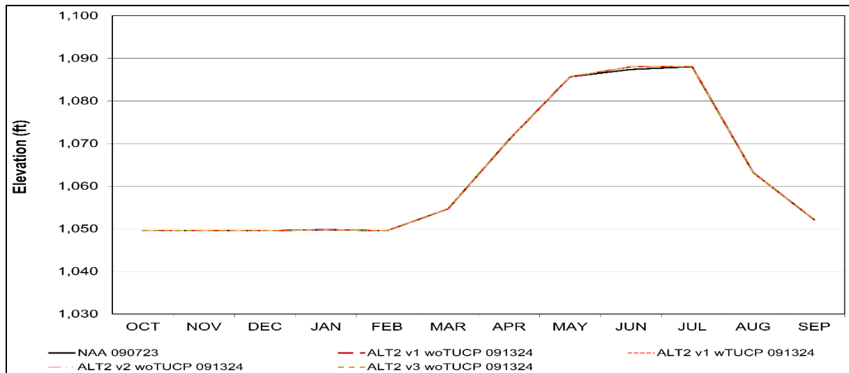
Figure S-27. New Melones Reservoir Alternative 2 Long-Term Average Maximum Water Level Elevation
