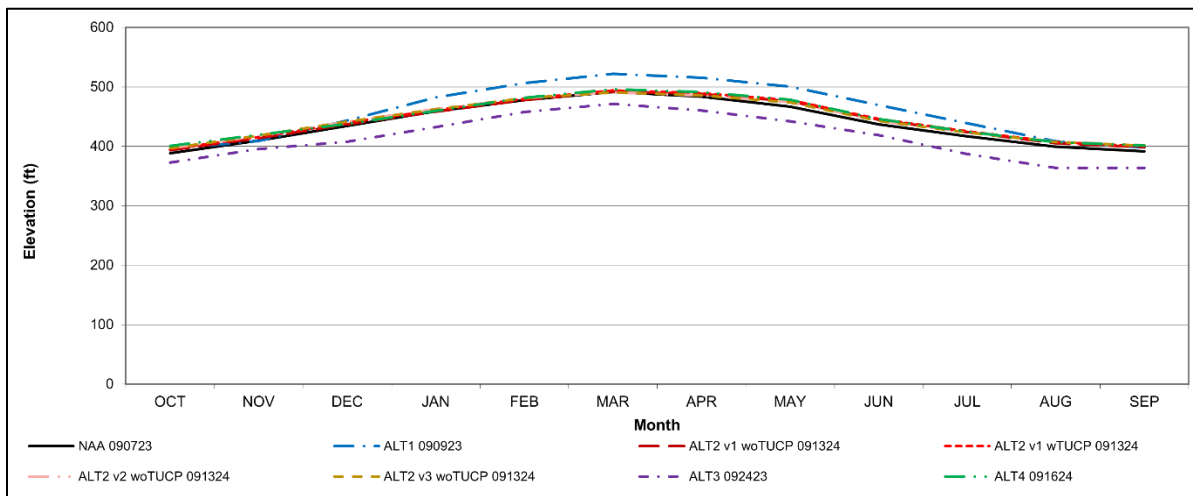
Figure S-14. San Luis Reservoir Long-Term Average Water Level Elevation
