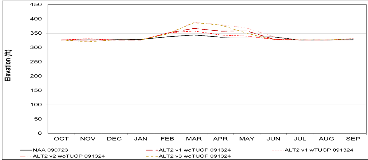
Figure S-30. San Luis Reservoir Alternative 2 Long-Term Average Minimum Water Level Elevation
