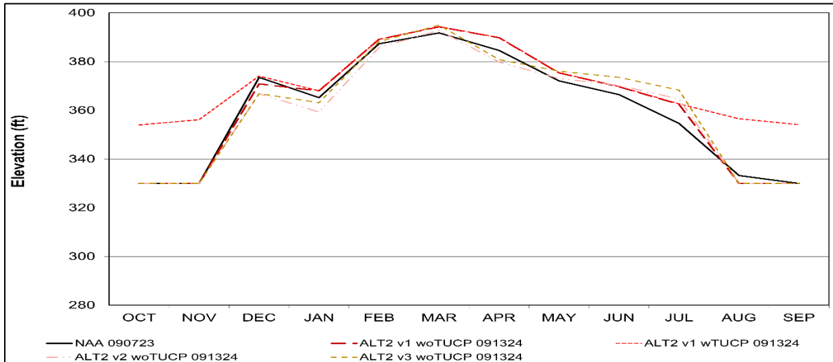
Figure S-22. Folsom Reservoir Alternative 2 Long-Term Average Minimum Water Level Elevation
