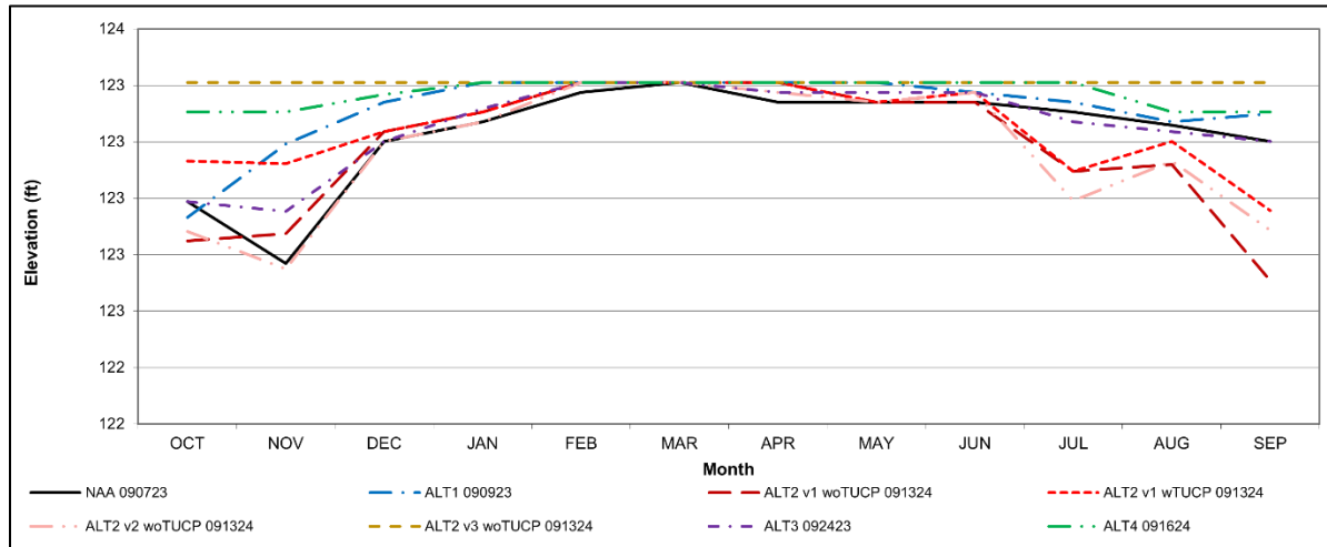
Figure S-8. Lake Natoma Long-Term Average Water Level Elevation
