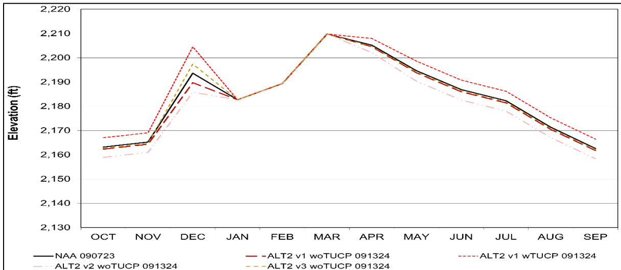
Figure S-16. Trinity Reservoir Alternative 2 Long-Term Average Minimum Water Level Elevation
