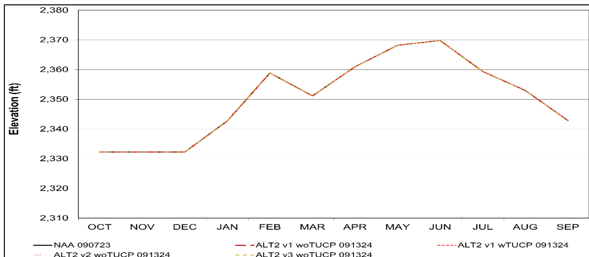
Figure S-17. Trinity Reservoir Alternative 2 Long-Term Average Maximum Water Level Elevation
