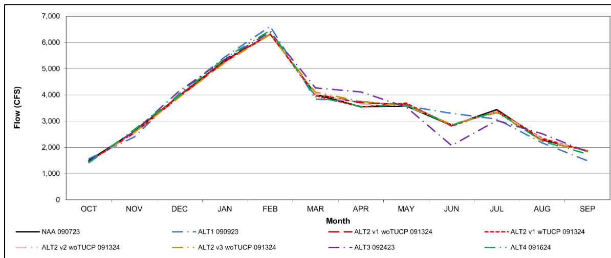
Figure S-9. American River Average Flow below Nimbus Dam
