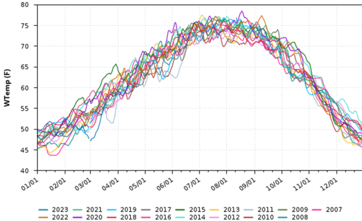
Figure B-86. Prisoners Point Daily Average Water Temperature (°F) for WY 2007–2023
