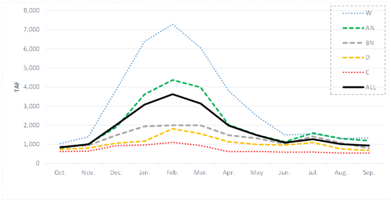
Figure B-73. Inflows to the Central Valley by Month and Water Year Type (Proposed Action)
