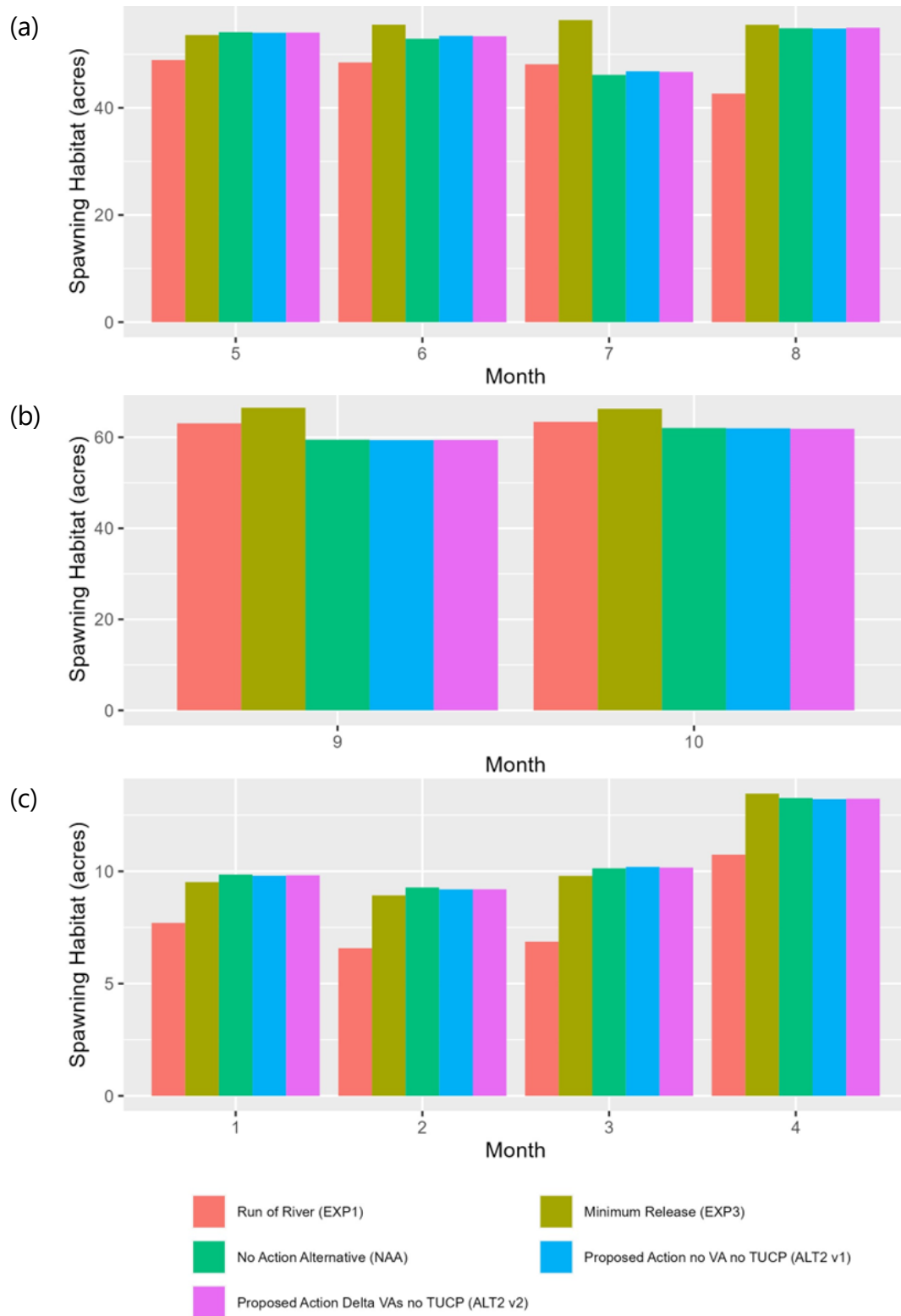
Figure B-25. Estimated Spawning Habitat Area for Adult Winter-run Chinook Salmon (a), Spring-run Chinook Salmon (b), and Steelhead (c) in the Upper Sacramento River
