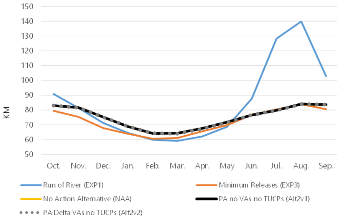
Figure B-91. Location of X2
