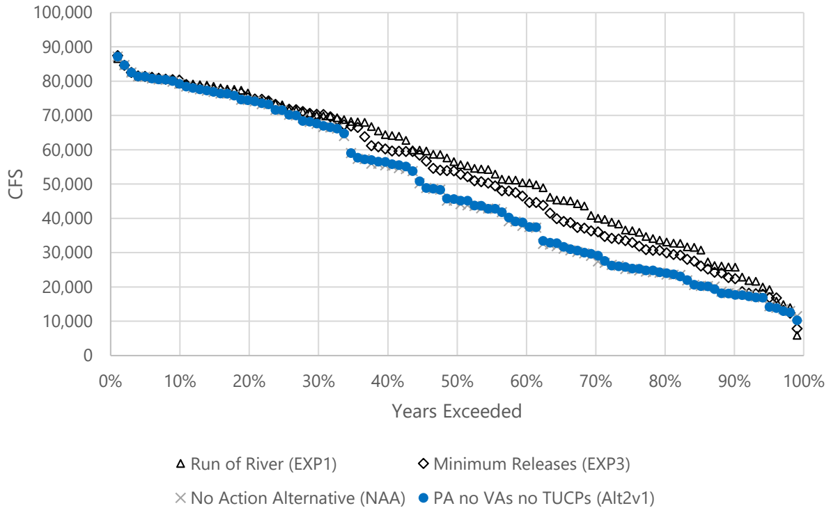
Figure B-82. Sacramento River at Freeport Annual Peak Flow Frequency
