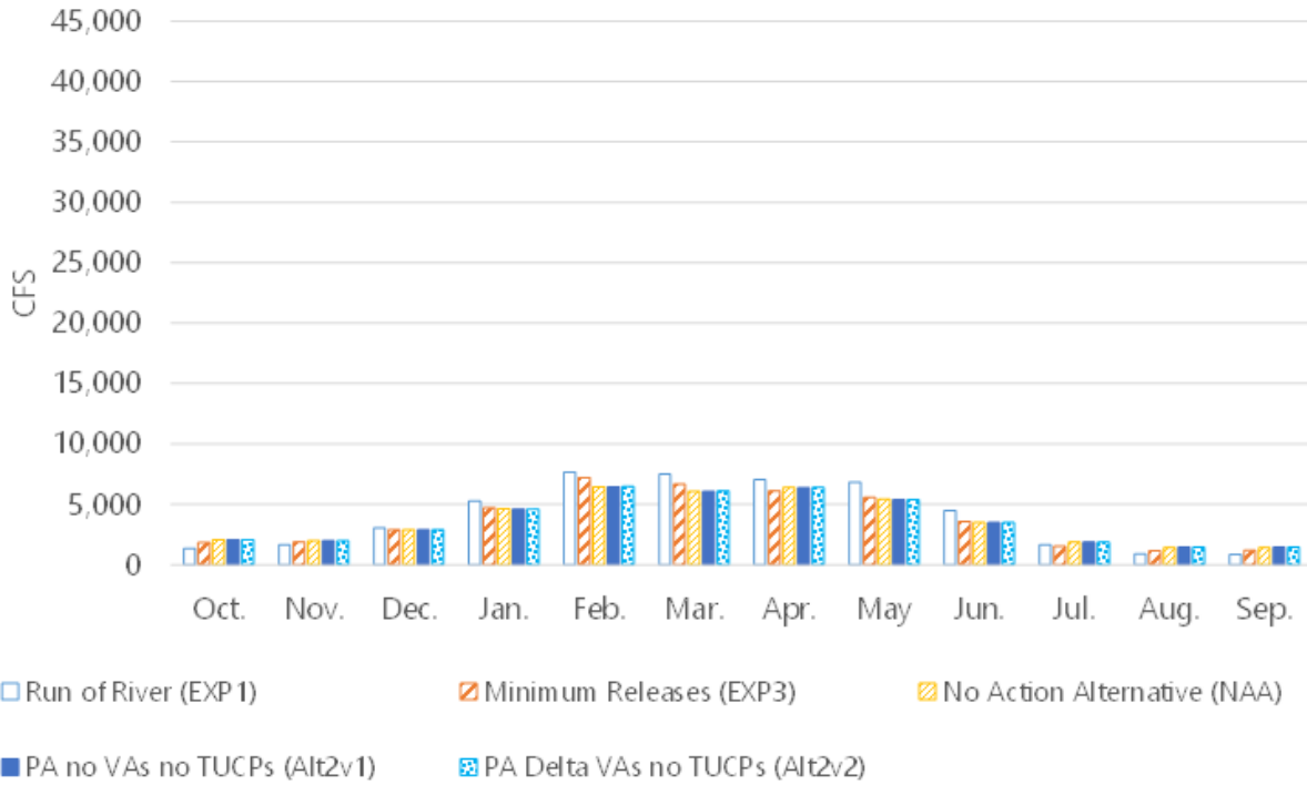
Figure B-78. San Joaquin River at Vernalis Monthly Flows, All Water Year Types
