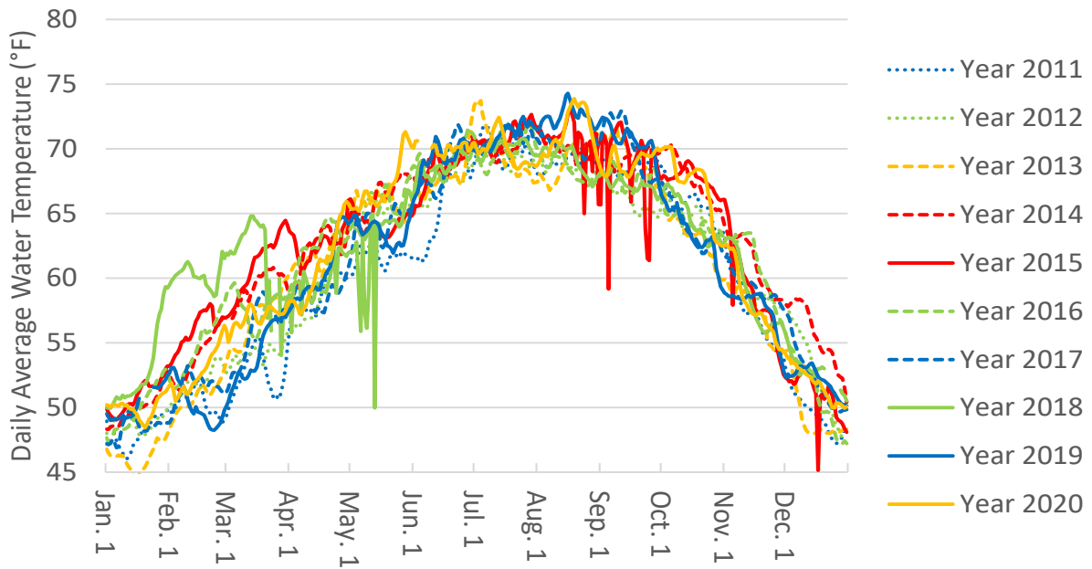
Figure B-85. Historical Water Temperatures at Port Chicago (PCT)
