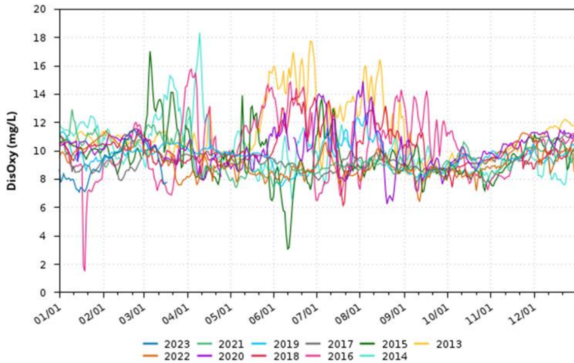
Figure B-69. San Joaquin River at Mossdale Bridge Daily Average Dissolved Oxygen (mg/L) for WY 2013–2023
