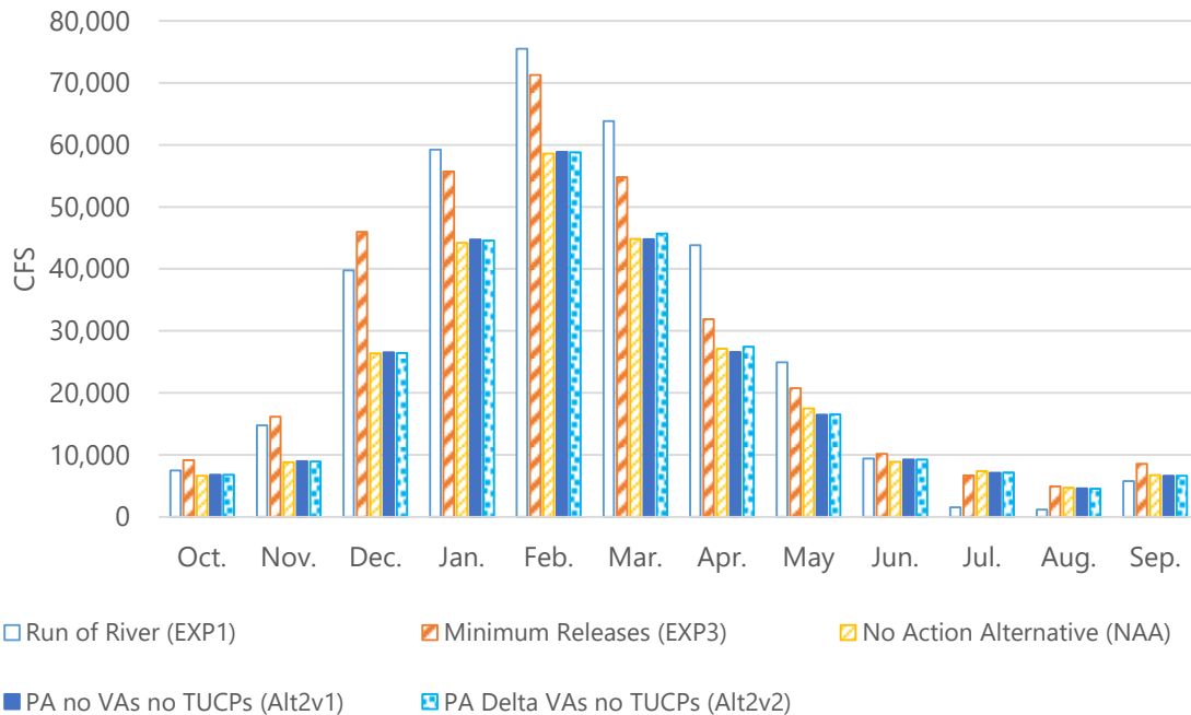
Figure B-81. Delta Monthly Outflow, All Water Year Types
