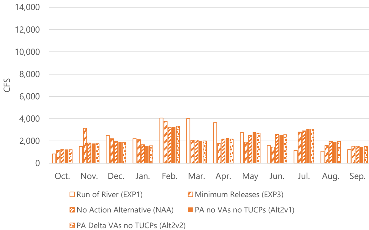
Figure B-45. American River below Nimbus Dam Monthly Flows, Critical Water Year Type
