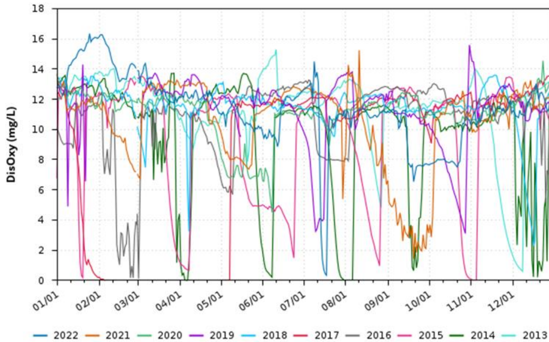
Figure B-24. Sacramento River at Bend Bridge Daily Average Dissolved Oxygen (mg/L) for WY 2013–2022
