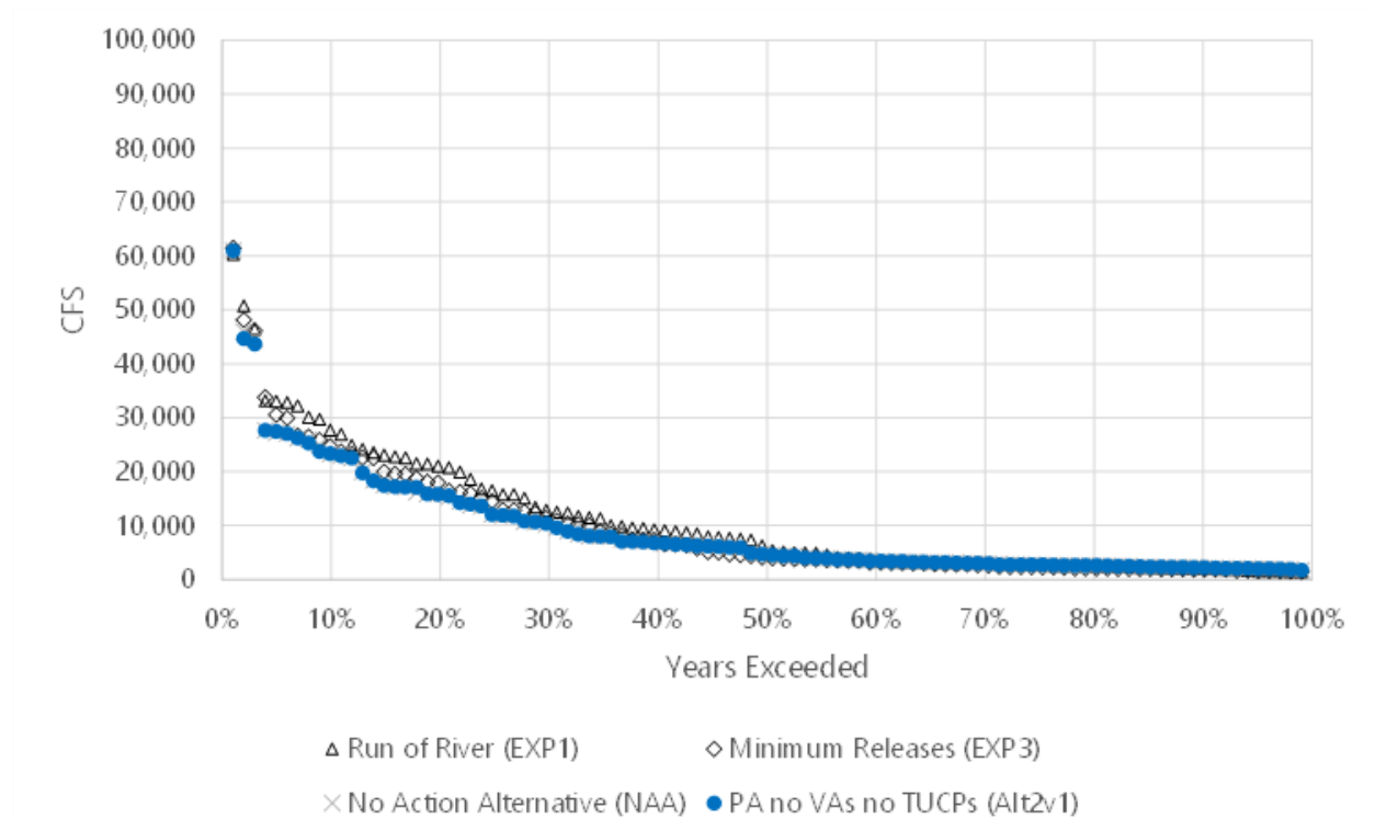
Figure B-83. San Joaquin River at Vernalis Annual Peak Flow Frequency
