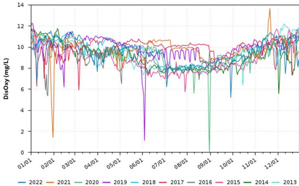
Figure B-59. Stanislaus River at Ripon Daily Average Dissolved Oxygen (mg/L) for WY 2013–2022
