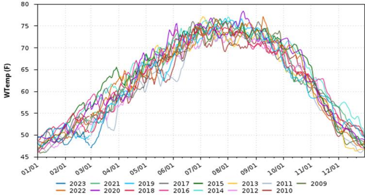
Figure B-88. Old River at Franks Tract Daily Average Water Temperature (°F) for WY 2009–2023
