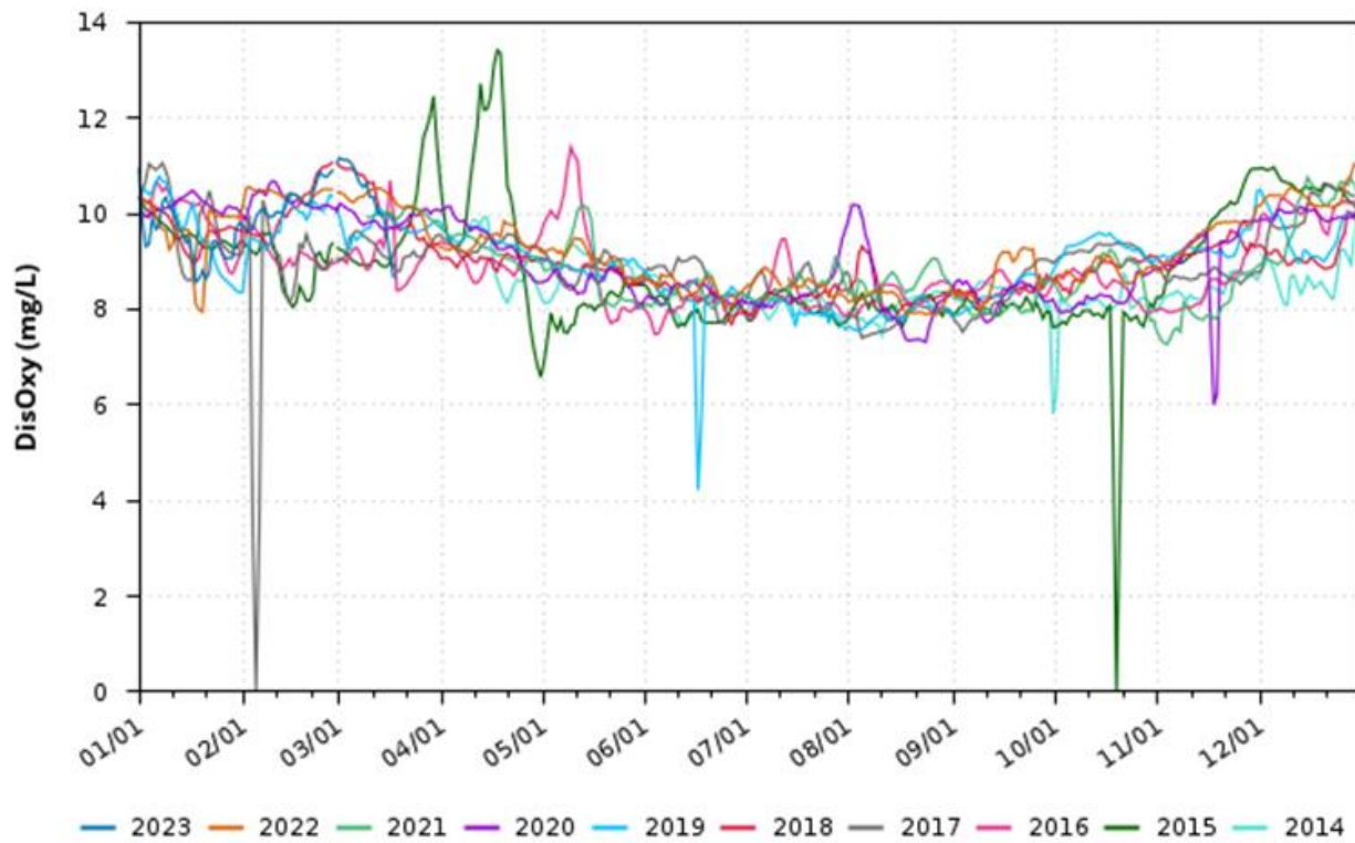
Figure B-89. Old River at Franks Track Daily Average Dissolved Oxygen (mg/L) for WY 2014–2023
