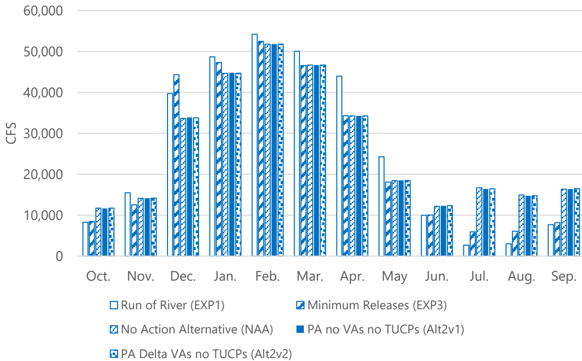
Figure B-15. Sacramento River at Verona Monthly Flows, Wet Water Year Type
