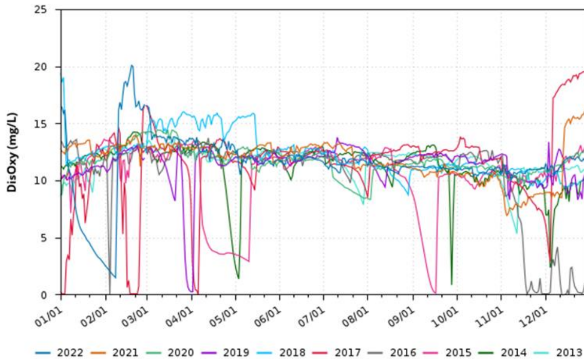
Figure B-37. Sacramento River above Clear Creek Daily Average Dissolved Oxygen (mg/L) for WY 2013–2022
