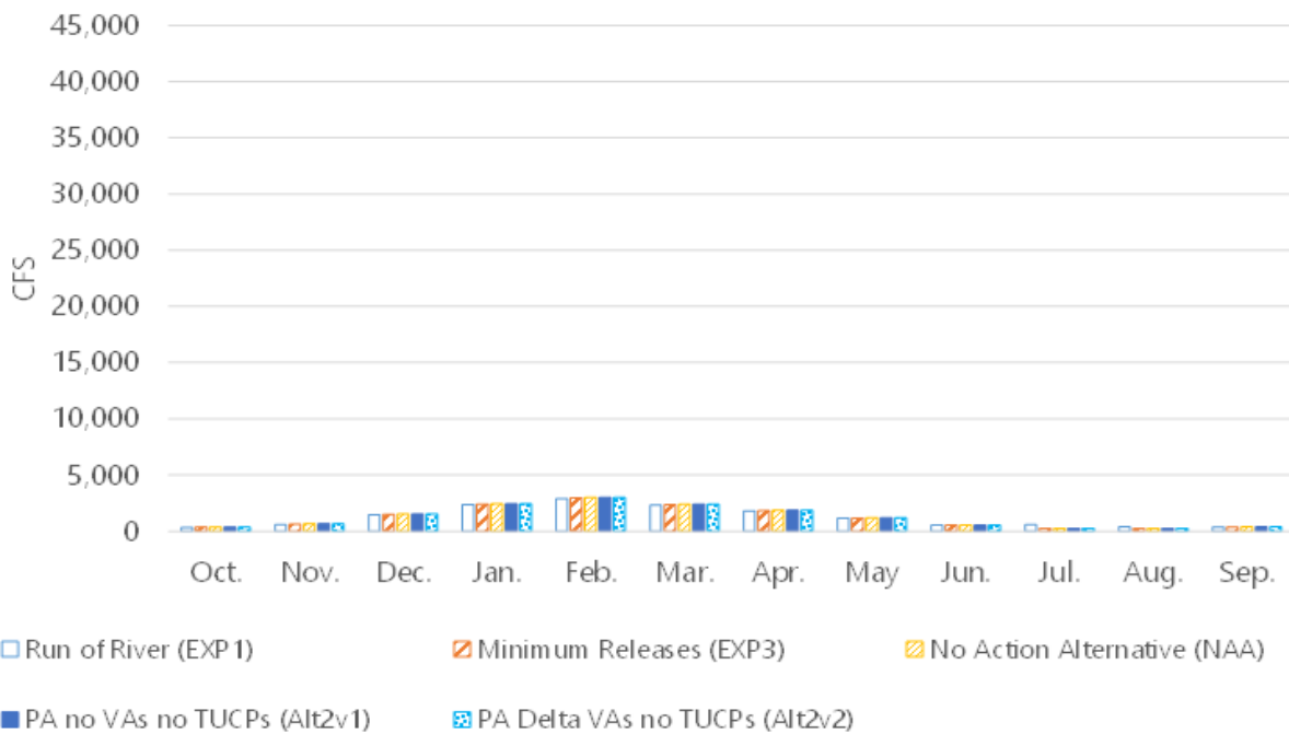
Figure B-79. Mokelumne River Monthly Flows, All Water Year Types
