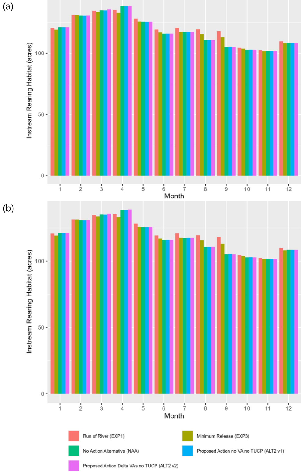
Figure B-70. Estimated Instream Rearing Habitat for Juvenile Spring-run Chinook Salmon (a) and Steelhead (b) in the San Joaquin River
