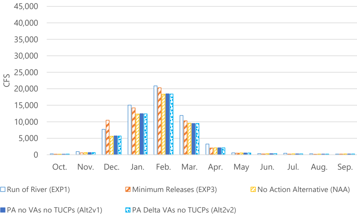
Figure B-77. Flow through Yolo Bypass Monthly Flows, All Water Year Types
