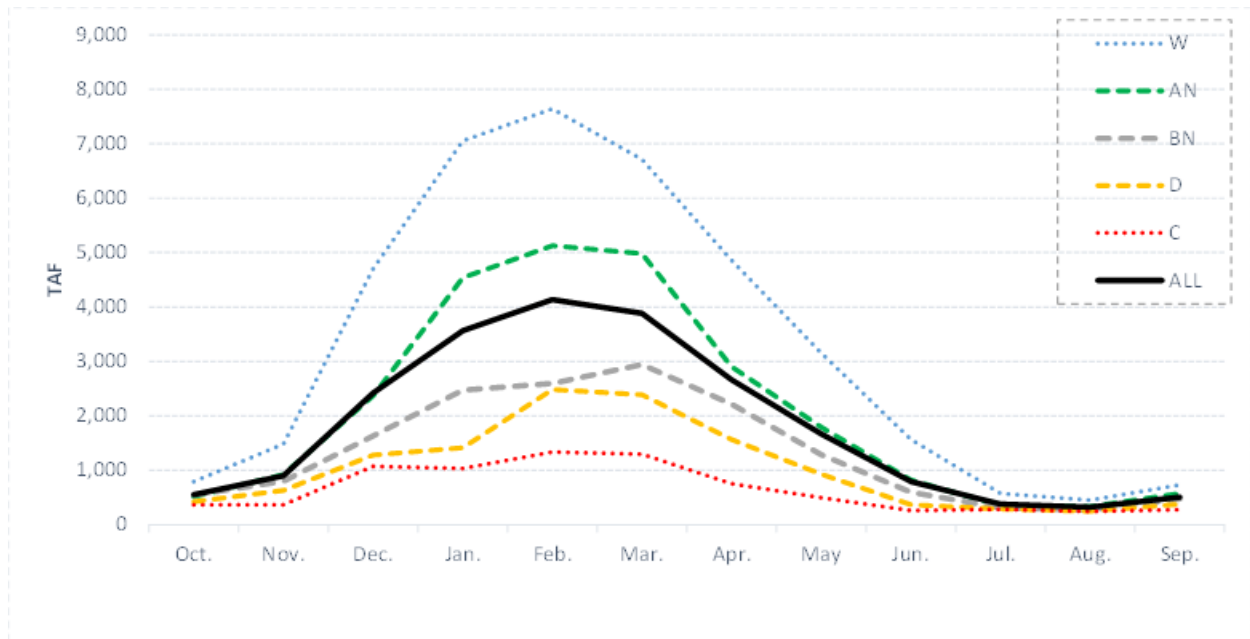
Figure B-72. Inflows to the Central Valley by Month and Water Year Type (EXP1)
