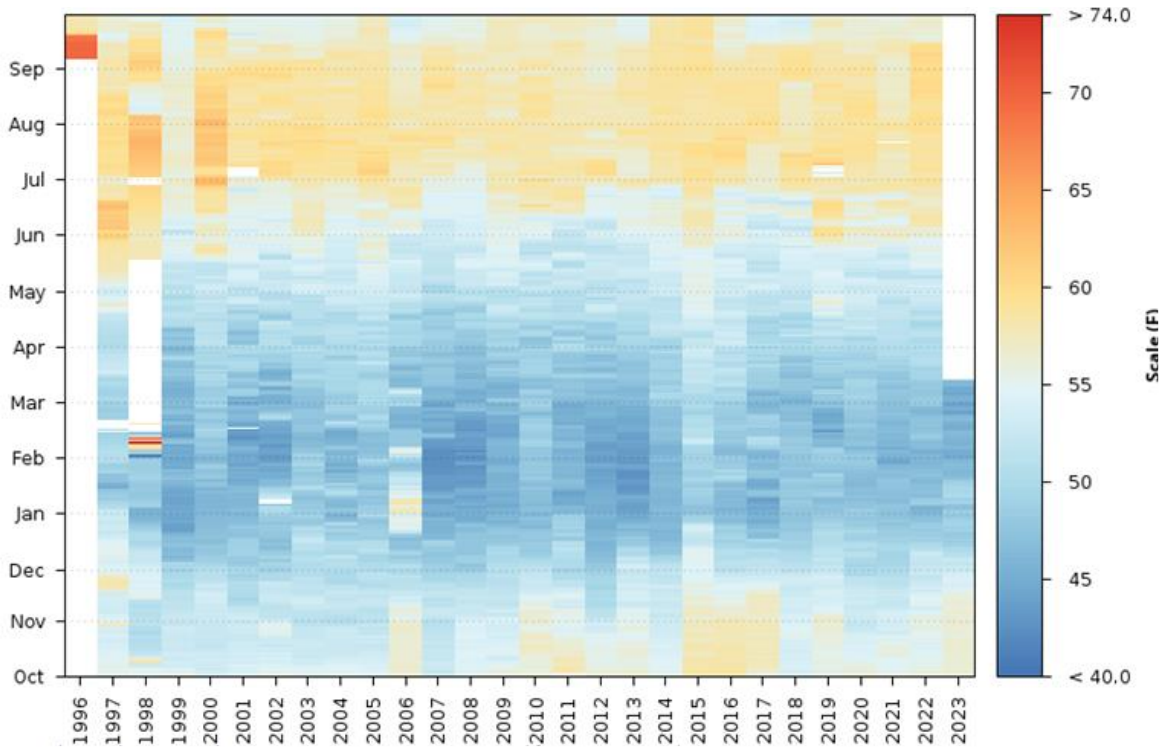
Figure B-36. Clear Creek near Igo Daily Average Water Temperature (°F) for WY 1996–2023
