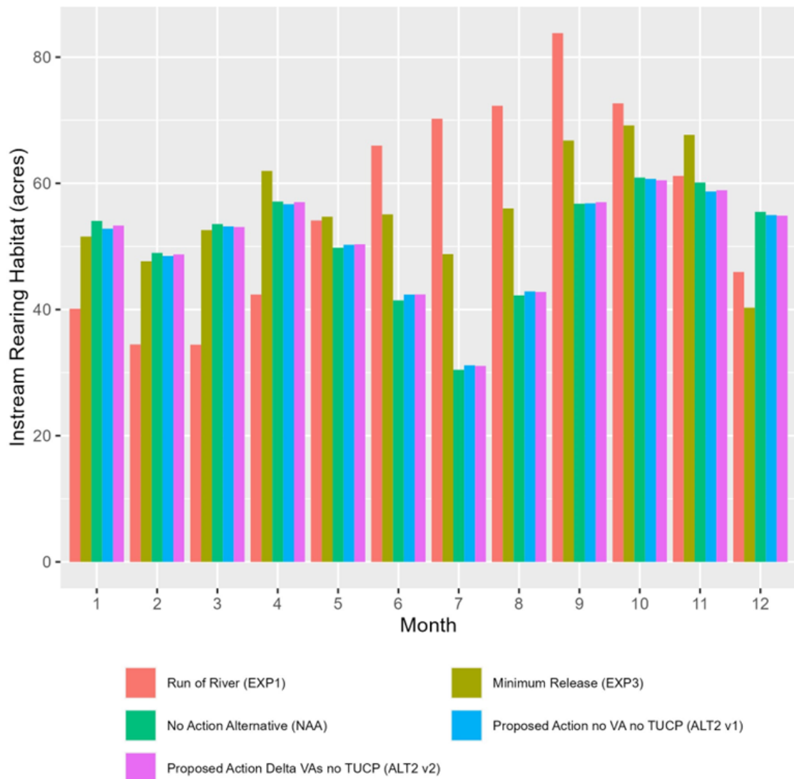
Figure B-26. Estimated Instream Rearing Habitat for Juvenile Winter-run Chinook Salmon, Spring-run Chinook Salmon, and Steelhead in the Upper Sacramento River
