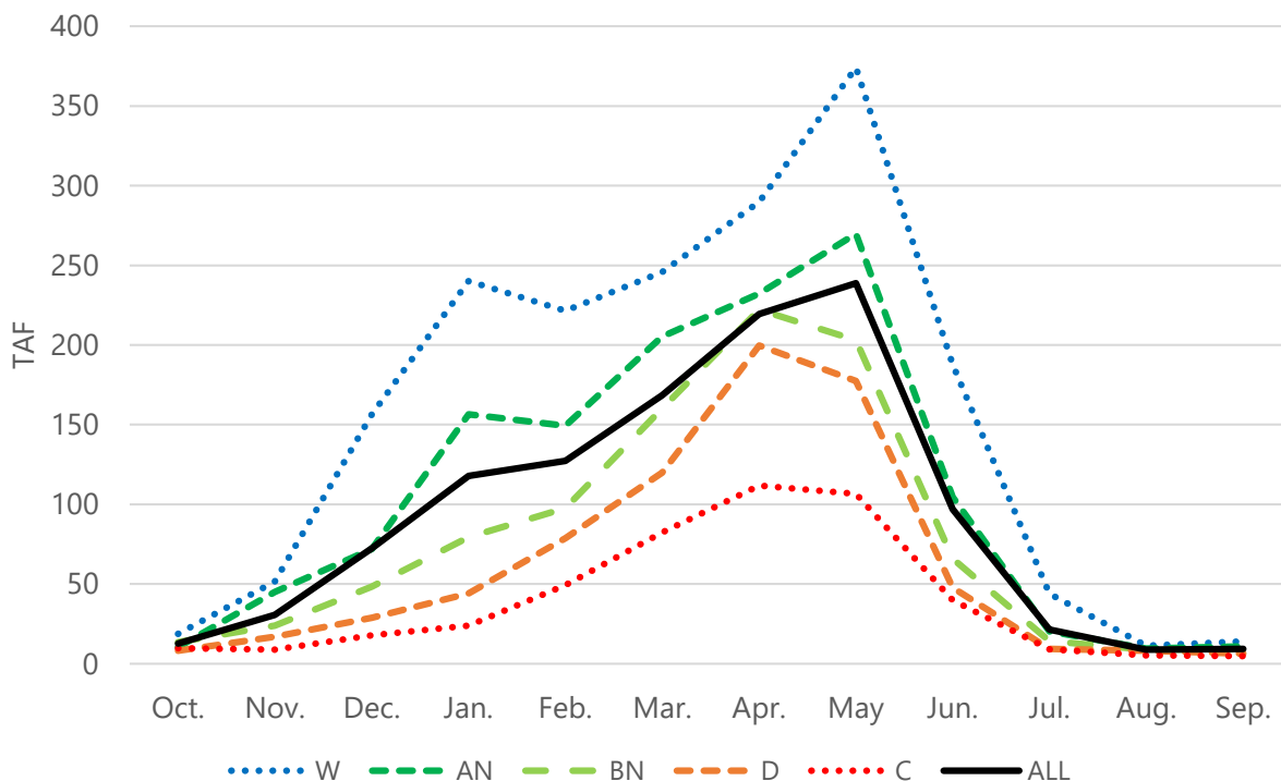
Figure B-51. Inflow to New Melones Reservoir by Month and Water Year Types (40-30-30)
