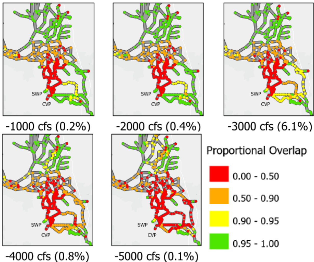
Figure B-90. No Action March Proportional Overlap with and without Exports
