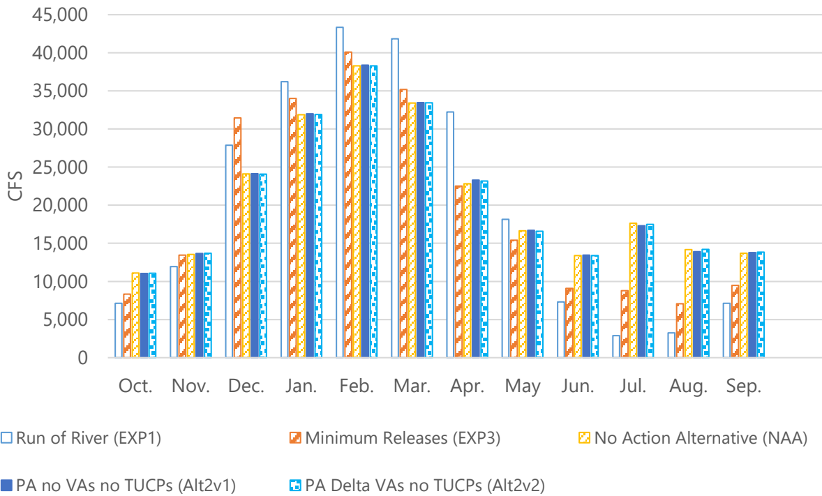
Figure B-76. Sacramento River at Freeport Monthly Flows, All Water Year Types
