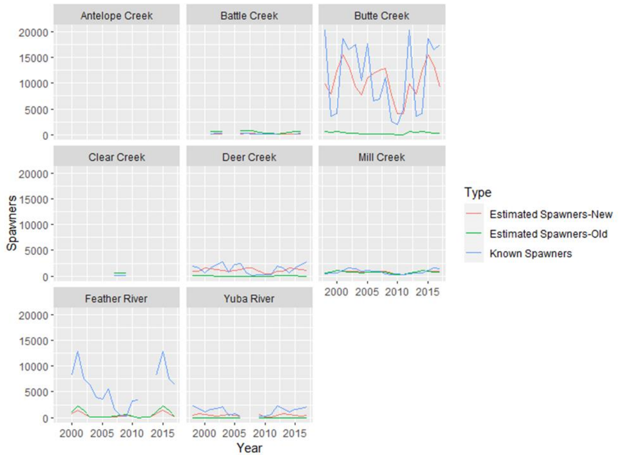
Figure F.3-6. Plot of estimated spawners, both with original and newly calibrated parameter estimates, and known spawner abundances for the best final calibration effort for spring-run Chinook salmon, presented for all watersheds that provided data to model calibration.
