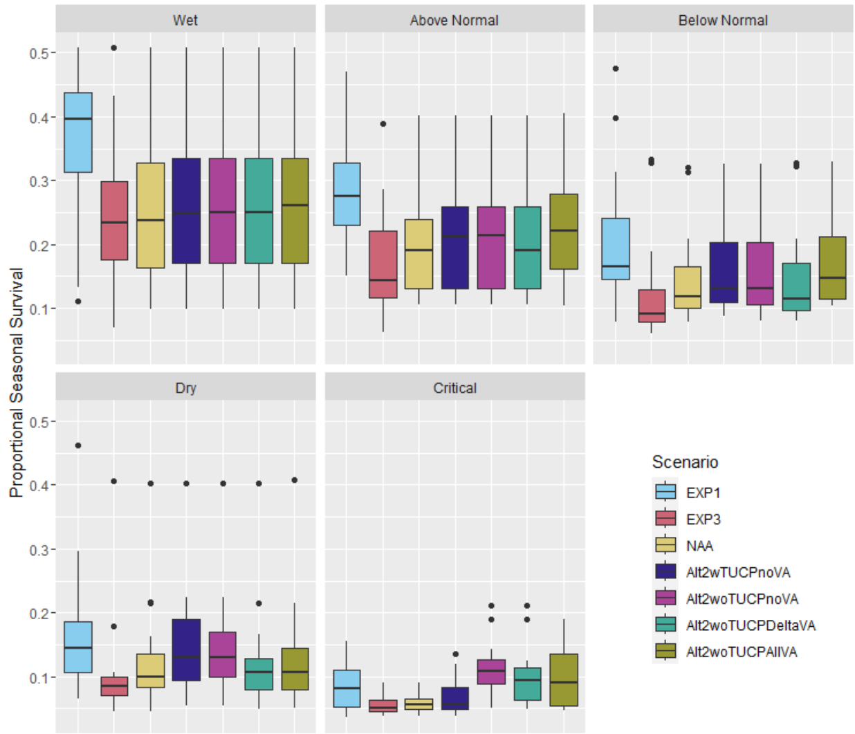
Figure J.5-4. Boxplots of mean annual seasonal (March 15 through June 15) survival for different modeled scenarios by water year type (BA scenarios).
