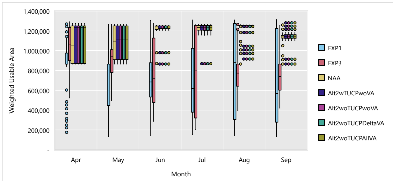
Figure N.2-11. Expected Total WUA for Steelhead Fry Rearing in the Stanislaus River Downstream of Goodwin Dam for EXP1, EXP3, the NAA, and Four Phases of Alternative 2 by Month
