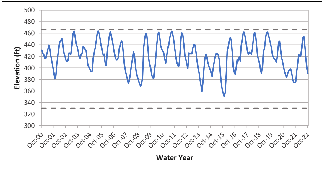
Figure C-17. Folsom Lake Elevation
