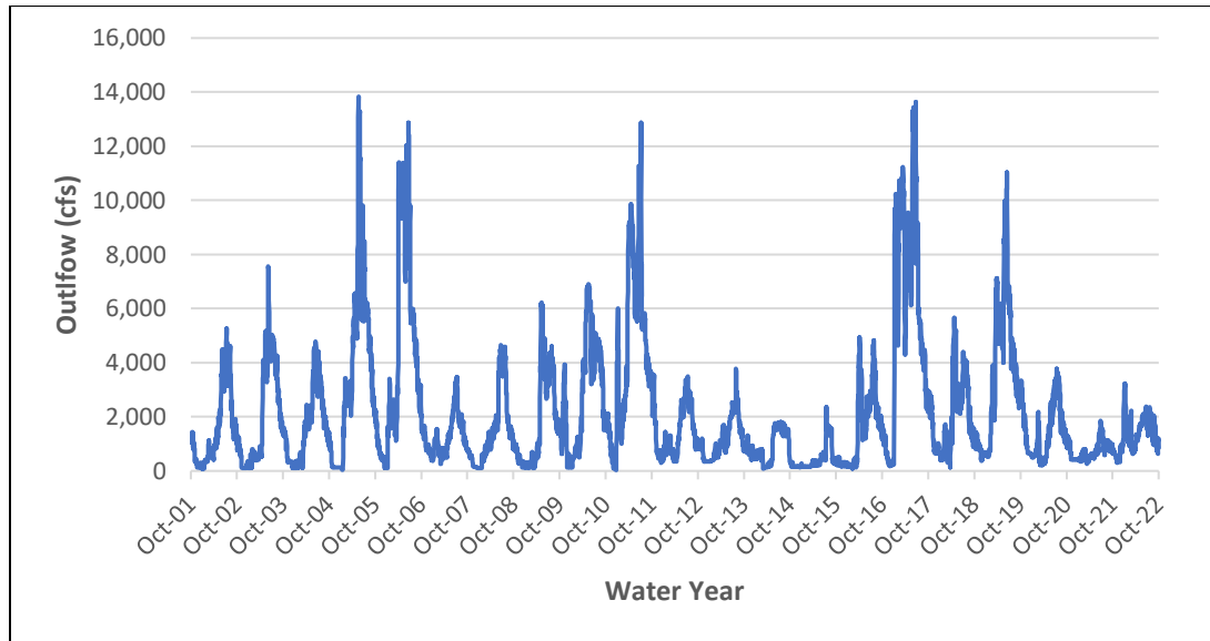
Figure C-22. Millerton Lake Outflow
