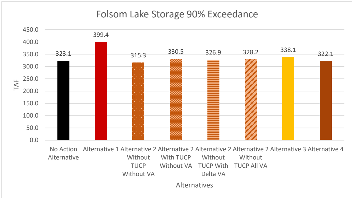
Figure W.1-10. Folsom Lake Storage 90% Exceedance
