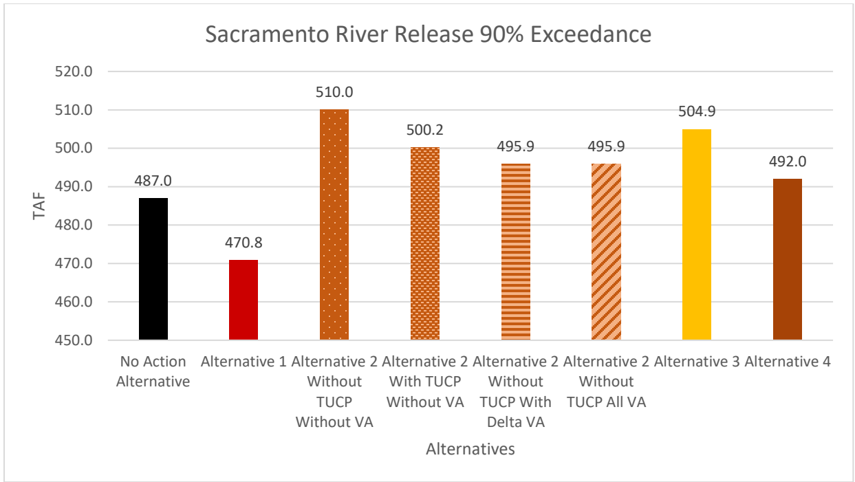
Figure W.1-8. Sacramento River Release 90% Exceedance
