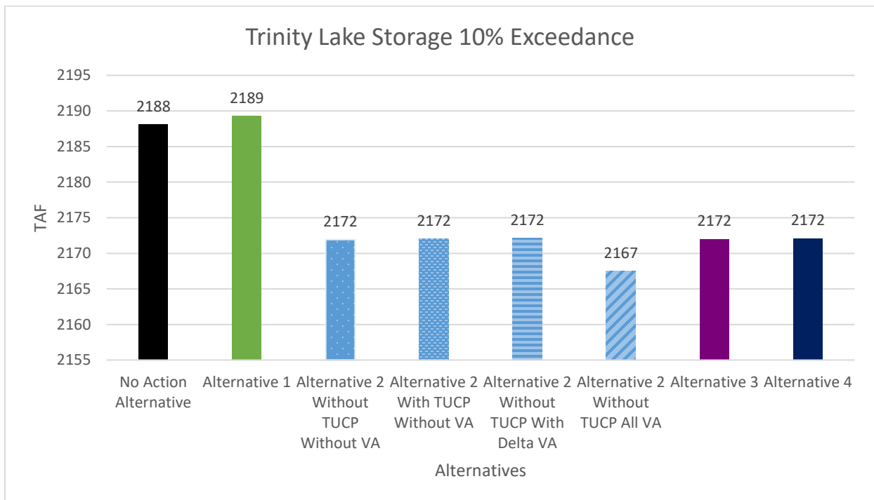
Figure W.1-1. Trinity Lake Storage 10% Exceedance
