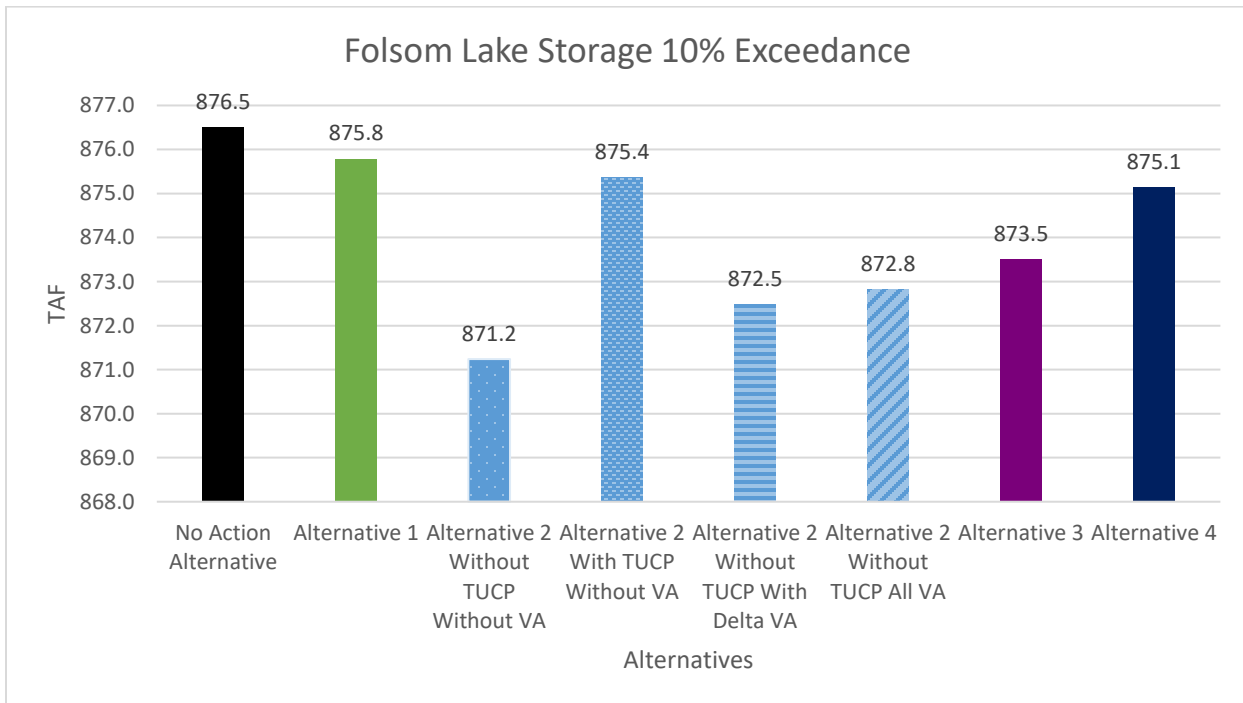
Figure W.1-9. Folsom Lake Storage 10% Exceedance
