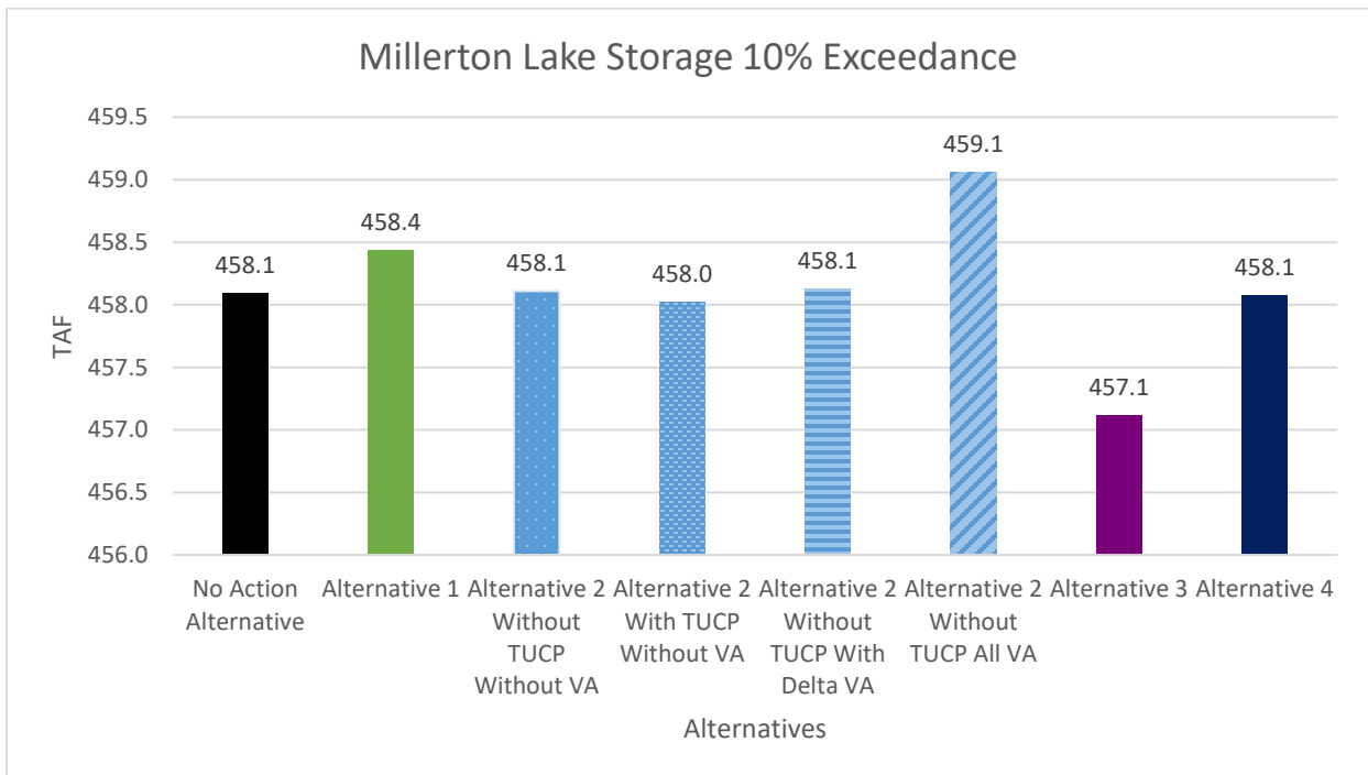
Figure W.1-17. Millerton Lake Storage 10% Exceedance
