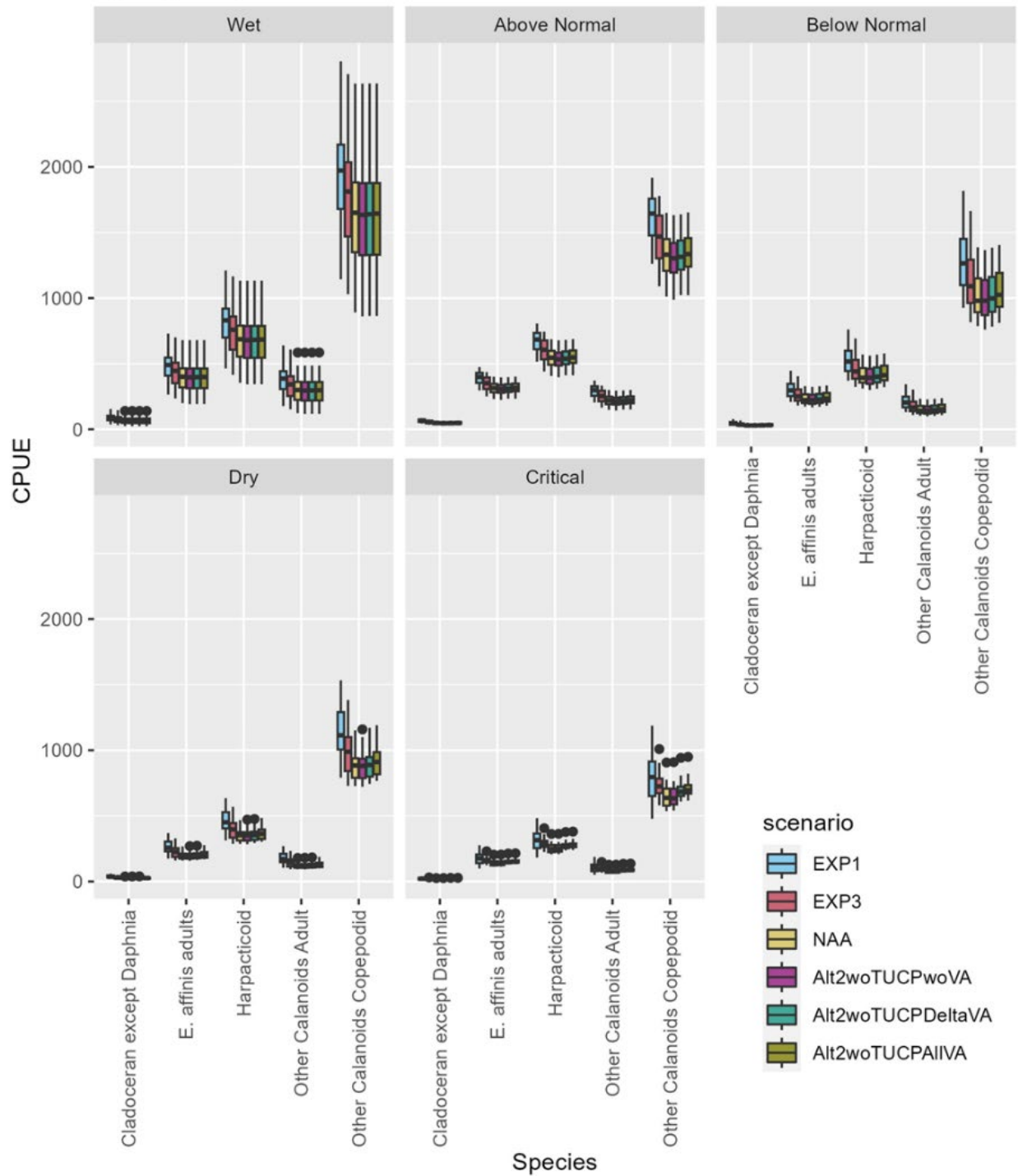
Figure 10-12. Boxplots of Significant Zooplankton Species CPUE by Scenario across Different Water Year Types for Spring
