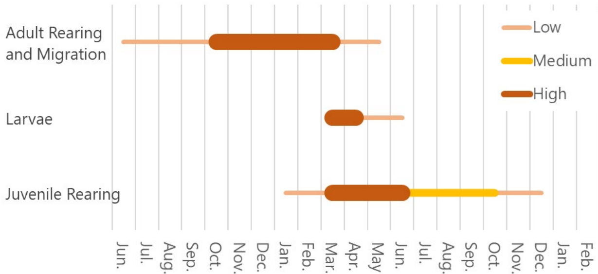
Figure 10-3. Temporal Life Stage Domains for Longfin Smelt
