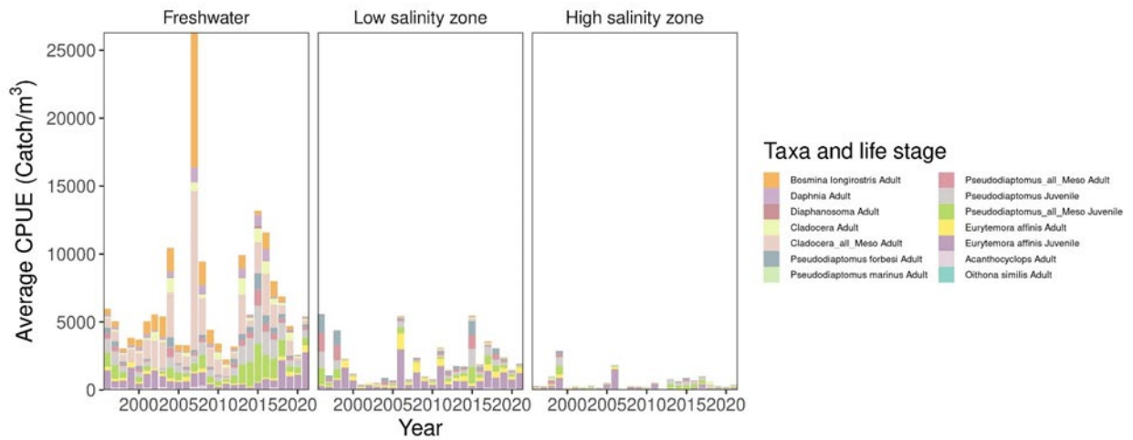
Figure 10-10. Average Mysid Density from Spring to Summer for Freshwater, Low Salinity Zone and High Salinity Zone
