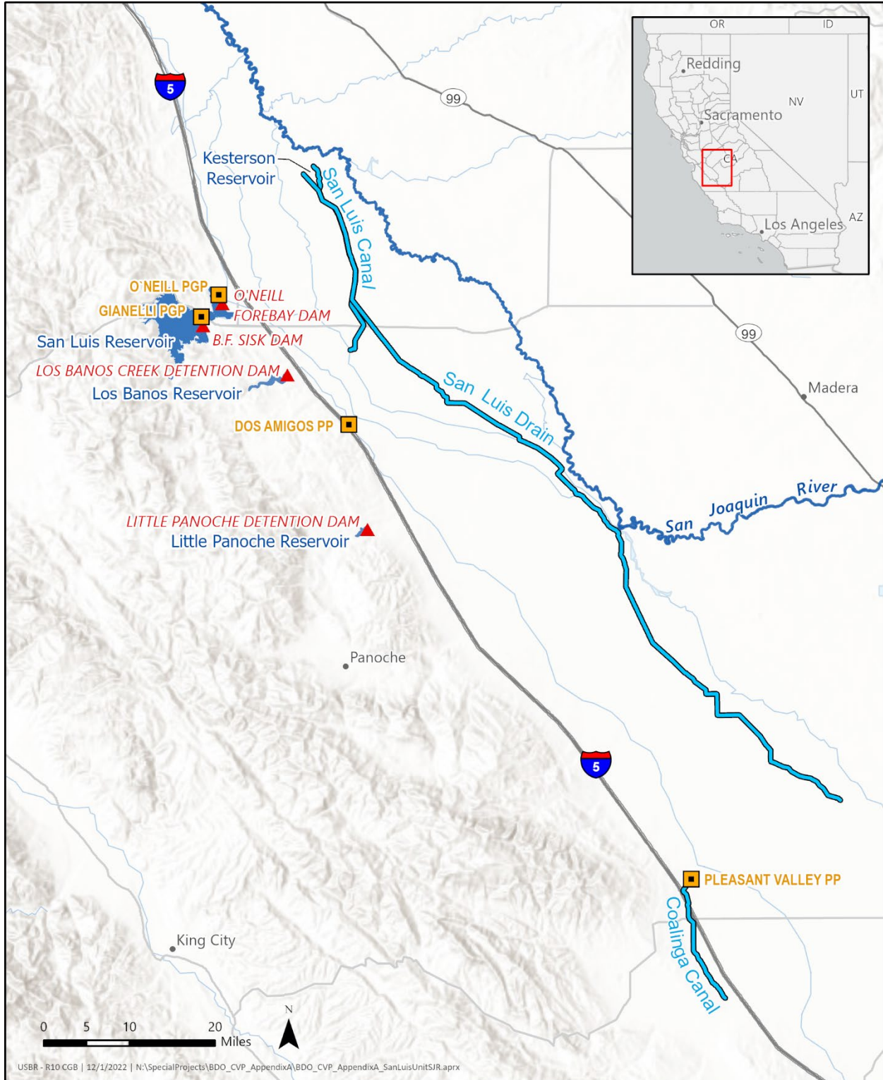
Figure A-21. Map of the CVP West San Joaquin Division
