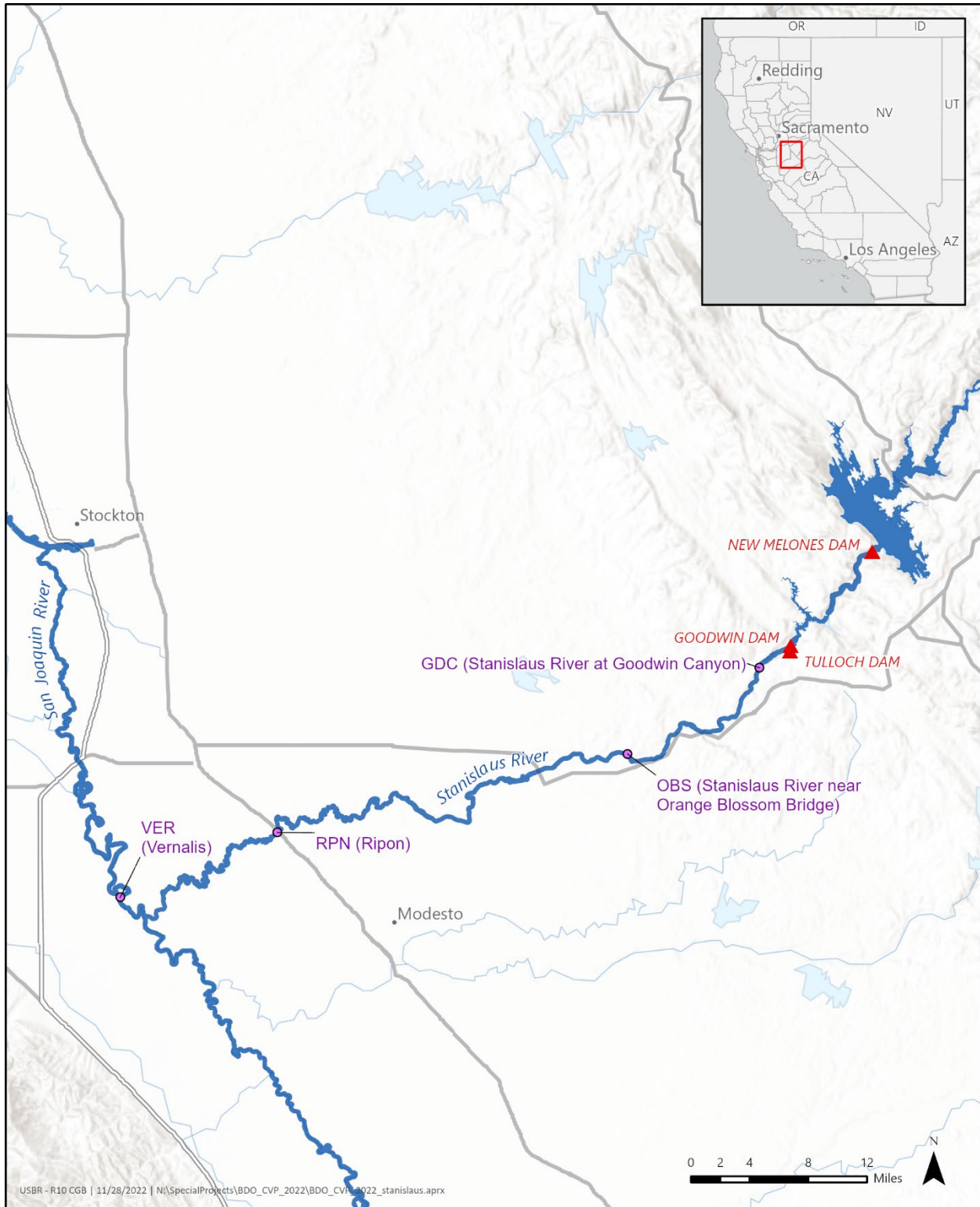
Figure A-22. Map of the CVP Eastside Division – New Melones Unit
