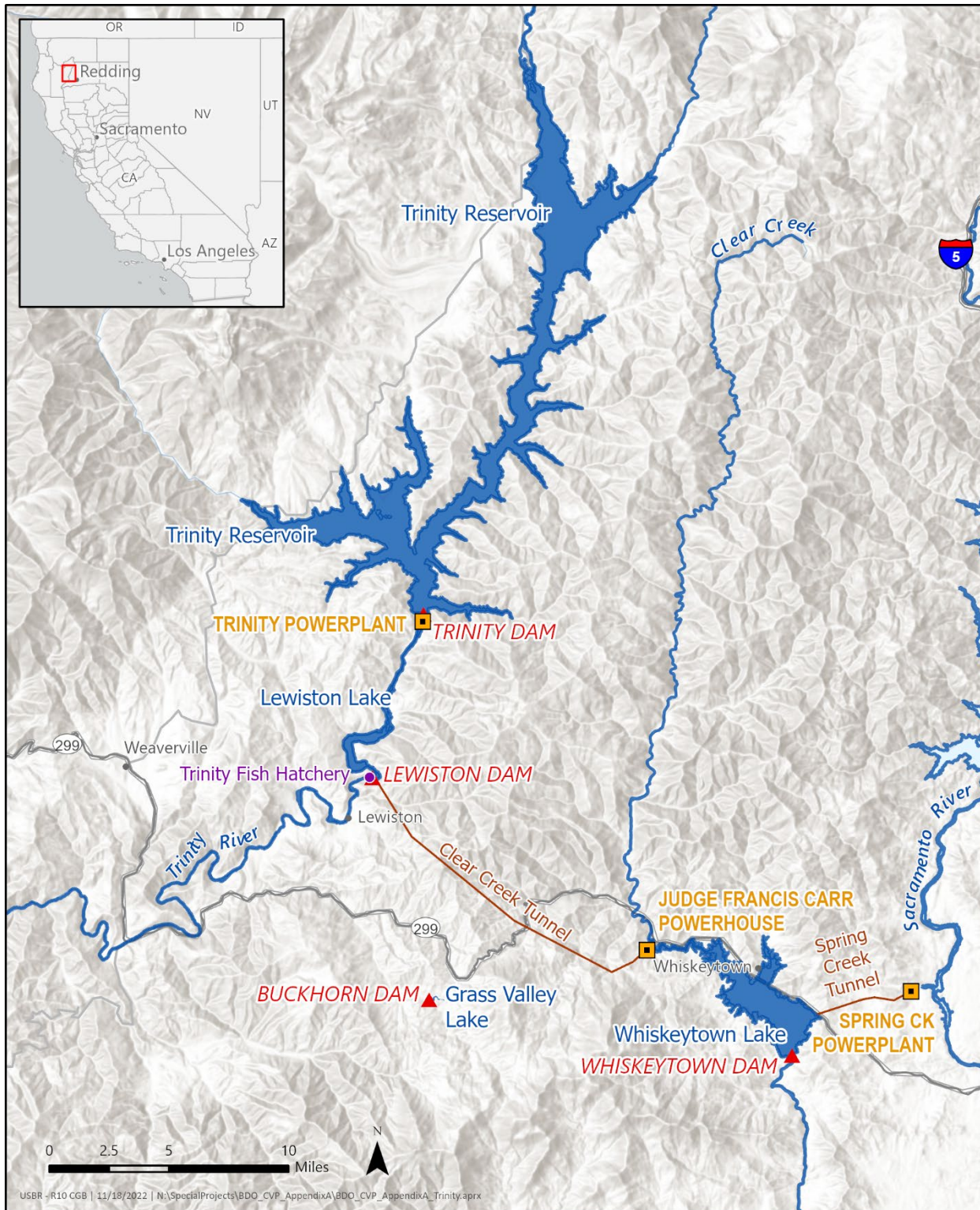
Figure A-35. Map of the CVP Trinity Division
