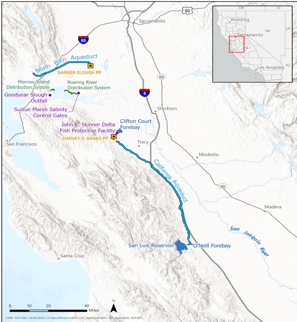
Figure A-44. Map of SWP Delta Facilities
