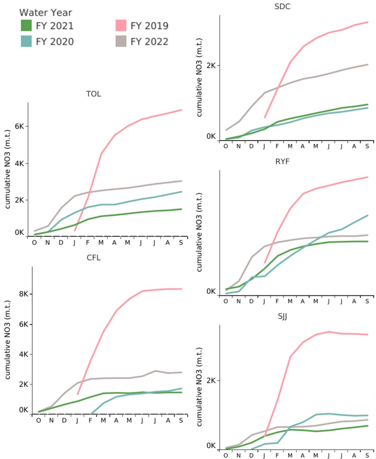
Figure J-24. Water year 2019 – 2022 cumulative nitrate (NO 3 ) flux (metric tons [m.t.]) by site
