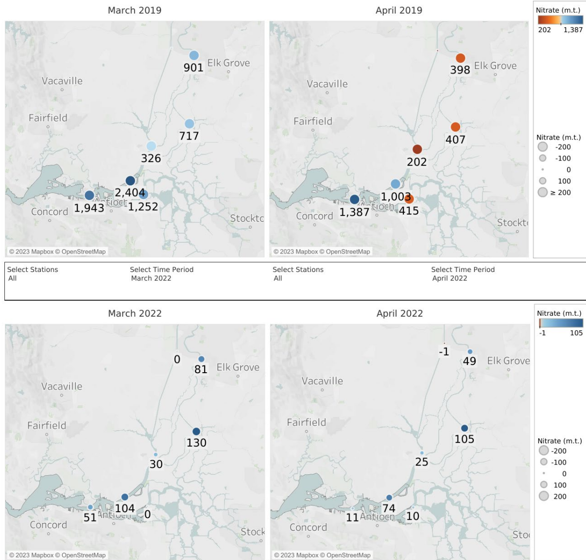
Figure J-25. Nitrate flux (megatonnes [m.t.]) in March 2019 (top left), March 2022 (bottom left), April 2019 (top right), and April 2022 (bottom right)
