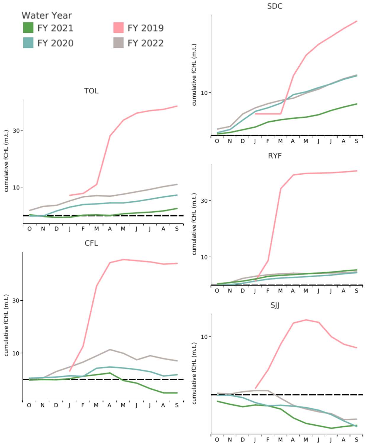
Figure J-26. Water year 2019 – 2022 cumulative chlorophyll (Chl a) flux (metric tons [m.t.]) by site
