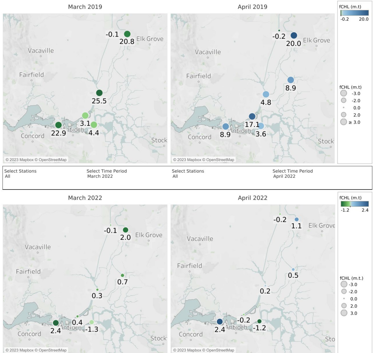
Figure J-27. Chlorophyll flux (fCHL, megatonnes [m.t.]) in March 2019 (top left), March 2022 (bottom left), April 2019 (top right), and April 2022 (bottom right)
