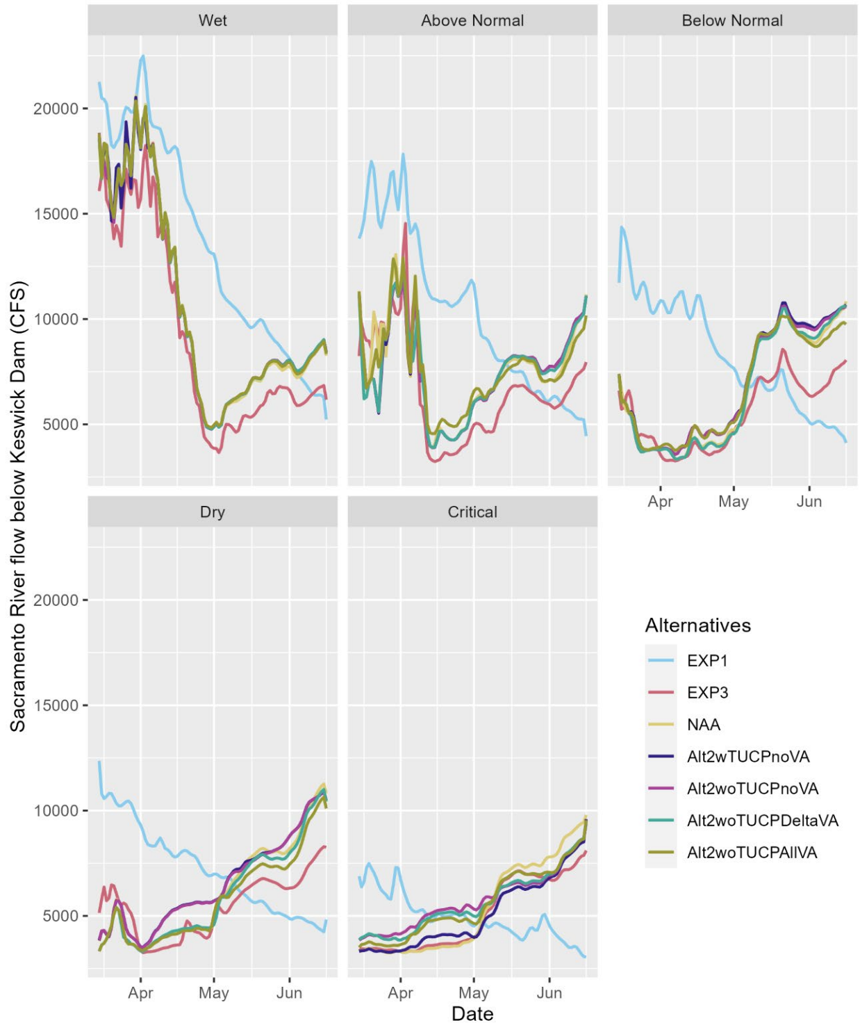
Figure J.4-6. Mean daily Sacramento River flow at Keswick (cfs) of different alternatives by date across water year types (USRDOM, 1922 – 2023).
