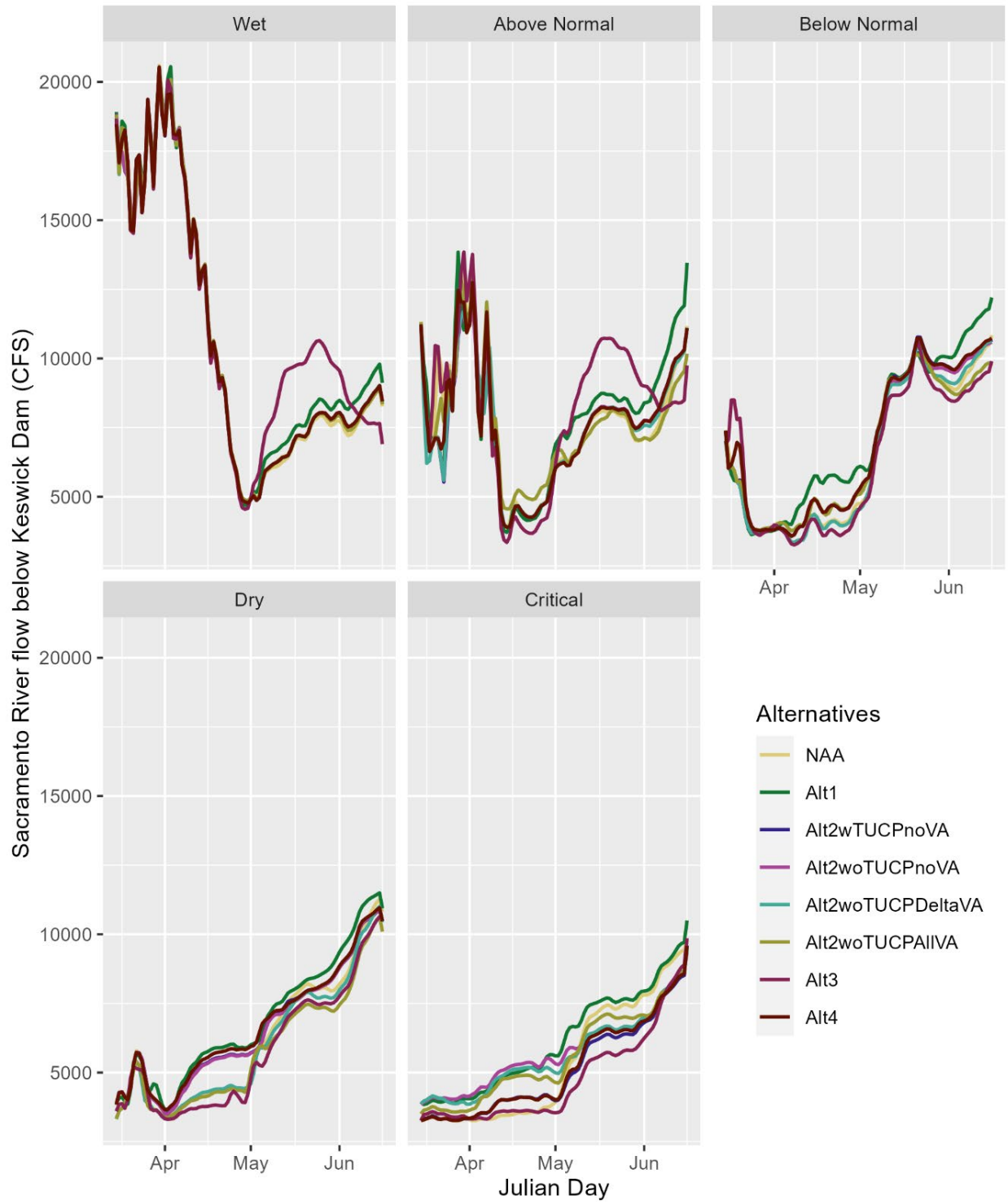
Figure J.4-7. Mean daily Sacramento River flow at Keswick (cfs) of different alternatives by date across water year types (USRDOM, 1922 – 2021).
