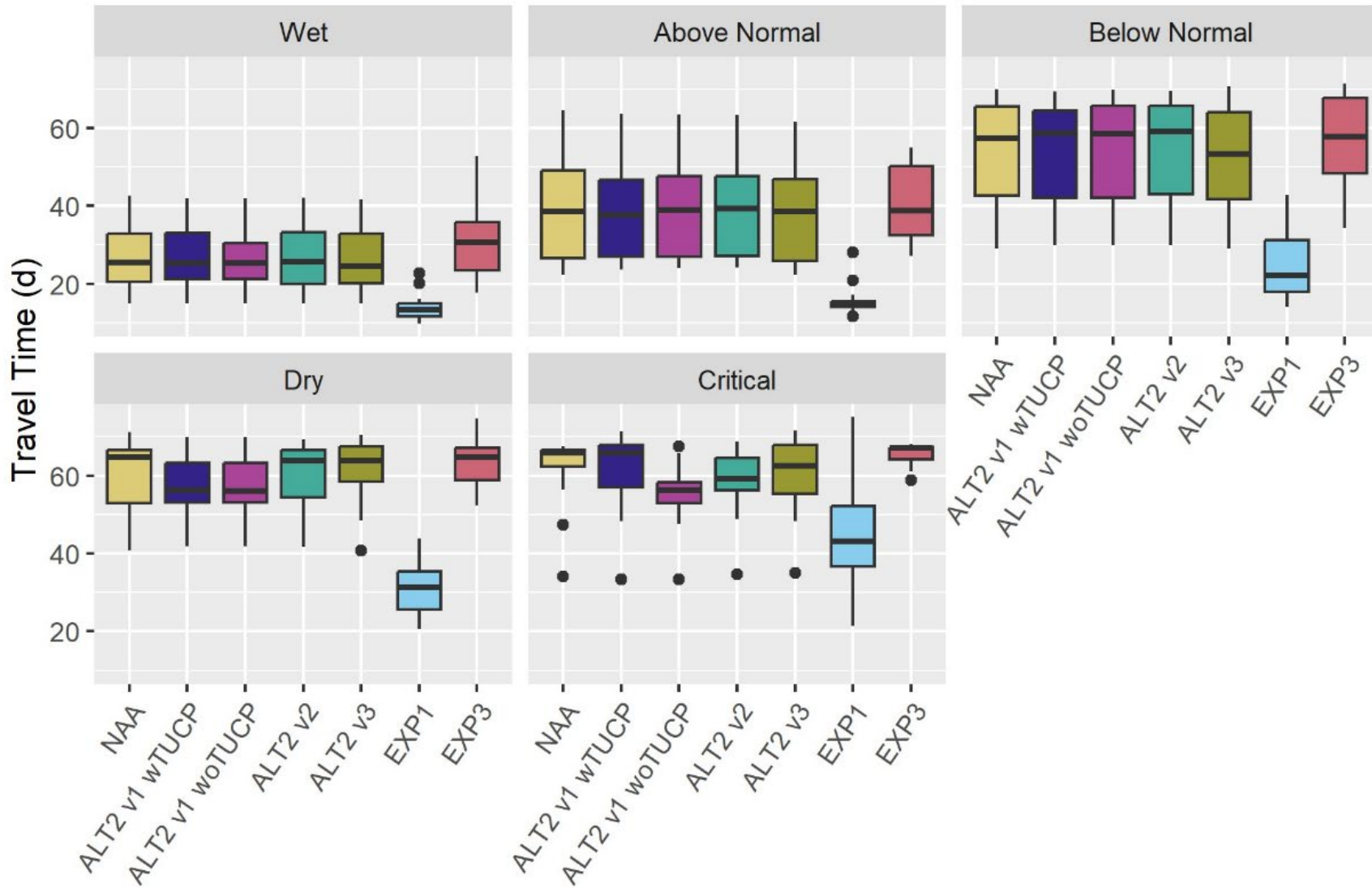
Figure J.4-10. Boxplots of mean travel time (days) between Red Bluff Diversion Dam and the Delta Cross Channel for different modeled scenarios by water year type.
