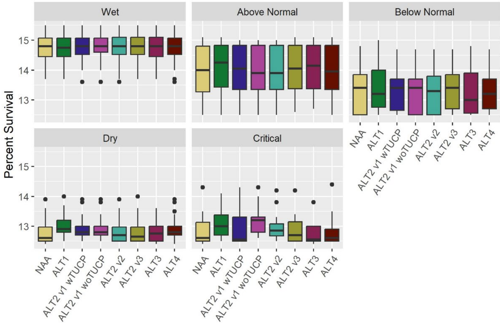
Figure J.4-3. Boxplots of mean survival between Red Bluff Diversion Dam and the confluence with the American River for different modeled scenarios by water year type.
