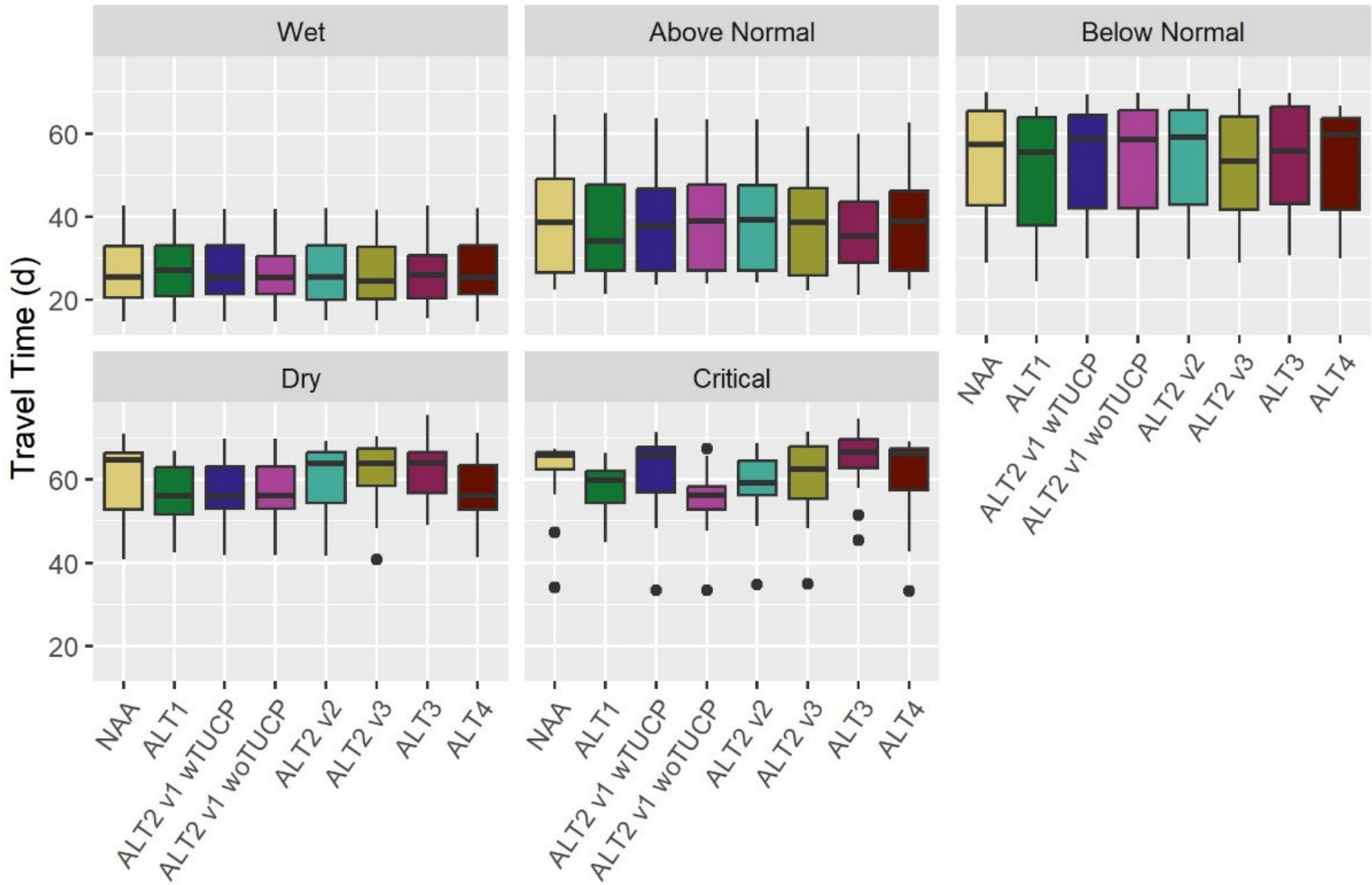
Figure J.4-11. Boxplots of mean travel time (days) between Red Bluff Diversion Dam and the Delta Cross Channel for different modeled scenarios by water year type.
