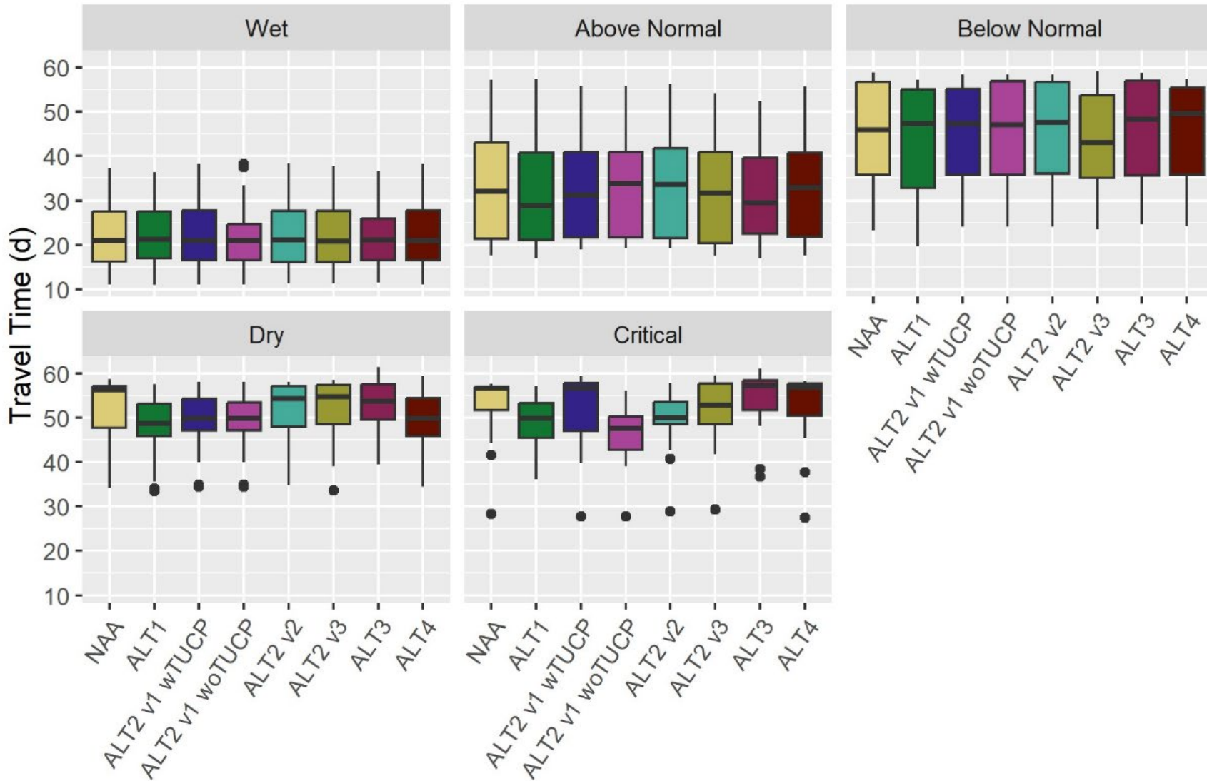
Figure J.4-9. Boxplots of mean travel time (days) between Red Bluff Diversion Dam and the confluence with the American River for different modeled scenarios by water year type.
