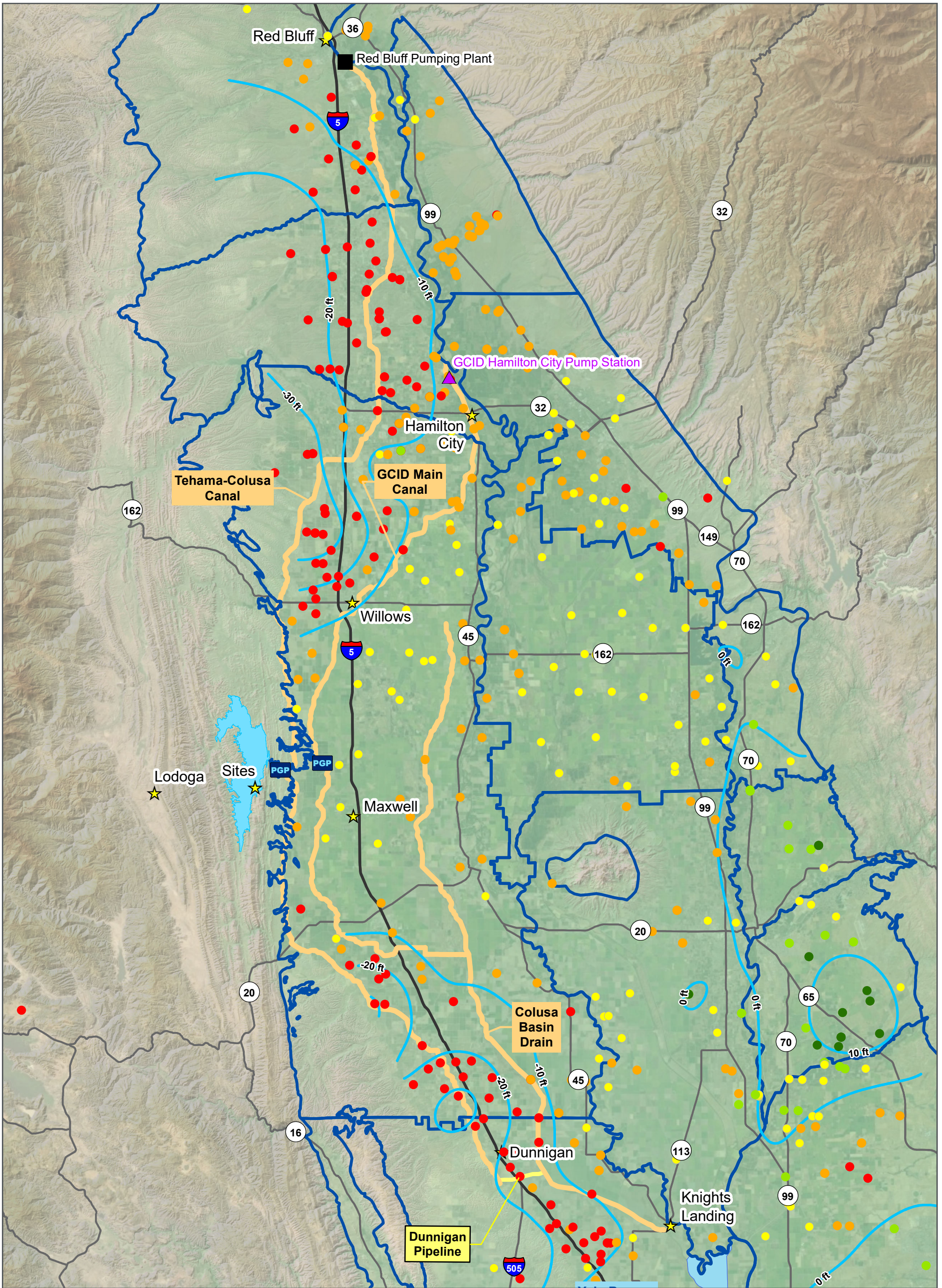
FIGURE 8A-2 CHANGE IN GROUNDWATER ELEVATION SPRING 2010 TO SPRING 2020
