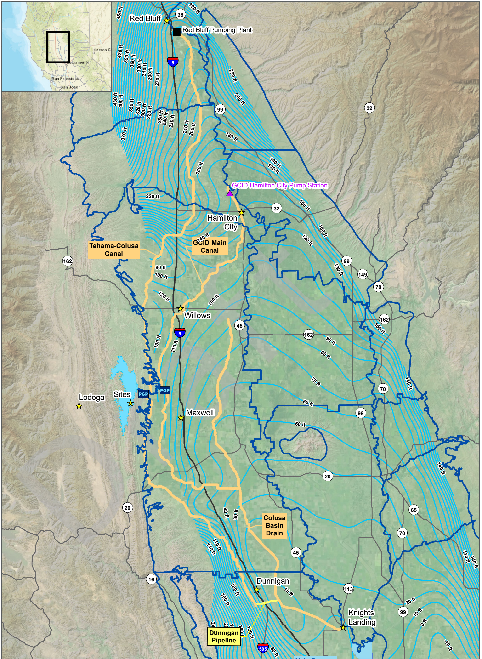
FIGURE 8A-1 GROUNDWATER ELEVATION CONTOURS SPRING 2020
