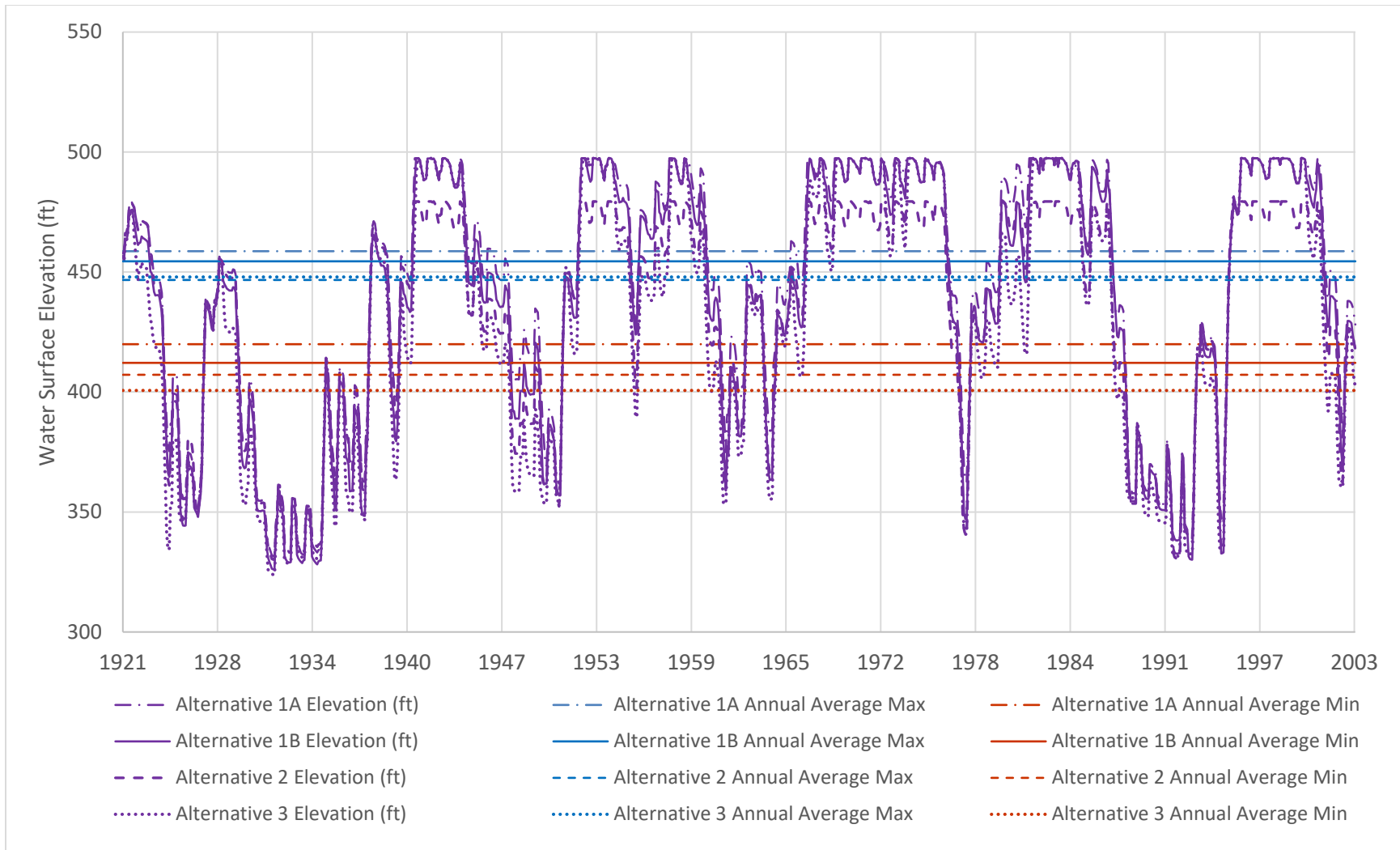
Figure 6F-1. CALSIM Modeled Sites Reservoir Surface Water Elevations and Long-Term Average Annual Maximum and Minimum Surface Water Elevations.
