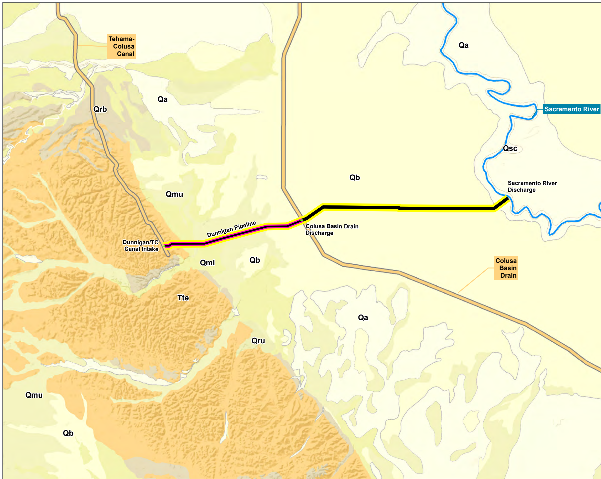
FIGURE 12-1C GEOLOGIC MAP OF THE STUDY AREA (SOUTHERN PORTION)
