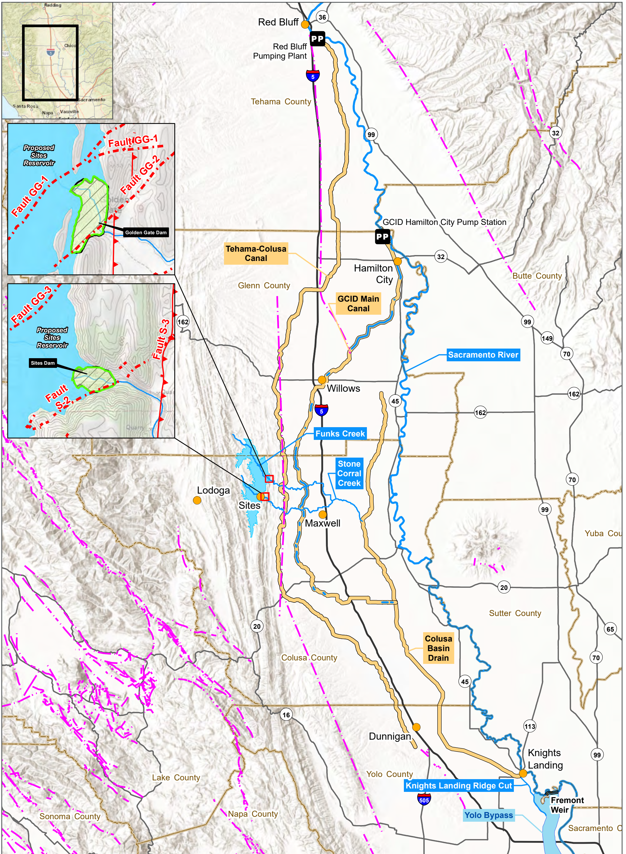
FIGURE 12-4 REGIONAL AND SITES RESERVOIR FAULTS MAP DATE: 6/22/2021
