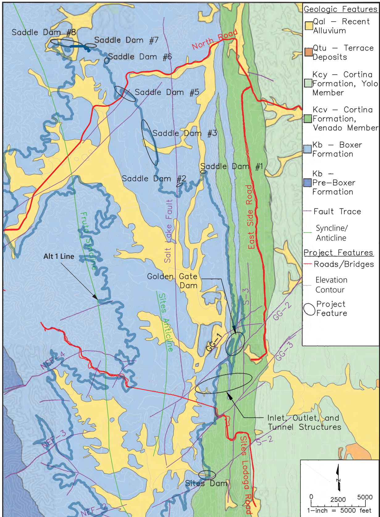
Figure 12-2 Detailed Geologic Map of Dam and Inundation Area
