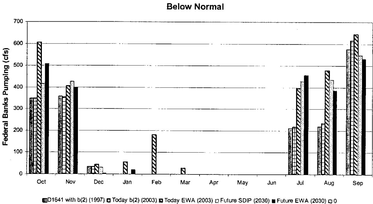
Figure 95 Average below normal year (40-30-30 Classification) monthly Federal Banks Pumping
