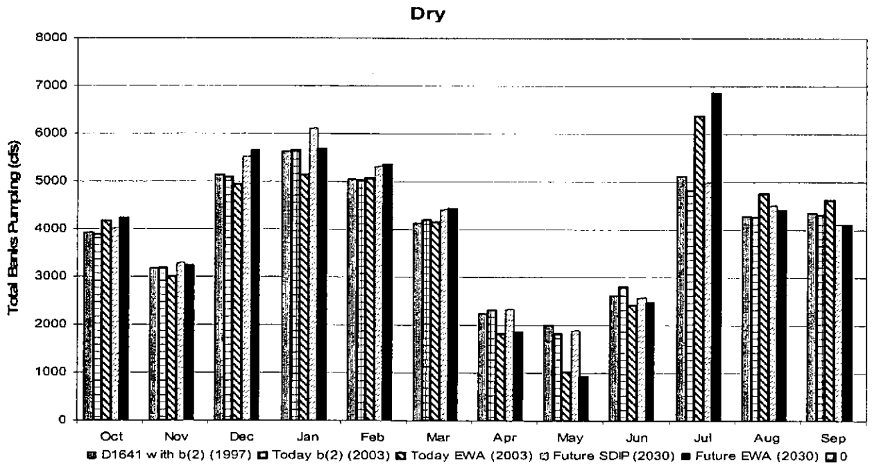
Figure 88 Average dry year (40-30-30 Classification) monthly Banks Pumping
