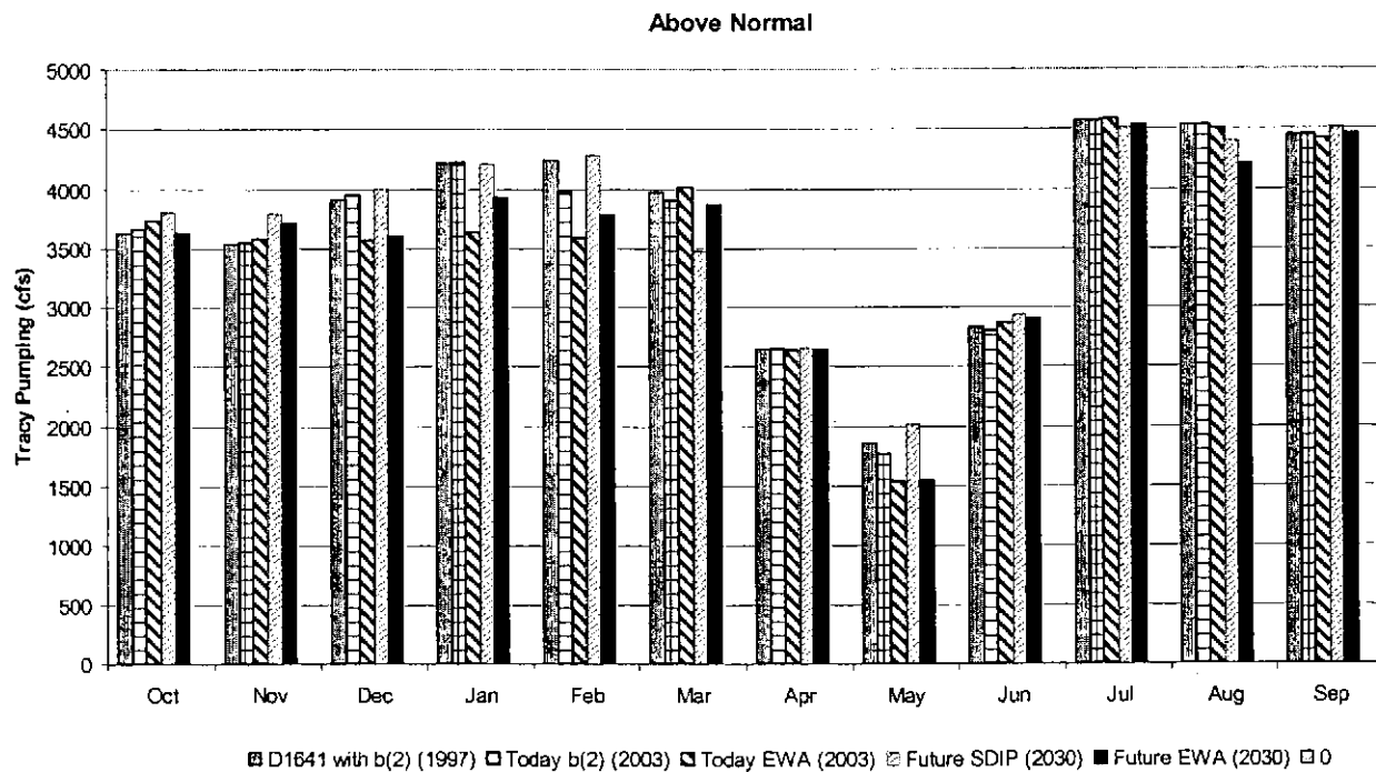
Figure 79 Average above normal year (40-30-30 Classification) monthly Tracy Pumping
