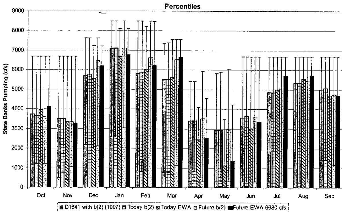
Figure 40 Banks Pumping 50 th Percentile Monthly Releases with the 5 th and 95 th as the bars
