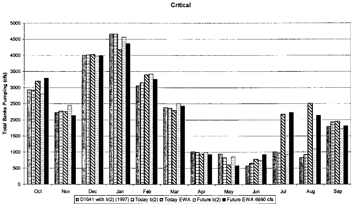
Figure 46 Average critical year (40-30-30 Classification) monthly Banks Pumping
