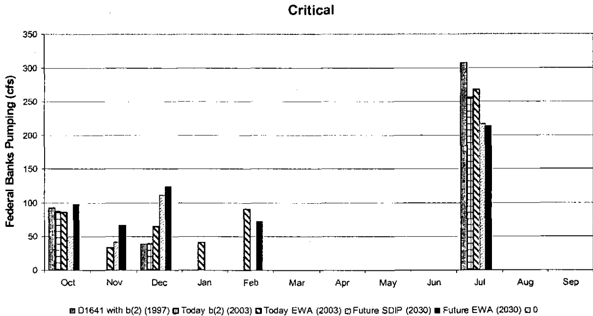
Figure 97 Average critical year (40-30-30 Classification) monthly Federal Banks Pumping
