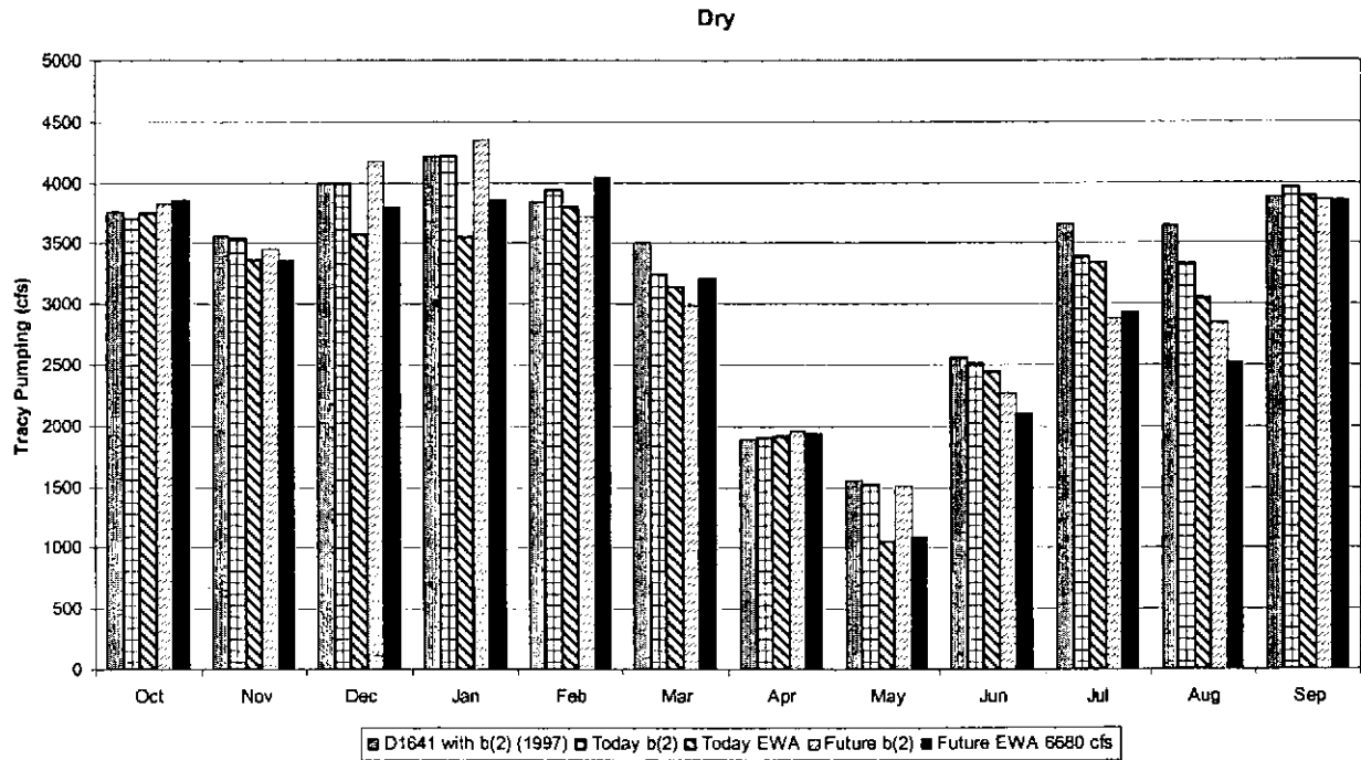
Figure 38 Average dry year (40-30-30 Classification) monthly Tracy Pumping
