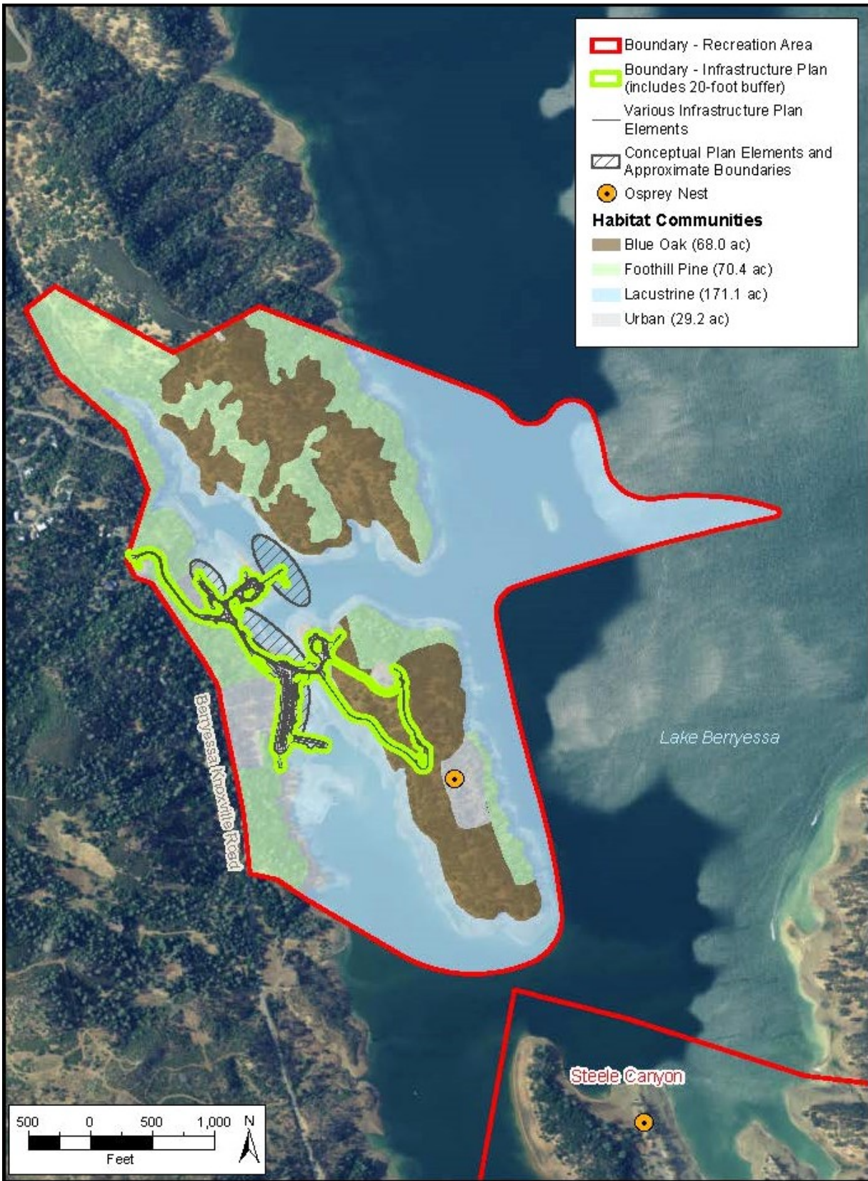
Figure F-6. Habitat Communities at Spanish Flat
