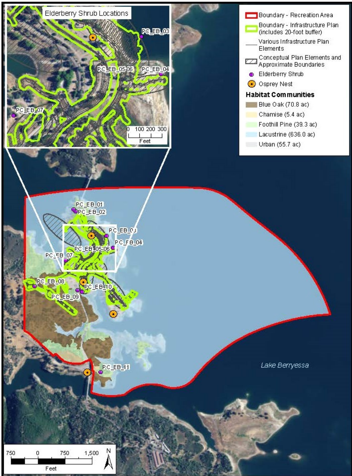
Figure F-3. Habitat Communities at Putah Canyon
