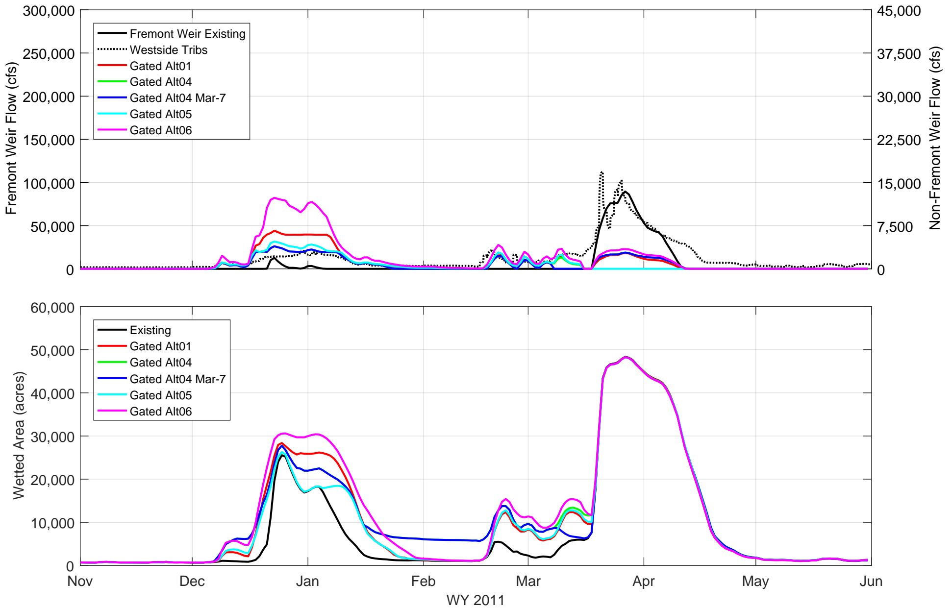
YOLO BYPASS DISCHARGES AND WET AREA BY ALTERNATIVE WATER YEAR 2011
