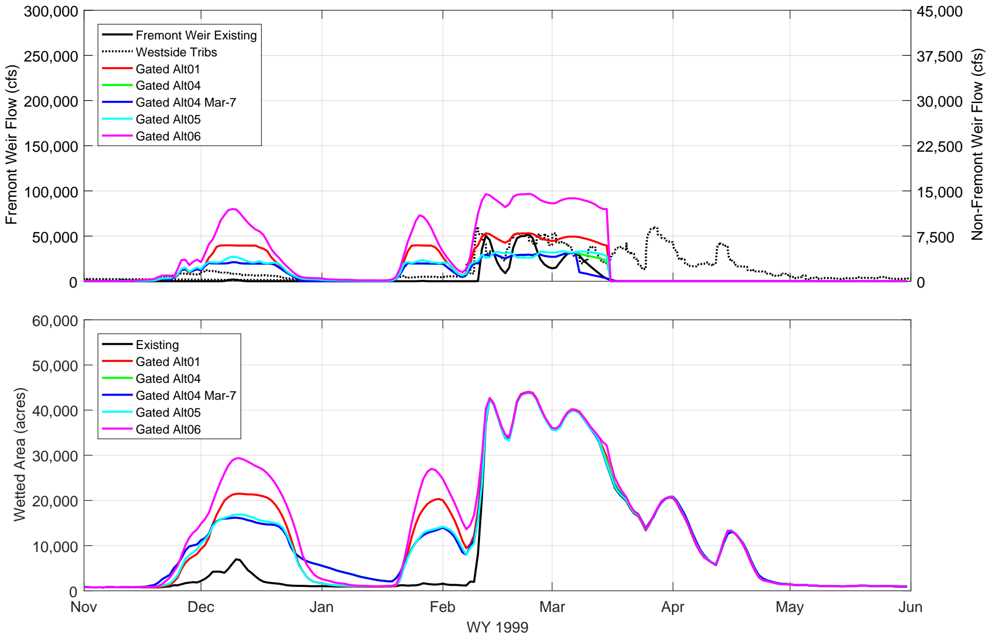
YOLO BYPASS DISCHARGES AND WET AREA BY ALTERNATIVE WATER YEAR 1999
