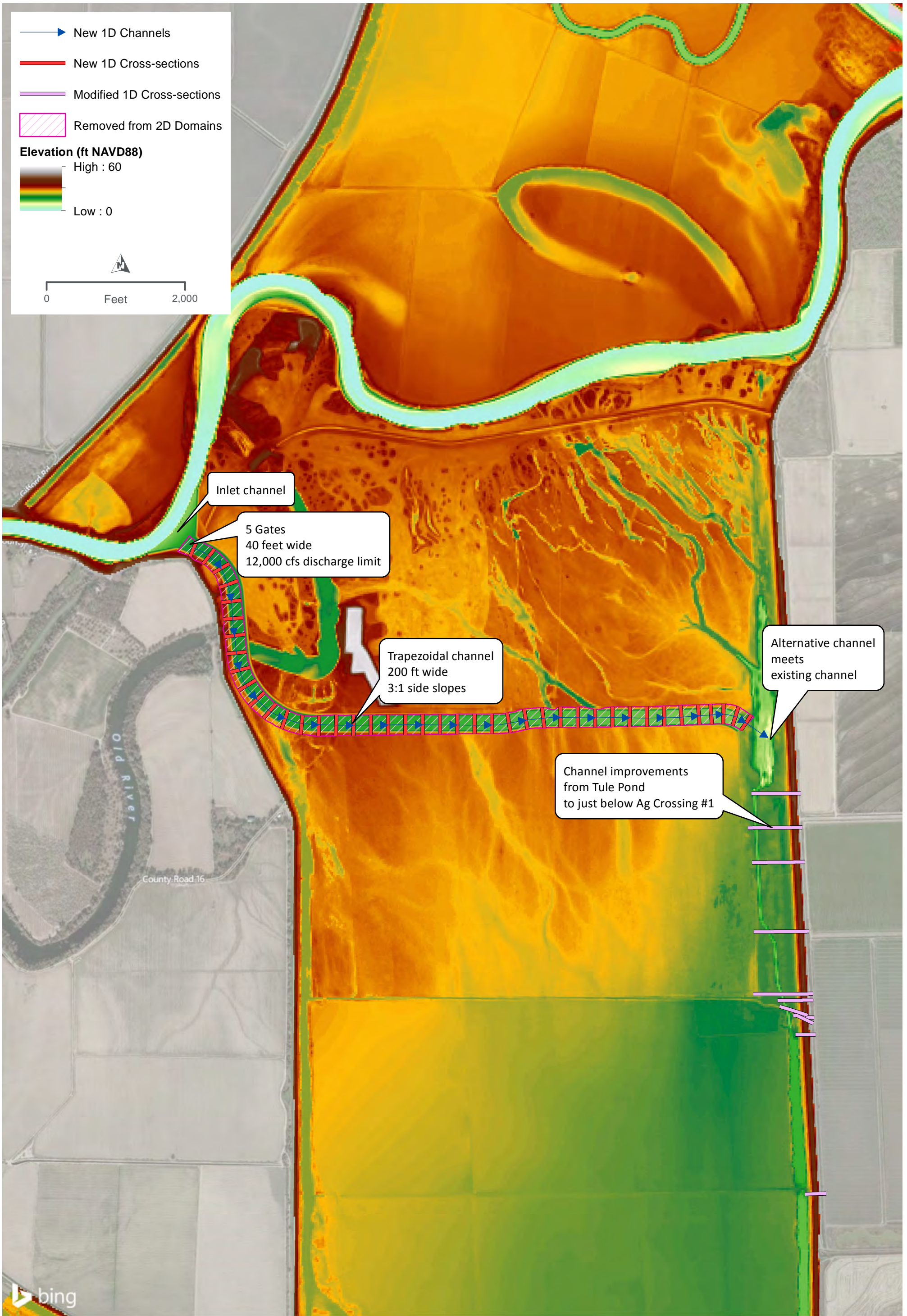
ALTERNATIVE #6 MODEL FEATURES 12,000 CFS AT WESTERN ALIGNMENT FIGURE 8
