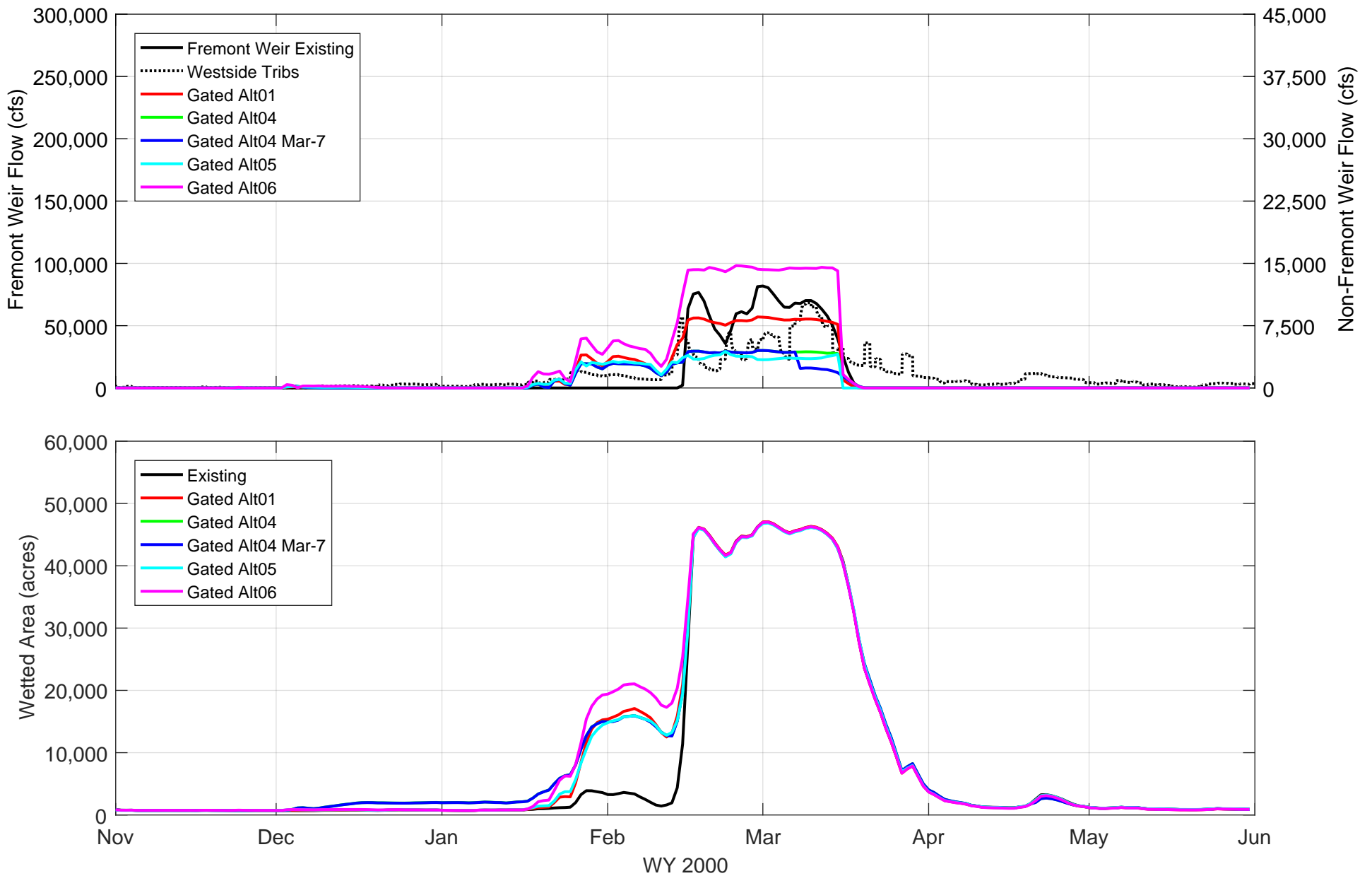
YOLO BYPASS DISCHARGES AND WET AREA BY ALTERNATIVE WATER YEAR 2000
