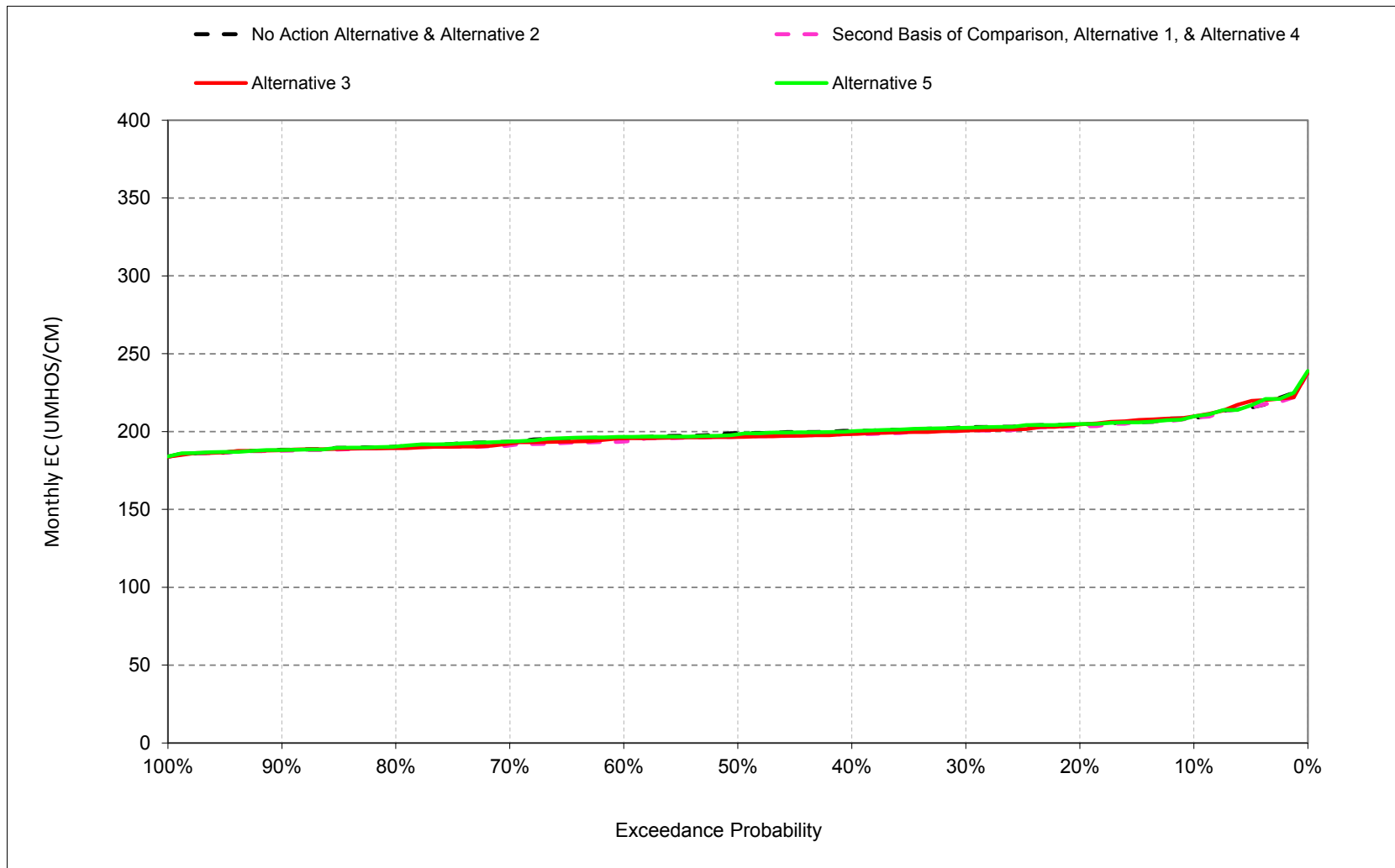
Figure 6E.B.14.3. Barker Slough North Bay Aqueduct Intake Salinity, Electrical Conductivity, December
