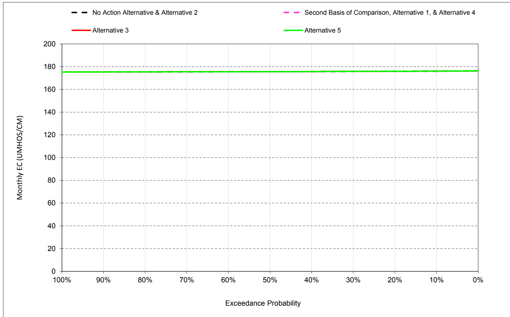
Figure 6E.B.1.1. Sacramento River d/s of Steamboat Slough Salinity, Electrical Conductivity, October
