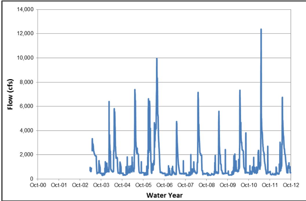
2 Figure 5.11 Historical Water Years 2003-2012 Trinity River Mean Daily Flows at 3 Douglas City
