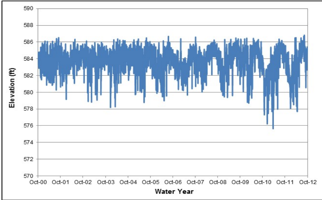
Figure 5.19 Historical Water Year 2001 - 2012 Keswick Reservoir Elevation
