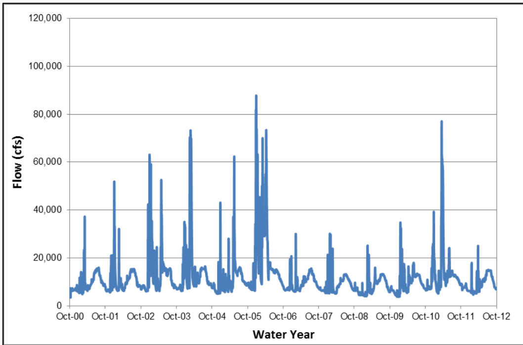
Figure 5.20 Historical Water Year 2001 - 2012 Sacramento River Mean Daily Flows at Bend Bridge
