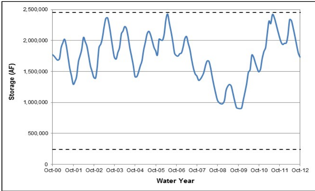
2 Figure 5.7 Historical Water Years 2001-2012 Trinity Lake Storage 1
