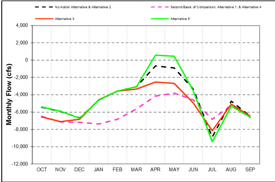
2 Figure 5.79 Old and Middle River, Dry Year Long-Term Average Flow 3 Bookmark not defined. Error! Bookmark not defined.
