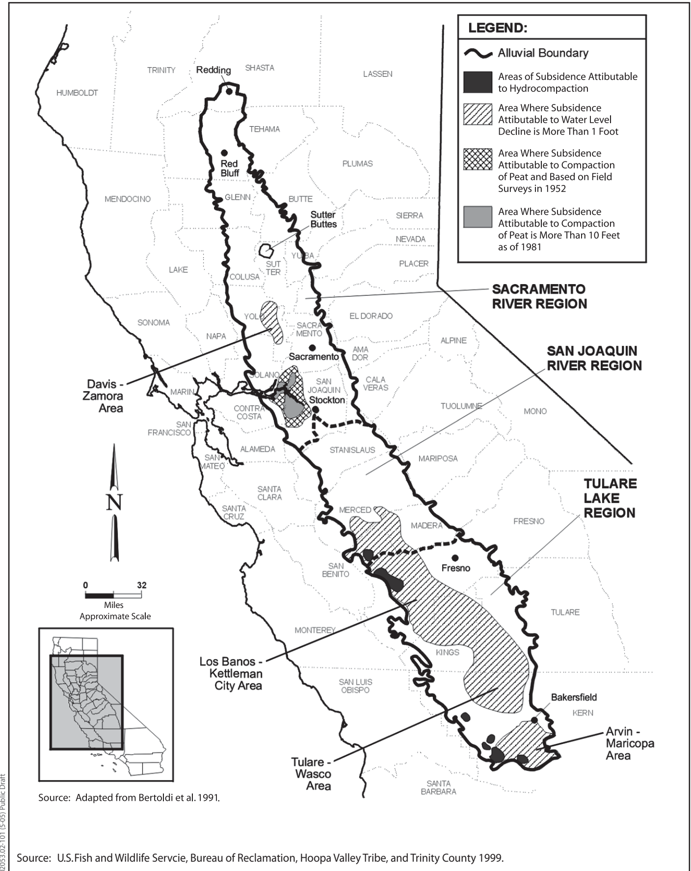
Figure 5.4-1 Aerial Extent of Land Subsidence in the Central Valley as a Result of Declines in Groundwater Elevations
