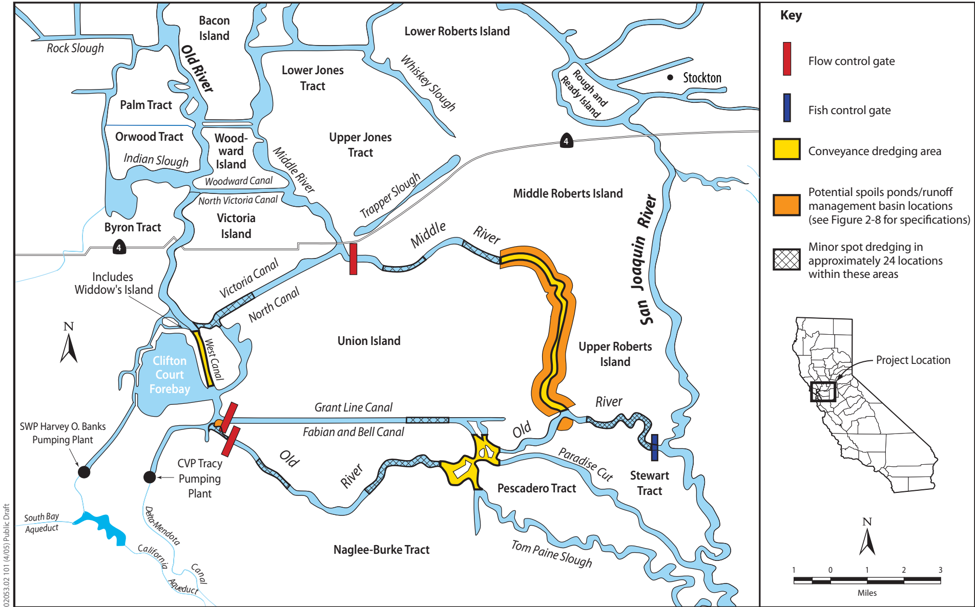
Figure 2-3 Preferred Physical/Structural Component
