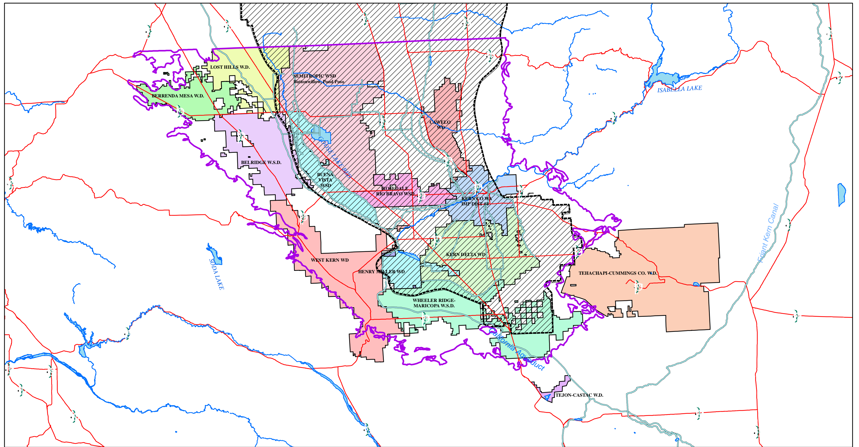
Figure 3-3c. Non-CVP Potential Exchanges Kern County Water Agency
