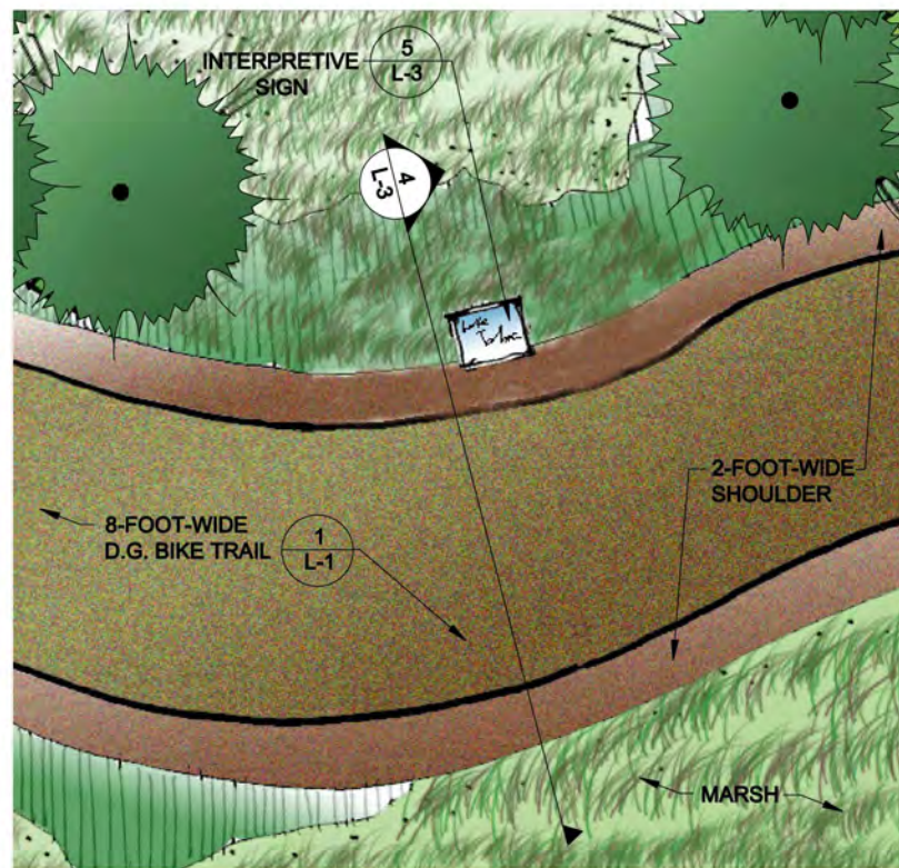
1 VIEW POINT (MIN.) L-3 SCALE: NTS
