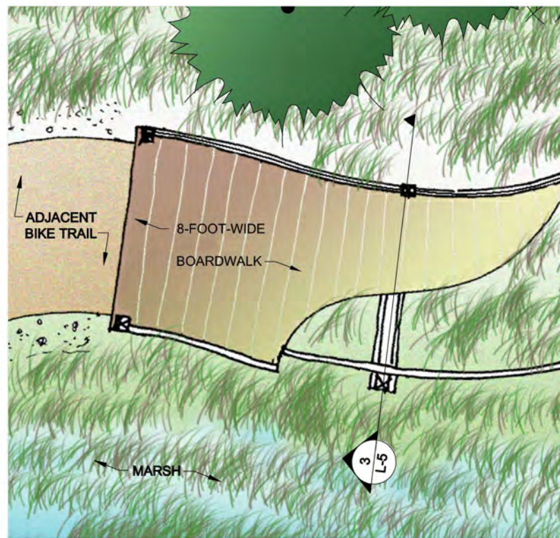
1 BOARDWALK (MIN.) L-5 SCALE: NTS
