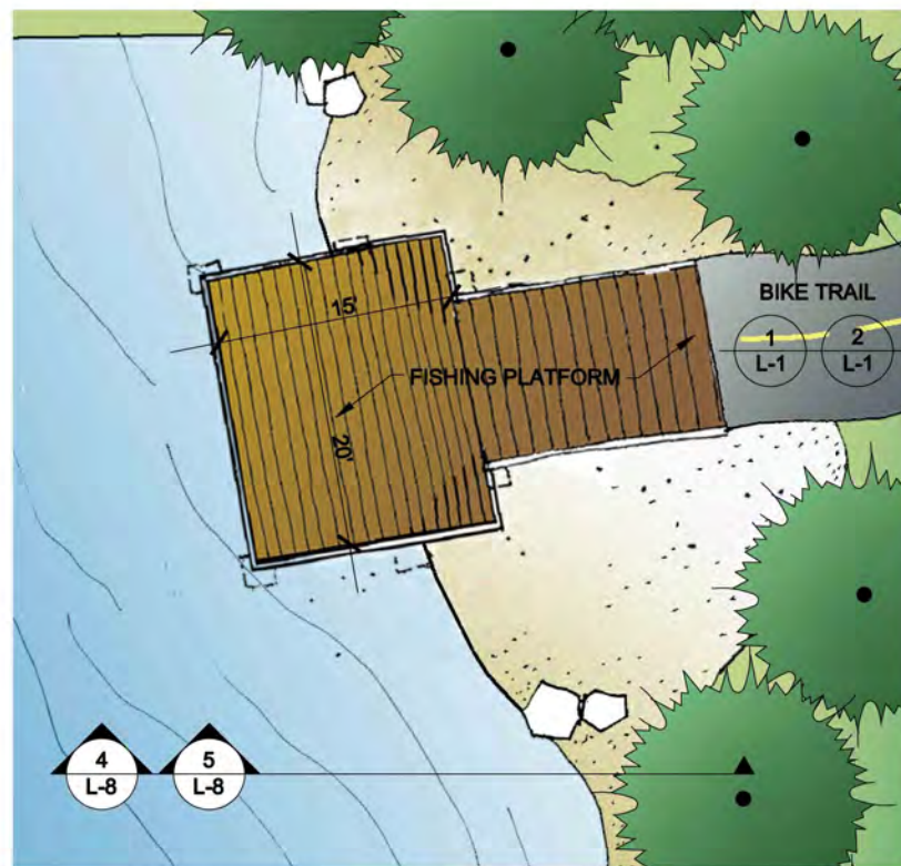
1 L-8 FISHING PLATFORM (MIN.) SCALE: NTS PLAN VIEW
