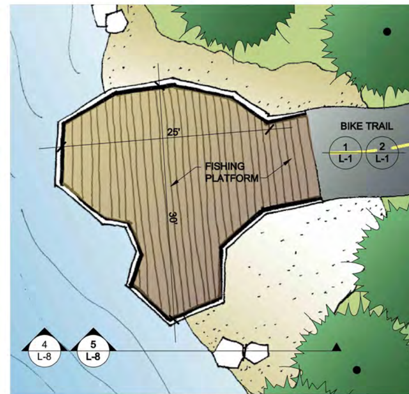
3 L-8 FISHING PLATFORM (MAX.) SCALE: NTS
