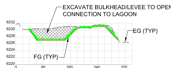
SECTION E-E
