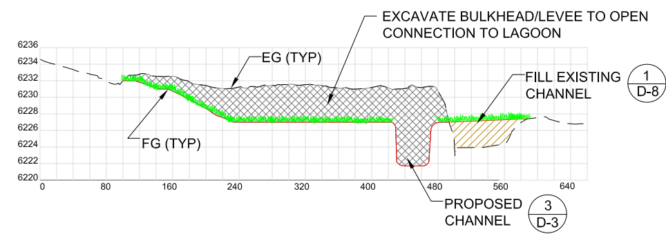
SECTION D-D SCALE 1"=80'; 1H:10V
