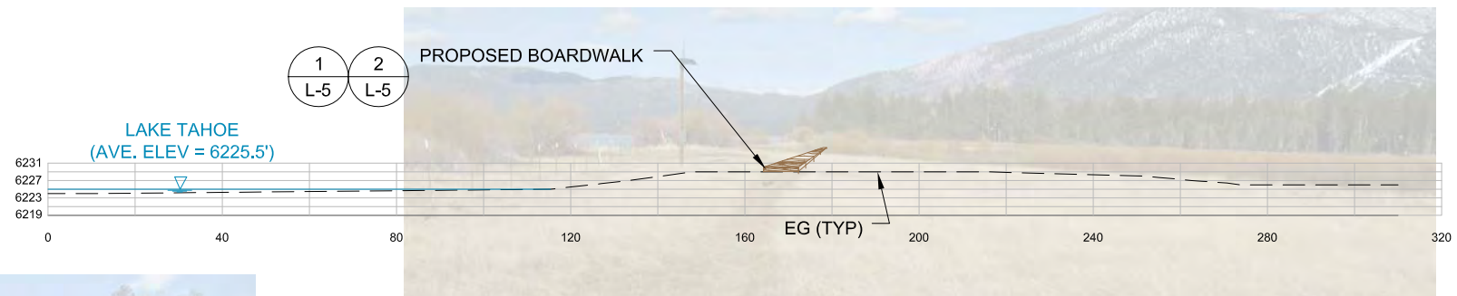
SECTION B-B
