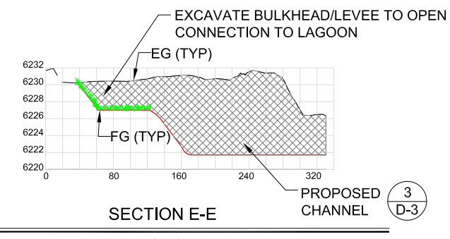
SECTION E-E SCALE 1"=80'; 1H:10V
