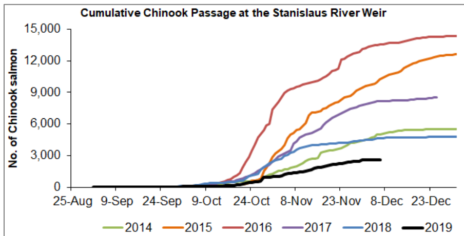
Figure 5-5. Cumulative Chinook salmon passage through December 3, 2019, at the Stanislaus River weir near Riverbank. Data courtesy of FISHBIO.
