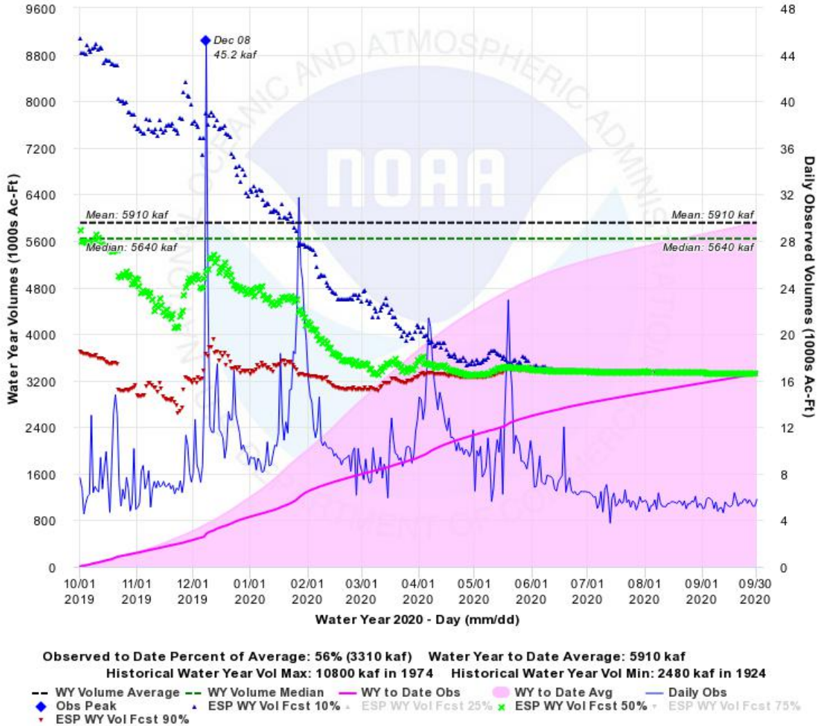
Figure 5. WY 2020 forecasted (10%, 50%, 90% exceedance) and actual daily and cumulative inflow volume at Shasta Lake. Source: https://www.cnrfc.noaa.gov/water_resources_update.php
