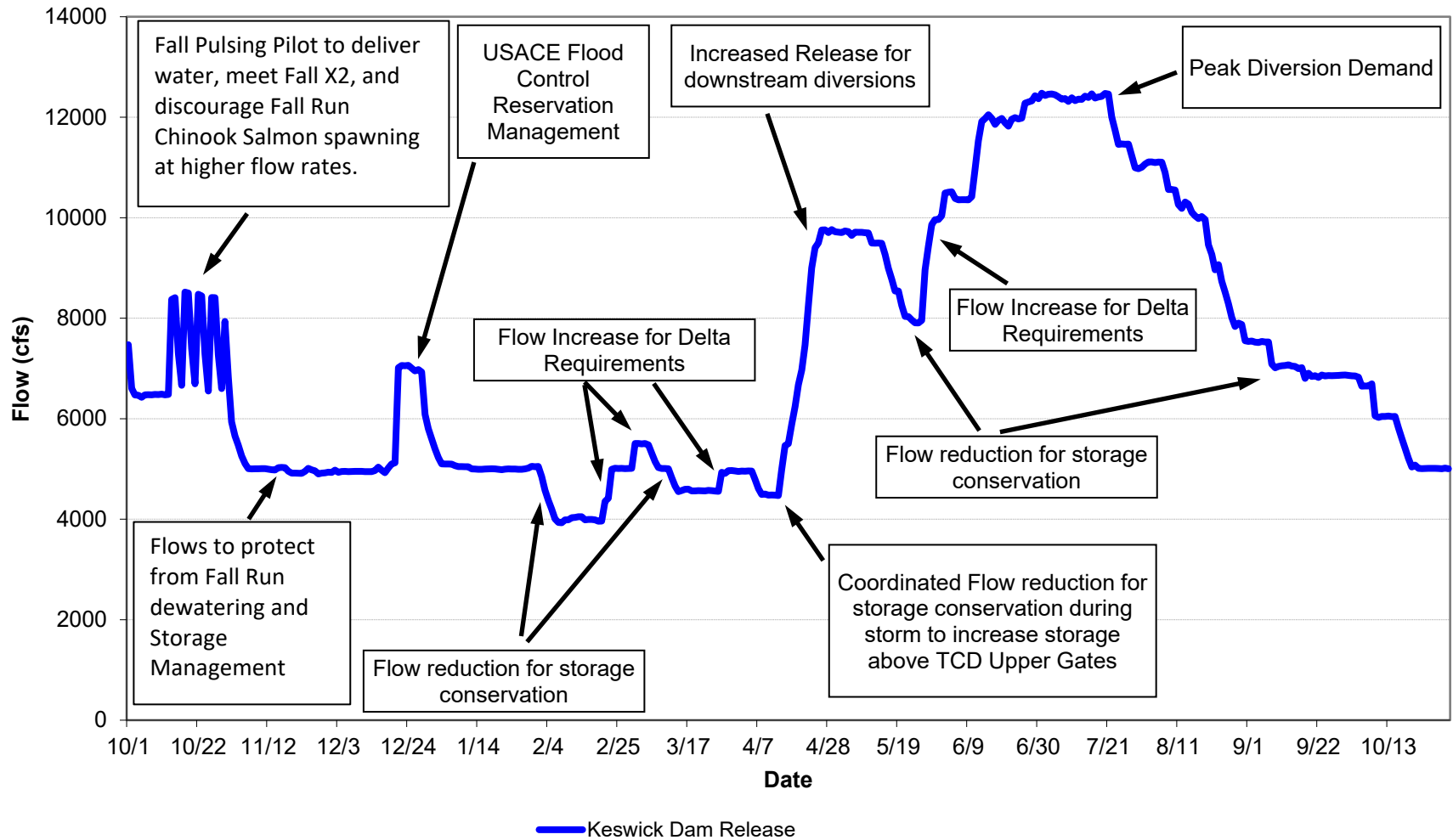
Figure 7. Sacramento River Releases from 10/1/2019 - 10/31/2020 with major events highlighted
