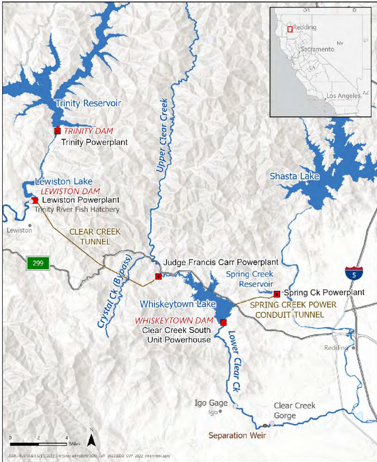
Figure 61. Clear Creek facilities in the Trinity Division of the Central Valley Project.
