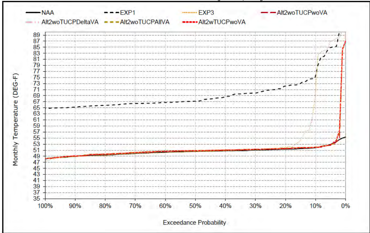
Figure 71. Exceedance plot of modeled water temperatures in Clear Creek in July. The proposed action is represented by Alt2woTUCPwoVA (Alt2v1).
