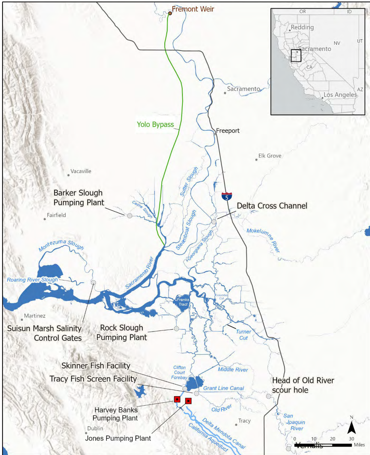
Figure 109. Map of key Bay-Delta Division facilities.
