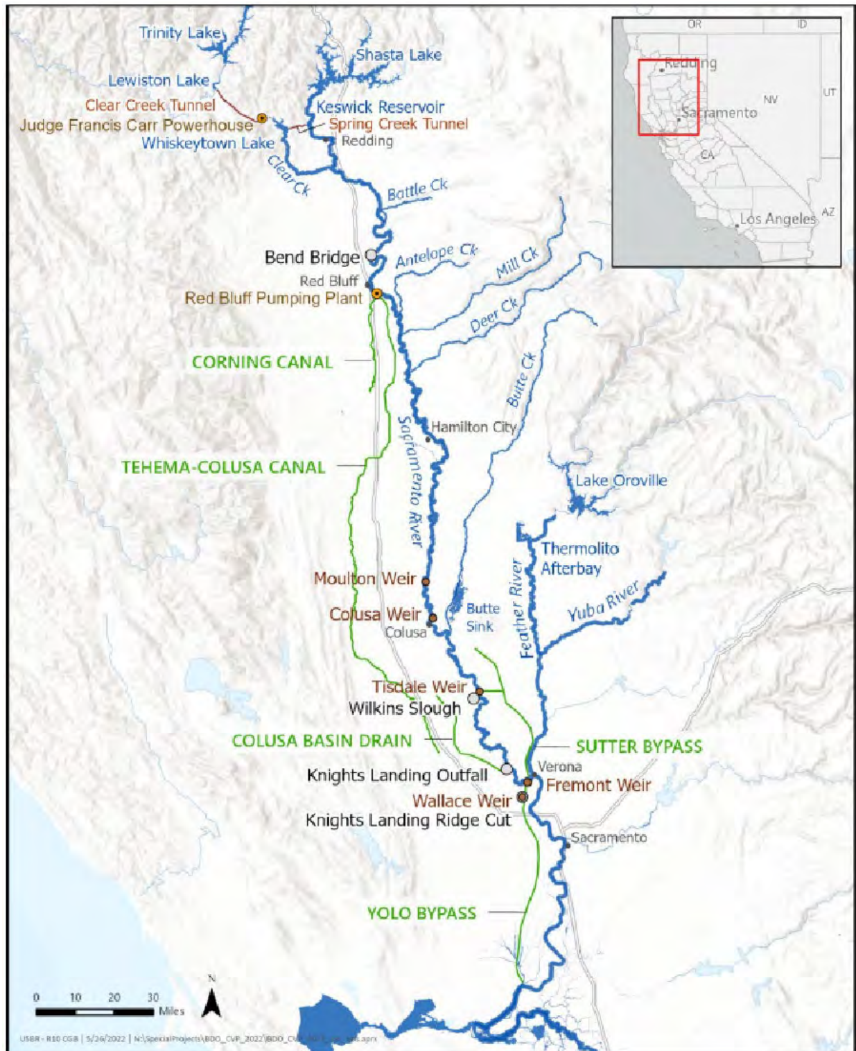
Figure 35. Sacramento River Facilities in the Shasta and Sacramento Divisions of the Central Valley Project and Flood Control Weirs and Bypasses.
