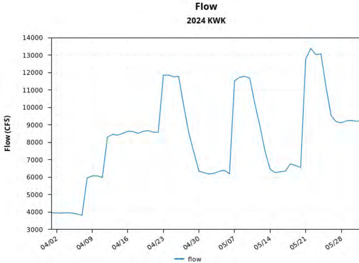
Figure 59. Flows (in cubic feet per second) in the Sacramento River at Keswick (KWK) Dam for April through May of 2024 showing the three managed Spring pulse flows.
