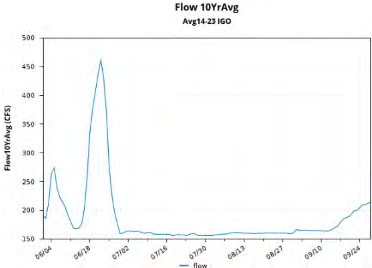
Figure 65. 10-year average flows (2014–2023) at Igo gauge in Clear Creek under current operations of 200 cubic feet per second (cfs) and 150 cfs base flows, pulse flows, and natural flows.
