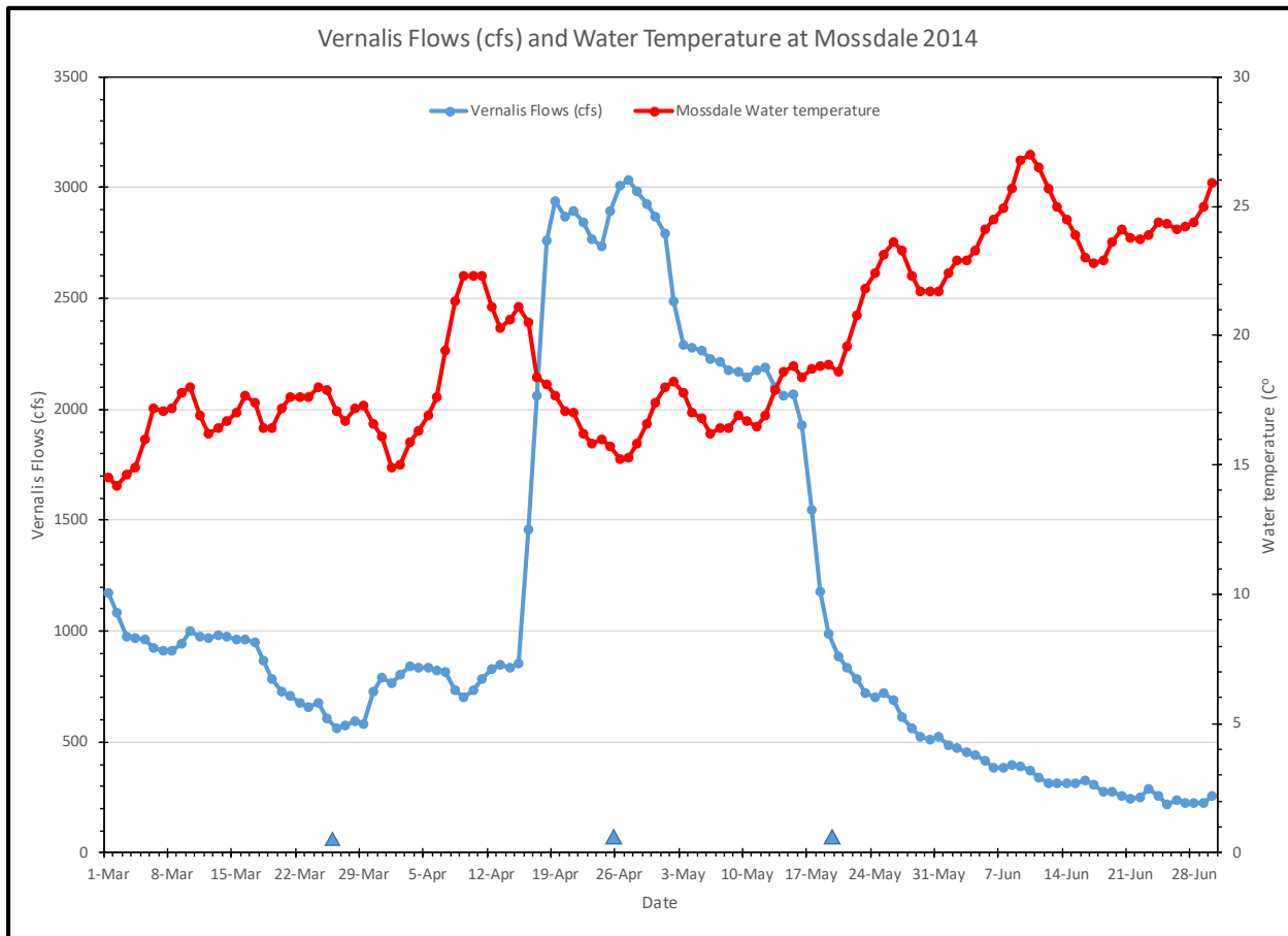
Figure 8. Vernalis Flows and Mossdale Water Temperatures March through June 2014
