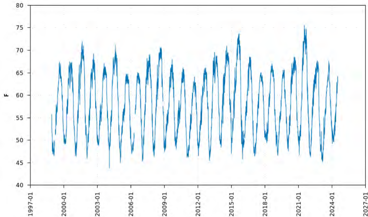
Figure 98. American River Below Watt Avenue Bridge Daily Average Water Temperatures (°F) 1998–2024.
