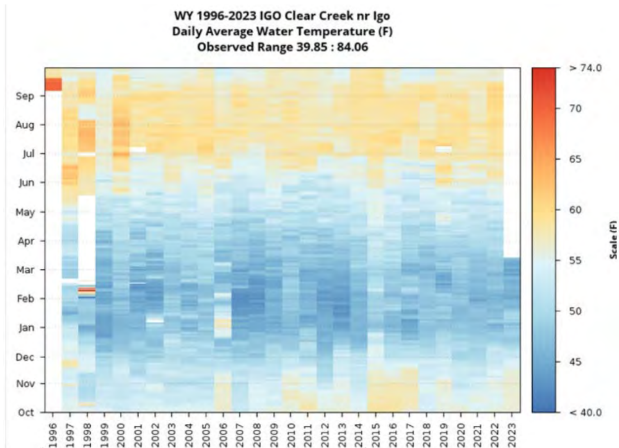
Figure 64. Clear Creek near Igo Daily Average Water Temperature (°F) for Water Year 1996–2023.
