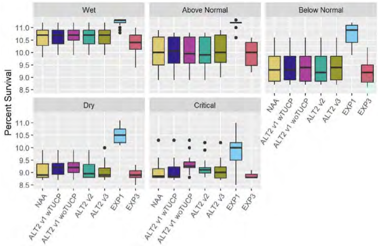
Figure 142. Boxplots of modeled mean survival between Red Bluff Diversion Dam and the Delta Cross Channel all modeled scenarios by water year type.
