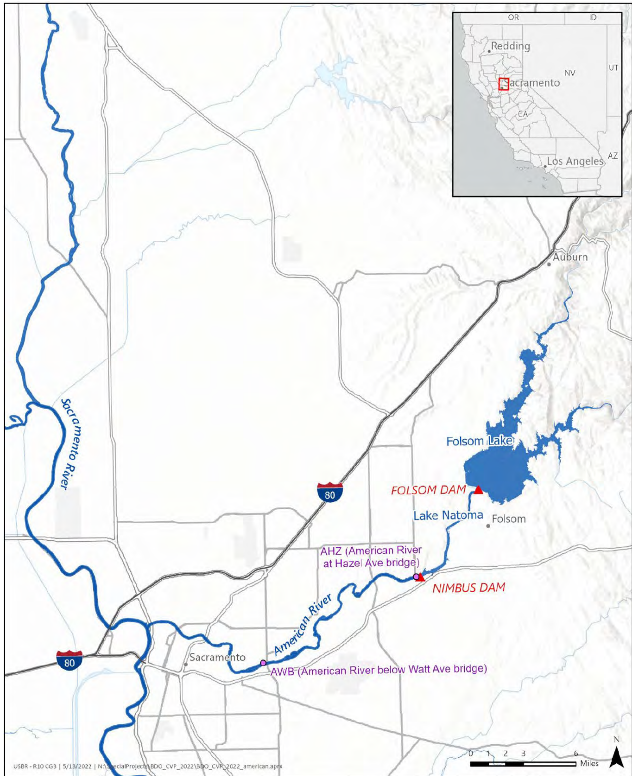
Figure 85. Facilities in the American River Division of the Central Valley Project.
