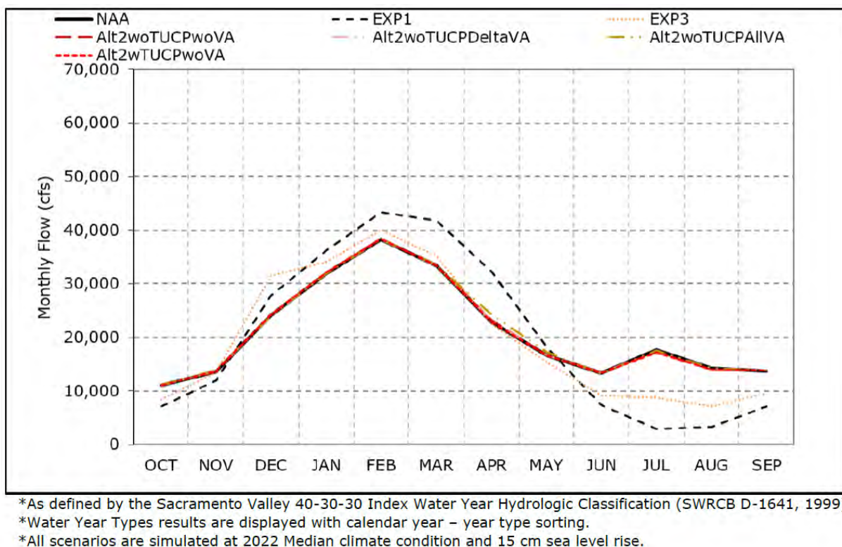
Figure 123. Modeled Freeport flow (cubic feet per second [cfs]) over all water year types.
