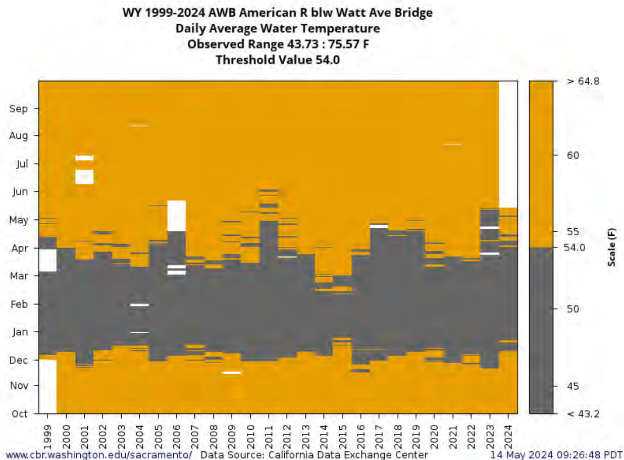
Figure 99. American River below Watt Avenue Bridge temperatures.
