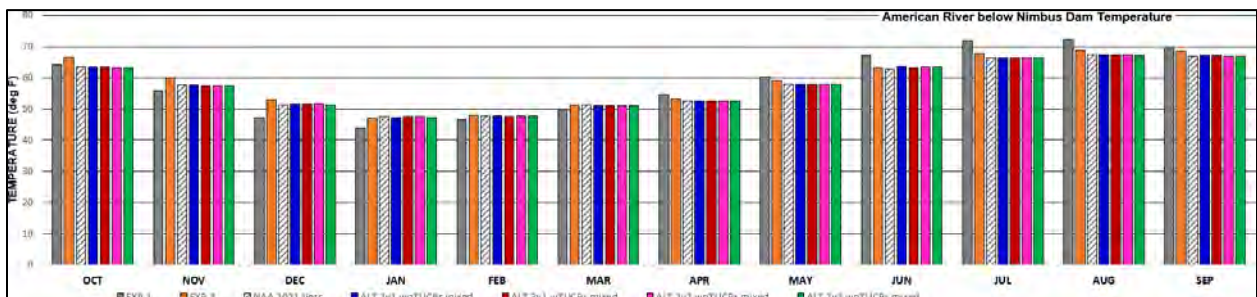
Figure 8. American River below Nimbus Dam monthly water temperature at the 50-percent exceedance probability.
