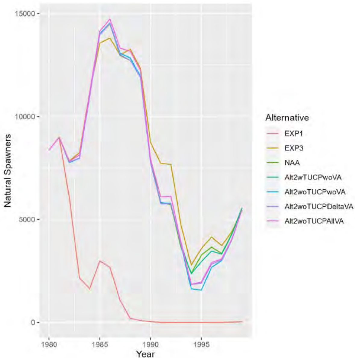
Figure 162. Expected annual abundances of natural-origin Sacramento River winter-run Chinook salmon spawners in the Upper Sacramento River from deterministic model runs.
