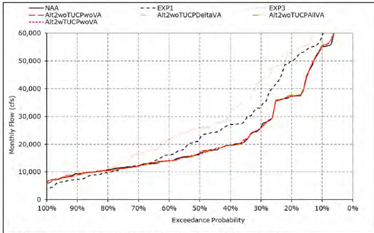
Figure 130. Exceedance plot of modeled Sacramento River Flow (cubic feet per second) at Freeport during December.
