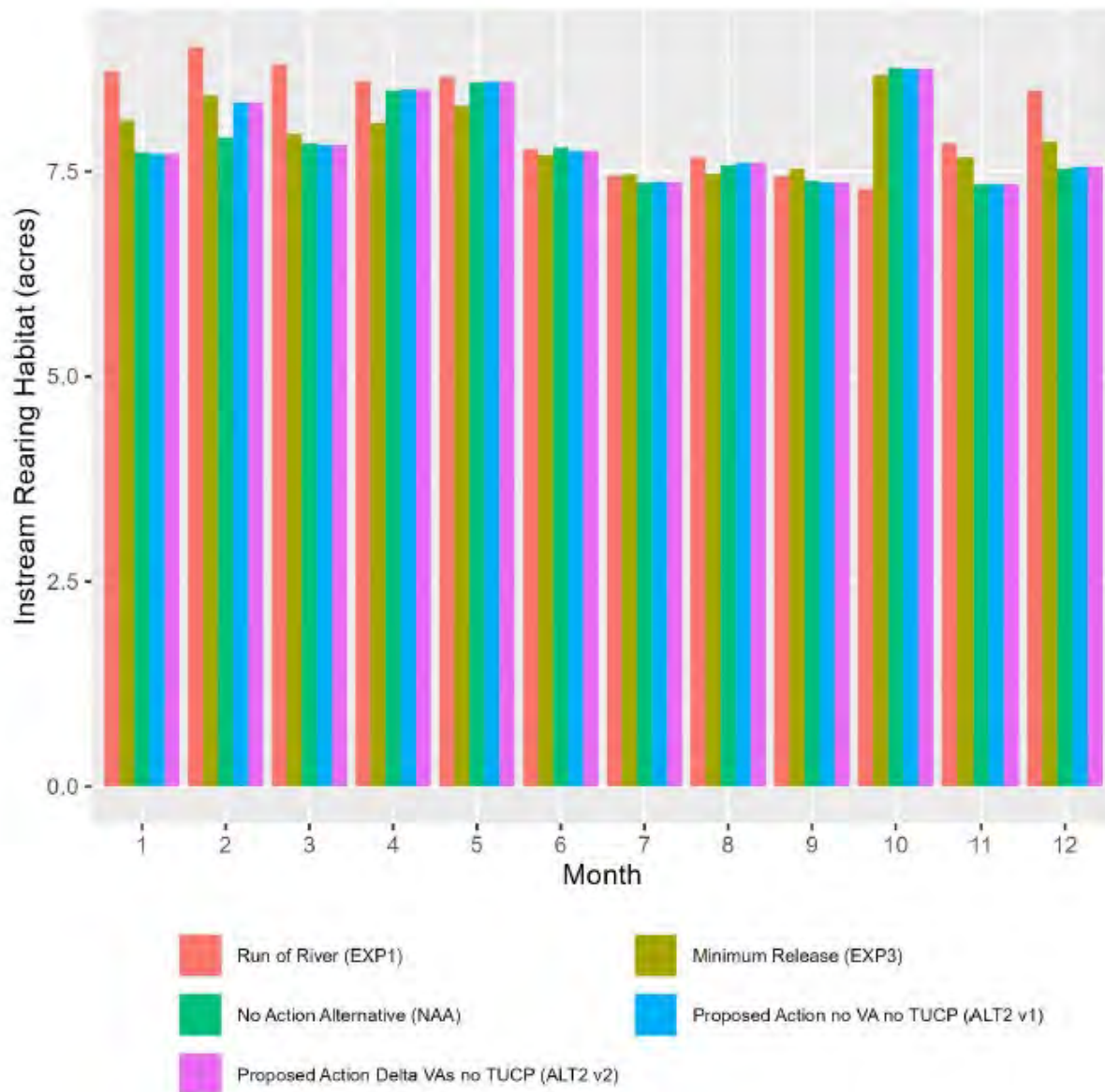
Figure 106. Estimated instream rearing habitat for juvenile California Central Valley steelhead in the Stanislaus River.
