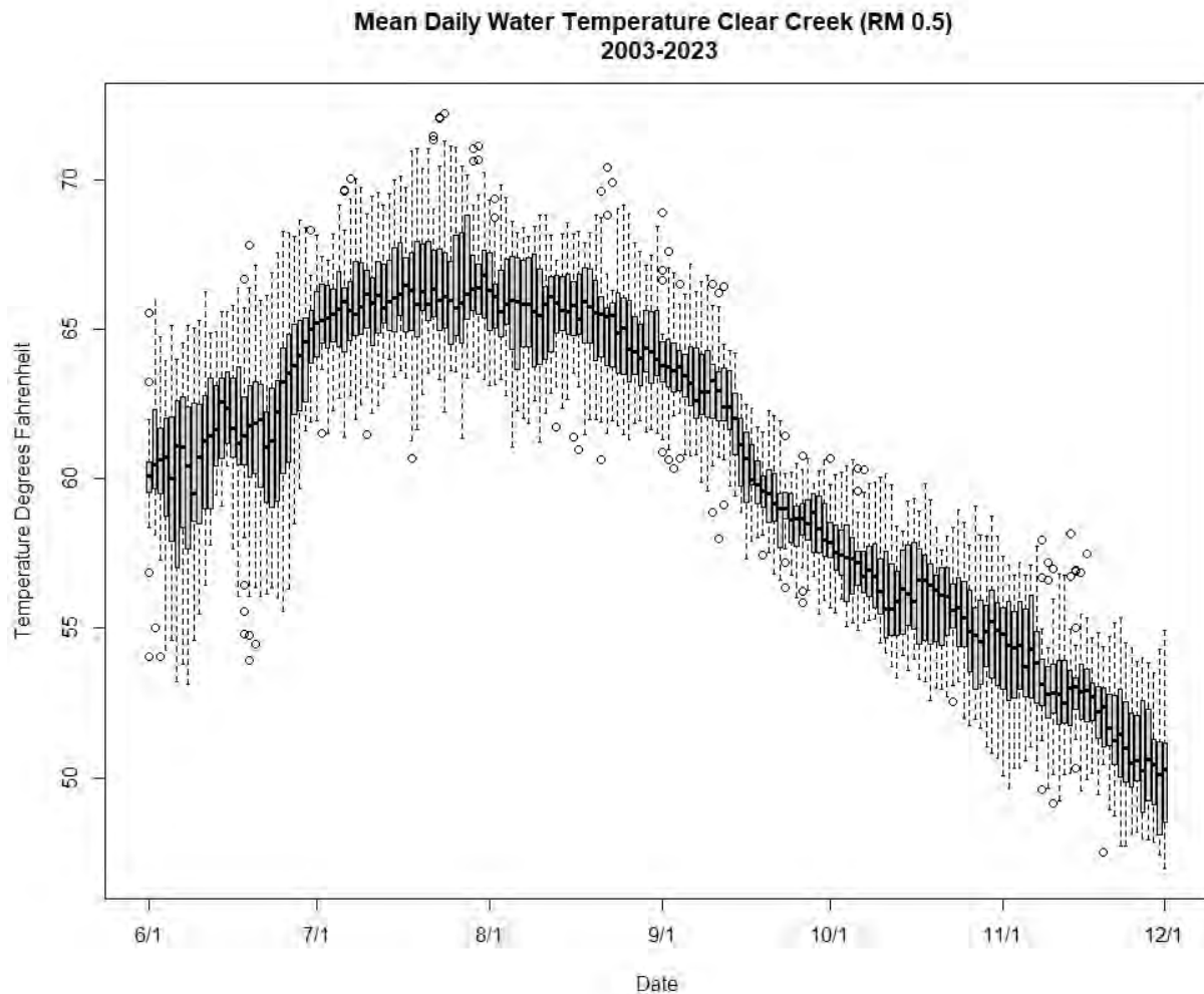
Figure 68. Historic water temperatures in Clear Creek just above the confluence with Sacramento River, 2003–2023.
