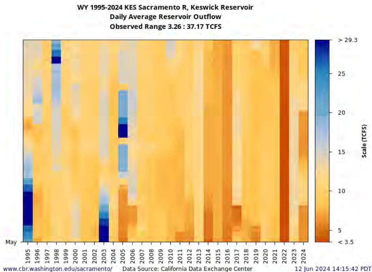
Figure 55. Keswick Reservoir daily average outflow, 1995–2024. There is a 2-week period (May 1–14) between the Bin determination (April 30) and the beginning of the temperature management season (May 15). High releases during this period could reduce the available cold water pool, especially in the drier years. Flows over the 29-year period shown are generally in the 7,000 to 8,500 cfs range during these 2 weeks (based on the most recent 10-year average, 2014–2023), but can vary widely, by an order of magnitude, from 3,250 to 37,000 cfs.
