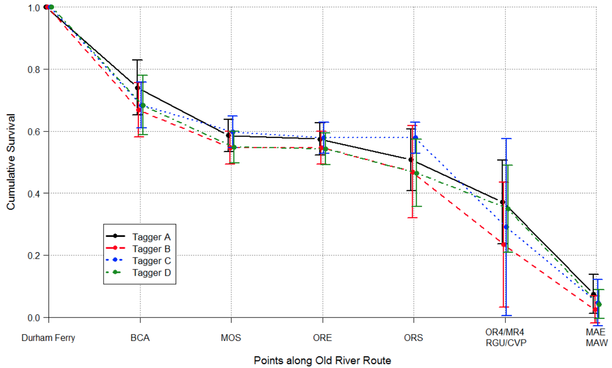
Figure 10. Cumulative survival from releases at Durham Ferry to various points along the Old River route to Chipps Island by surgeon (2012 study). Error bars are 95% confidence intervals.
