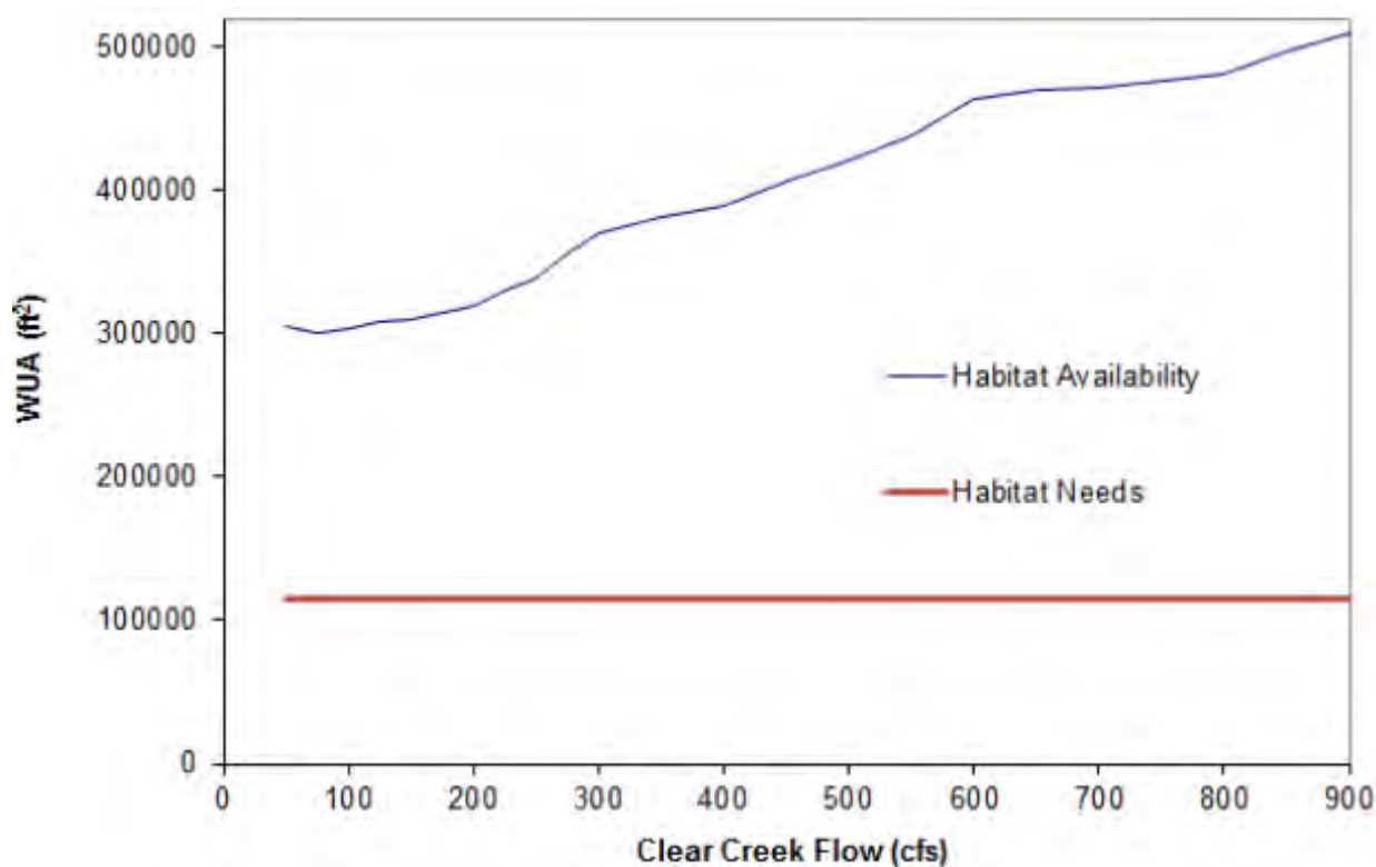
Figure 80. Central Valley spring-run Chinook salmon fry rearing flow-habitat availability relationship and habitat needs.
