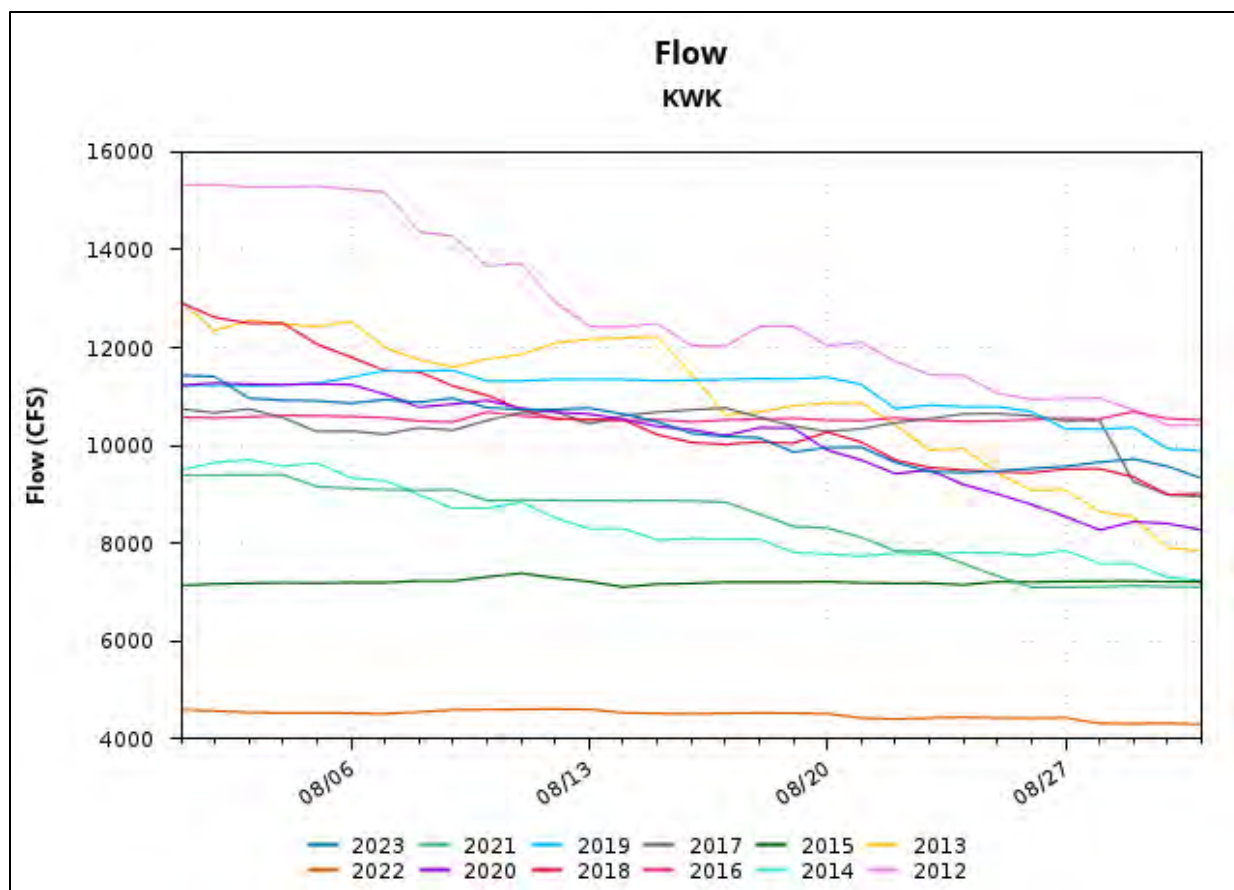
Figure 57. August flows (in cubic feet per second) at Keswick (KWK) gauge from 2012 to 2023.
