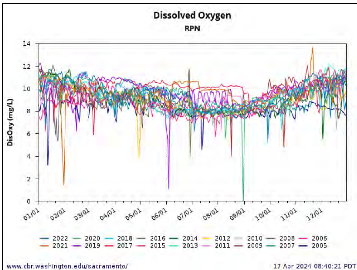
Figure 104. Stanislaus River at Ripon (RPN) daily average dissolved oxygen (mg/L) for years 2005–2022.
