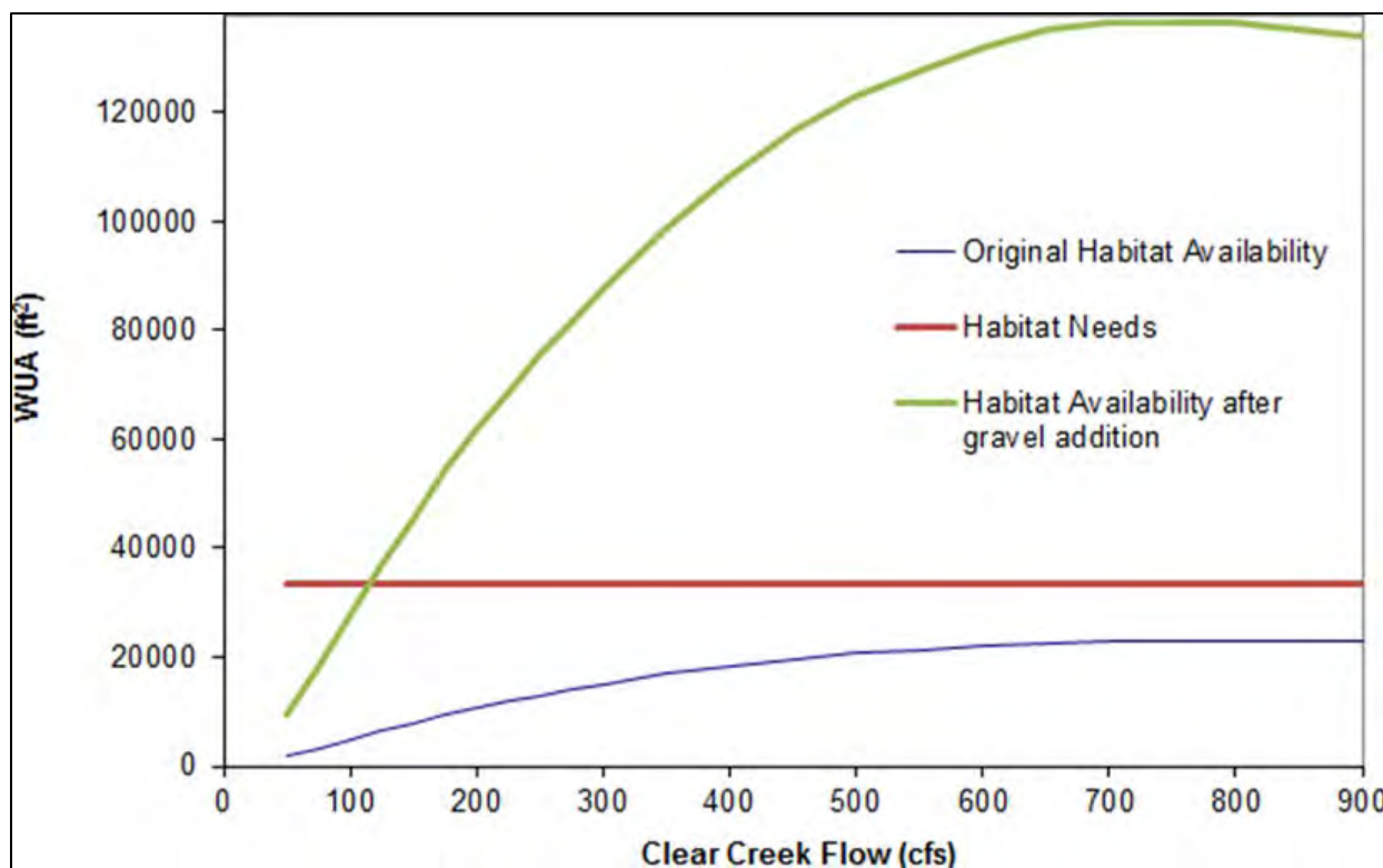
Figure 79. Weighted usable area (WUA) curve which includes the increased spawning habitat availability after gravel addition projects. 120,000 square feet (ft²) is approximately 2.75 acres.
