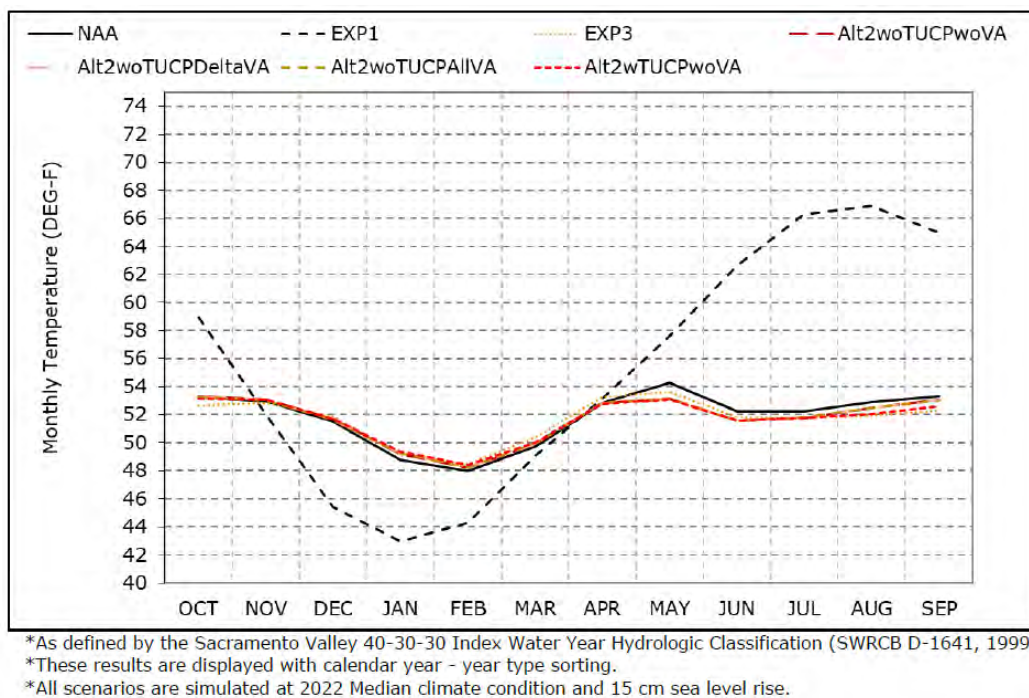
Figure 43. Sacramento River below Keswick, long-term average temperature.
