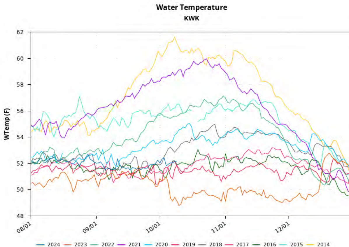
Figure 48. Water temperatures at Keswick gauge from August through December of 2014–2024.
