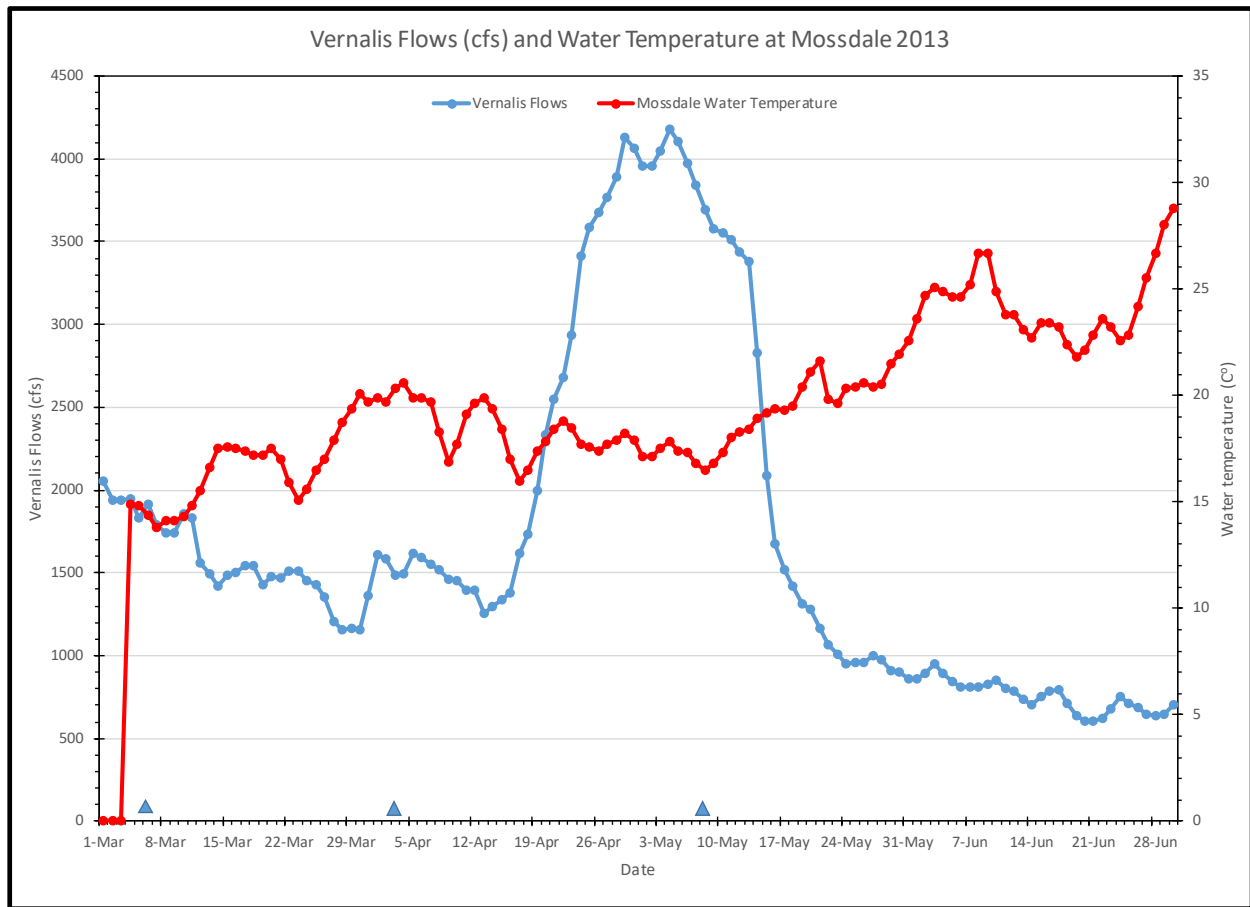
Figure 7. Vernalis Flows and Mossdale Water Temperatures March through June 2013
