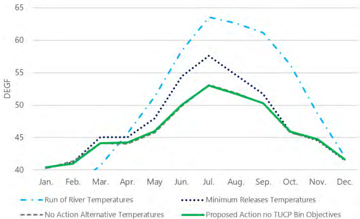
Figure 102. HEC-5Q modeled temperatures (°F) at Orange Blossom in the Stanislaus River.
