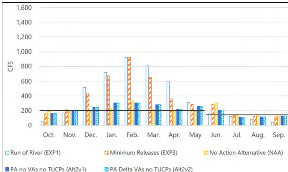
Figure 76. Monthly releases from Whiskeytown Dam for all modeling scenarios. Solid blue bars represent the proposed action (Alt2v1). Black 200 cfs line and gray 150 cfs line added to show current operations.
