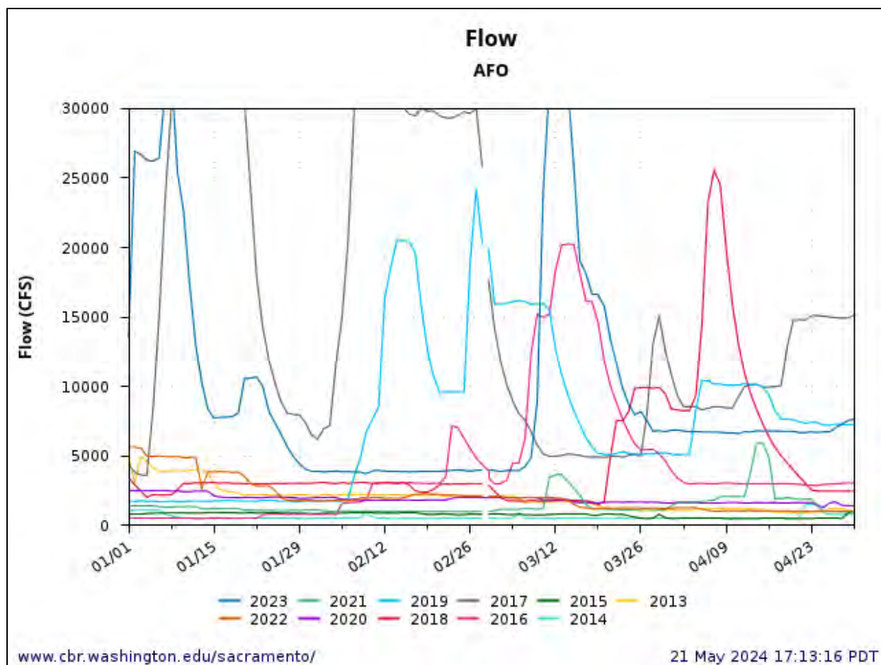
Figure 92. Flow at American River at Fair Oaks (AFO) 2013–2023.
