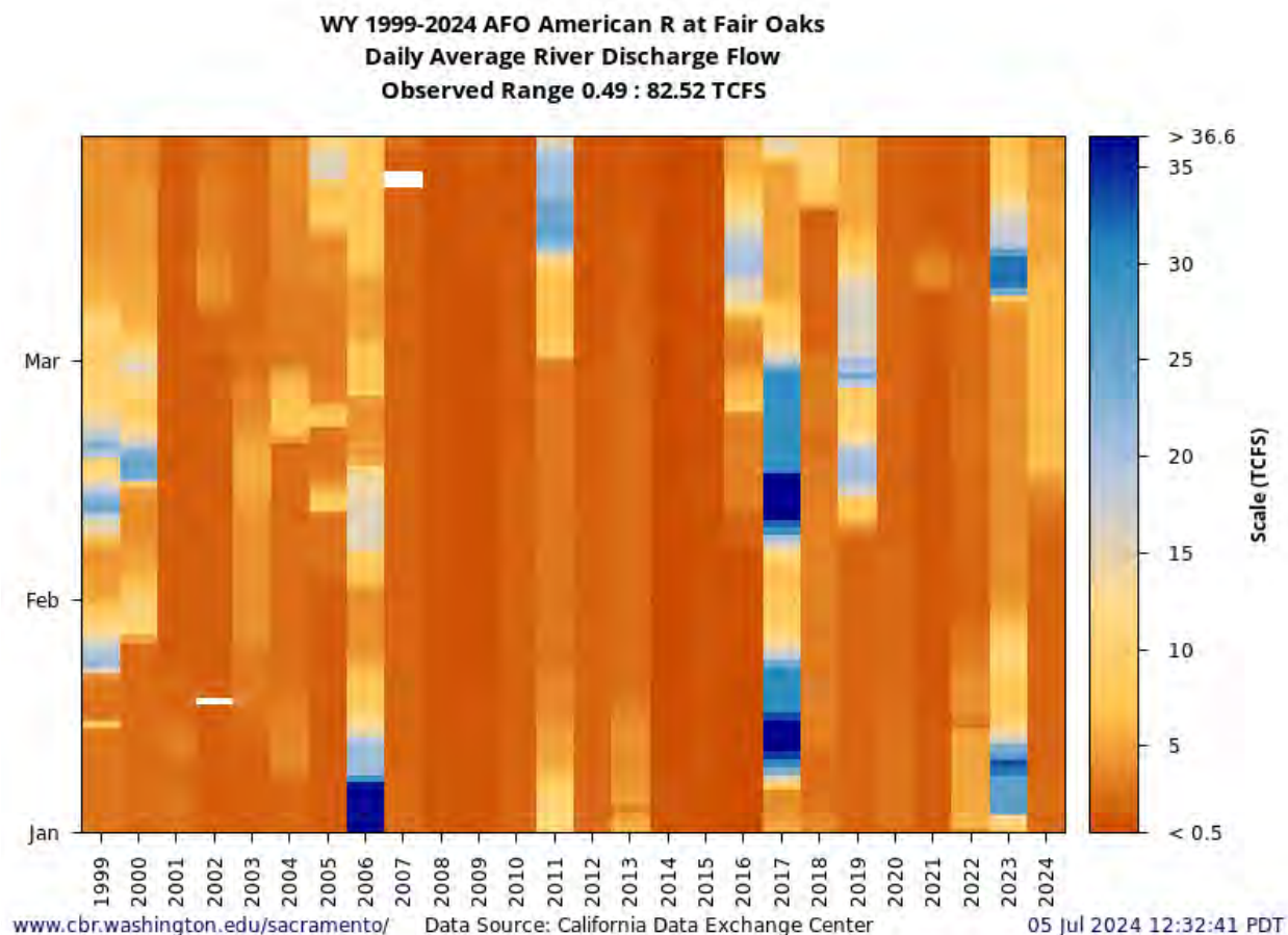
Figure 91. Water Year 1999–2024 American River at Fair Oaks (AFO) Daily Average River Discharge Flow (thousand cubic feet per second [TCFS]).
