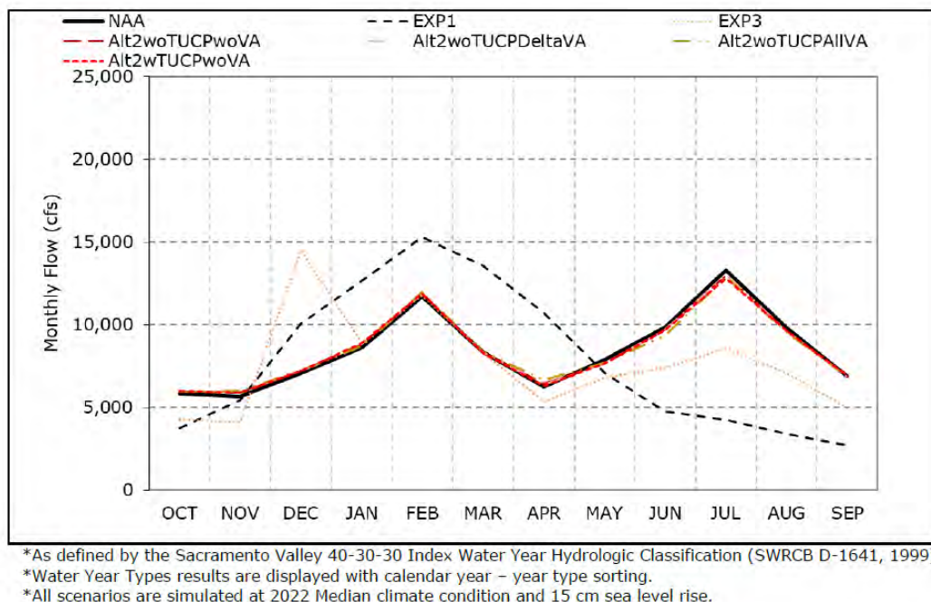
Figure 42. Sacramento River flow downstream of Keswick Reservoir, long-term average flow.
