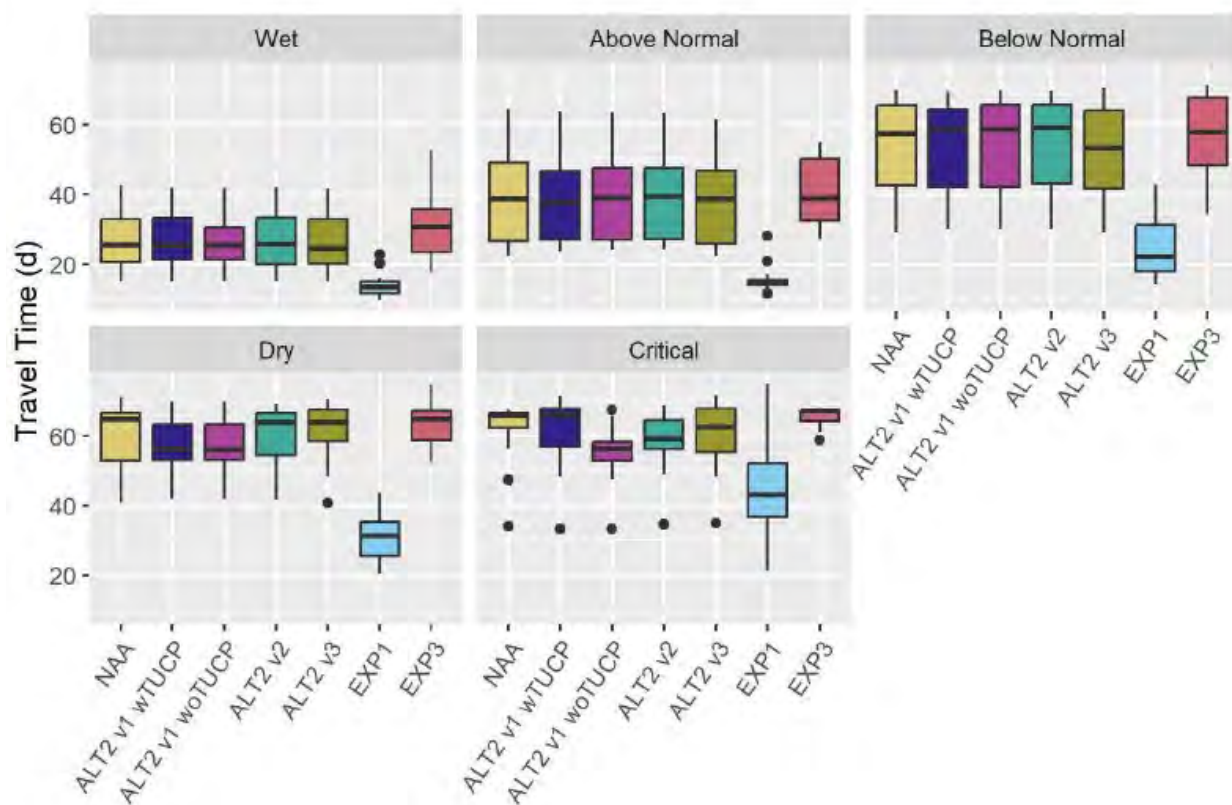
Figure 143. Boxplots of modeled mean travel time (days) between Red Bluff Diversion Dam and the Delta Cross Channel for all modeled scenarios by water year type.
