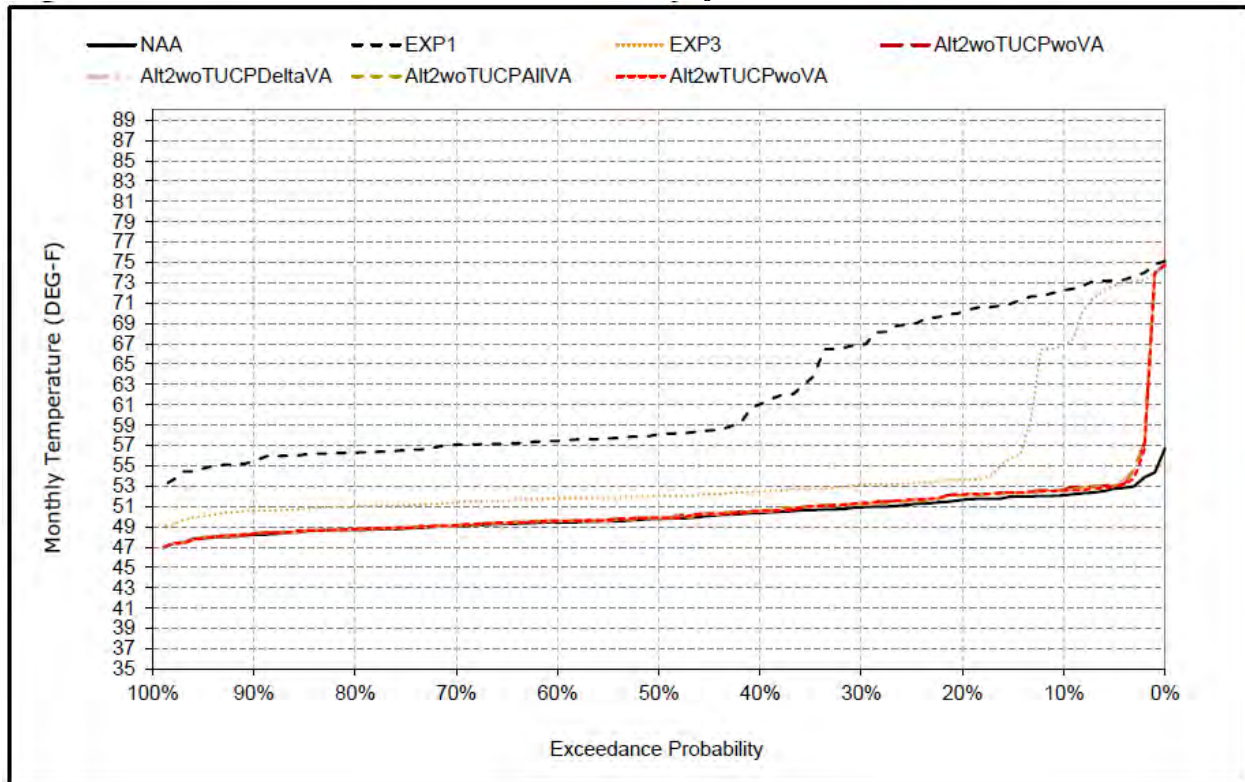
Figure 74. Exceedance plot of modeled water temperatures in Clear Creek in October. The proposed action is represented by Alt2woTUCPwoVA (Alt2v1).
