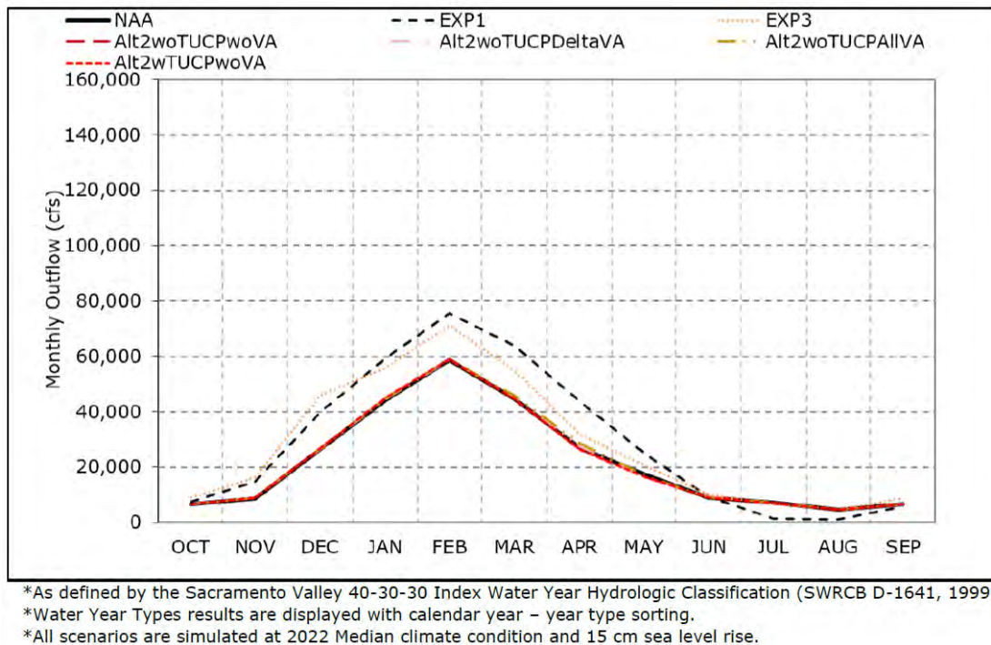
Figure 127. Modeled Delta outflow (cubic feet per second [cfs]) over all water year types.
