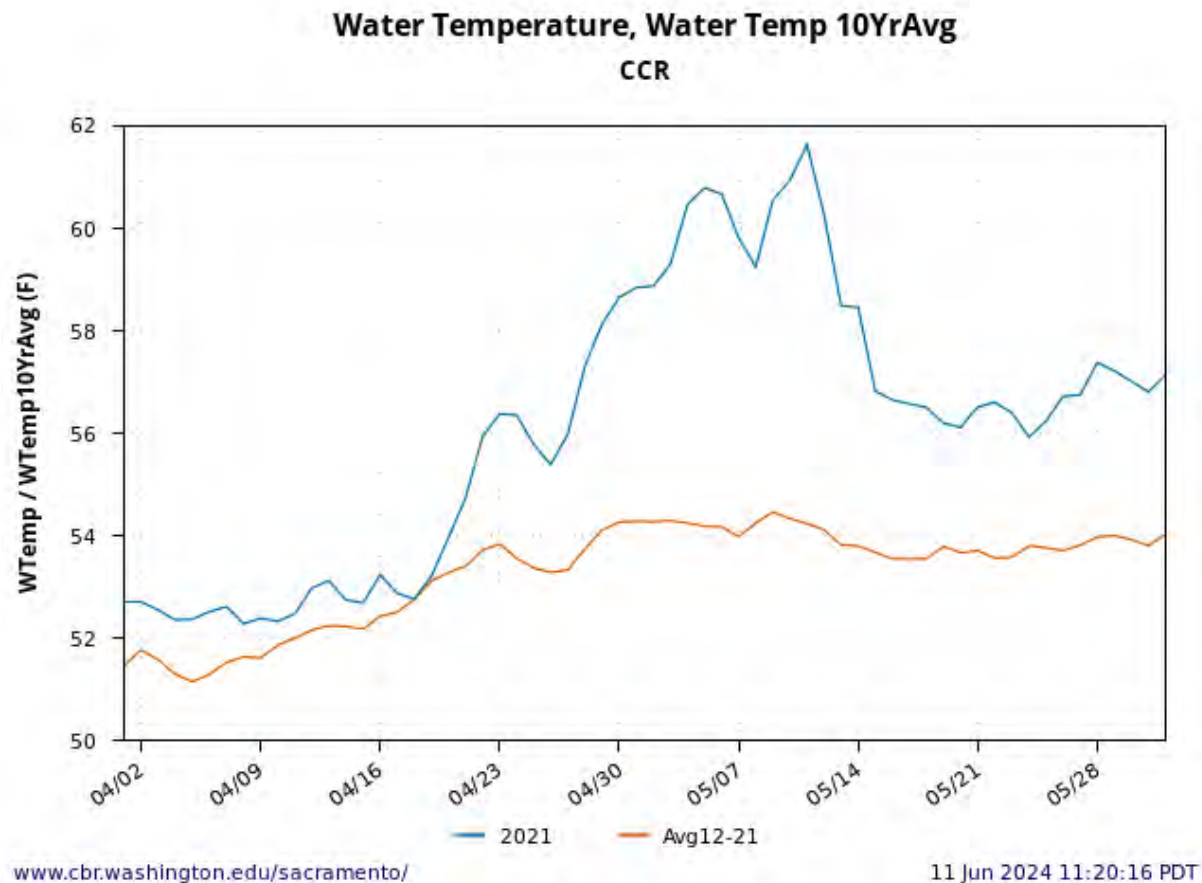
Figure 50. Water temperature in the Sacramento River above Clear Creek (CCR) in April and May 2021, versus the 10-year average.
