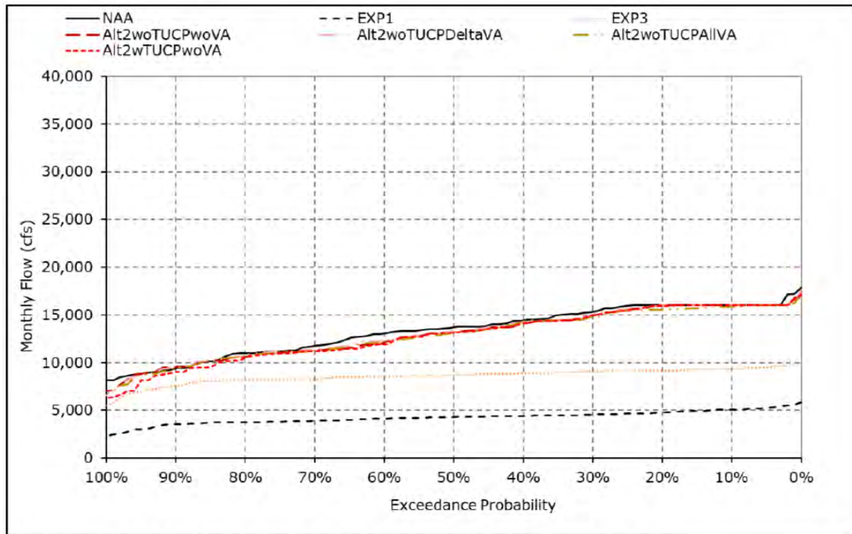
Figure 58. Sacramento River flow downstream of Keswick Reservoir, July.
