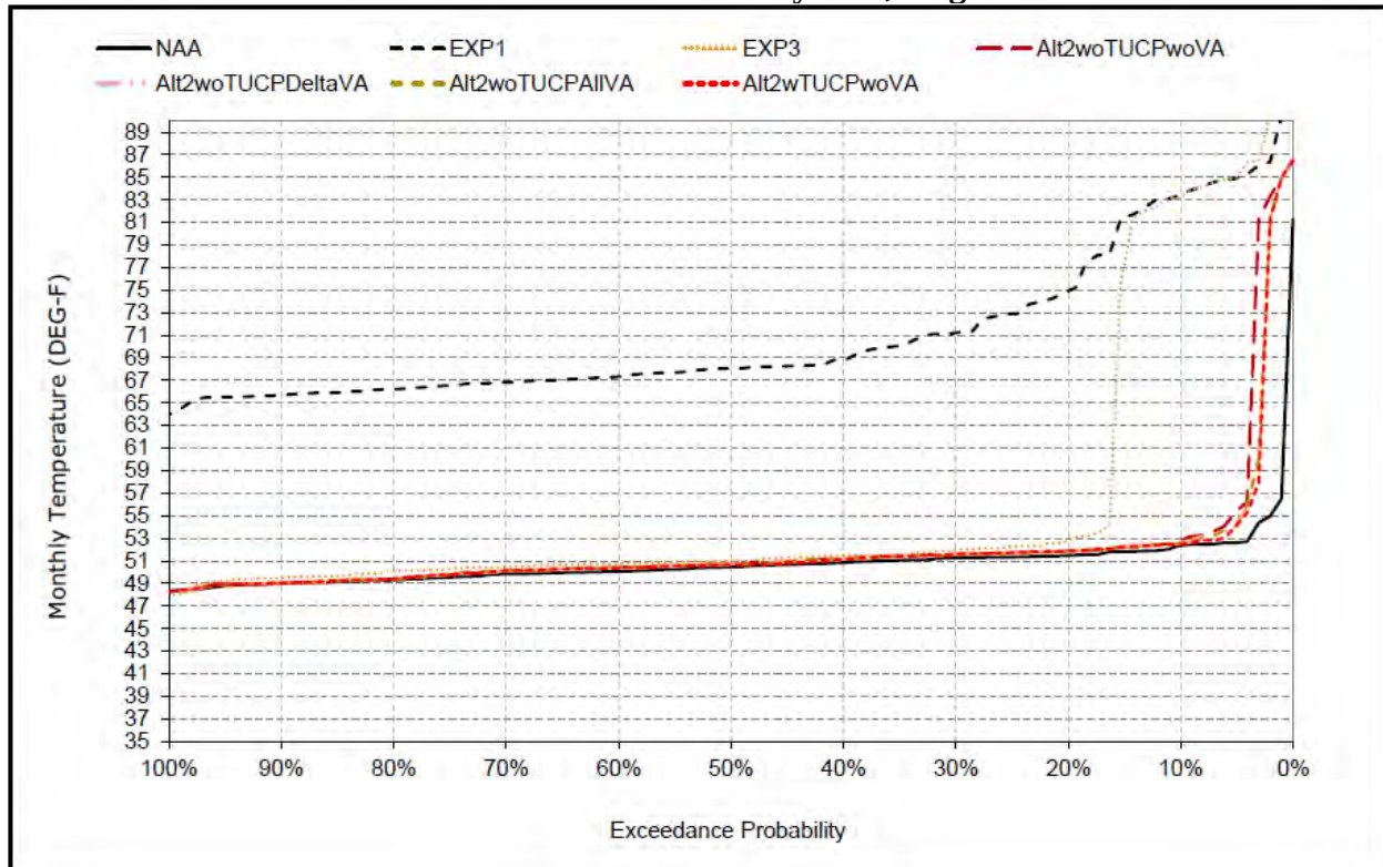
Figure 72. Exceedance plot of modeled water temperatures in Clear Creek in August. The proposed action is represented by Alt2woTUCPwoVA (Alt2v1).
