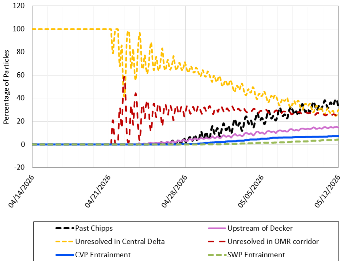
Figure 14. PTM Results for Surface Oriented Particles. OMR Scenario -2,000 cfs. Particles Injected 04/21/2026 at DSM2 Node 99 (Old River)
