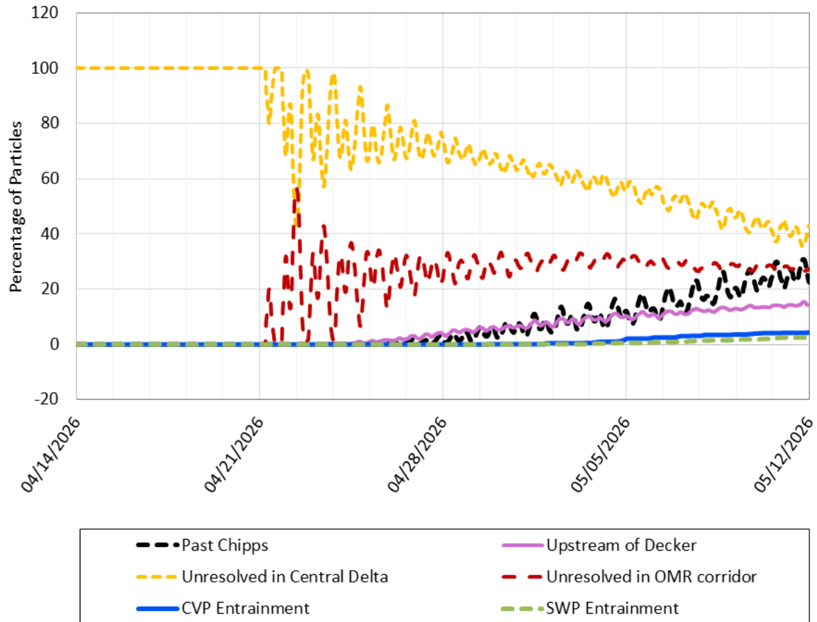
Figure 10. PTM Results for Neutral Particles. OMR Scenario -2,000 cfs. Particles Injected 04/21/2026 at DSM2 Node 99 (Old River)
