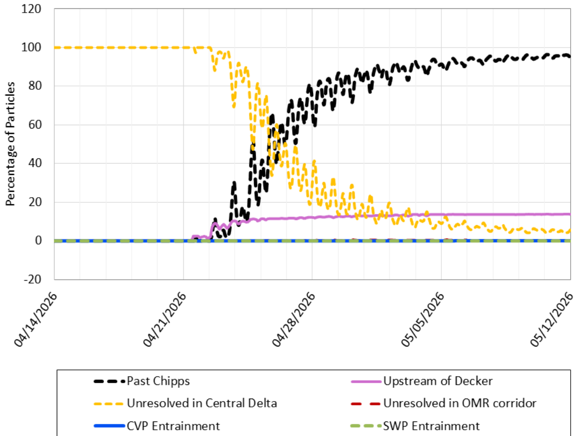
Figure 13. PTM Results for Surface Oriented Particles. OMR Scenario -2,000 cfs. Particles Injected 04/21/2026 at DSM2 Node 469 (Jersey Point)
