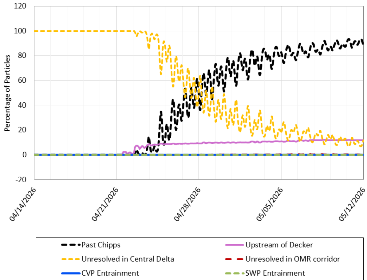
Figure 9. PTM Results for Neutral Particles. OMR Scenario -2,000 cfs. Particles Injected 04/21/2026 at DSM2 Node 469 (Jersey Point)
