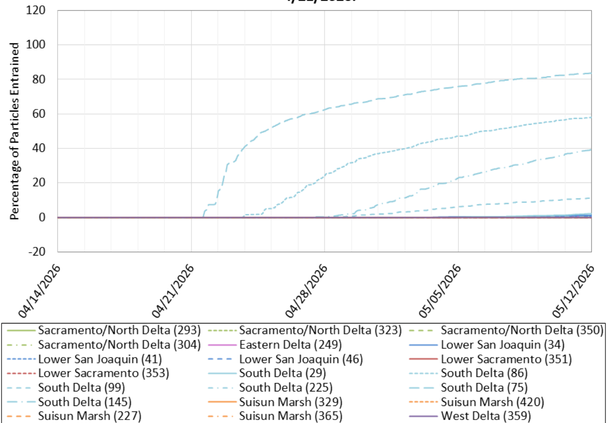
Average PTM Results by Injection Region for Position Oriented Particles Entrained at CVP and SWP. OMR Scenario = -2,000. Particles Injected 4/21/2026.
