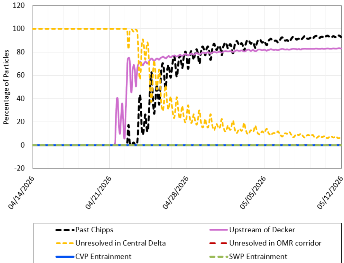
Figure 12. PTM Results for Surface Oriented Particles. OMR Scenario -2,000 cfs. Particles Injected 04/21/2026 at DSM2 Node 350 (Cache Slough)
