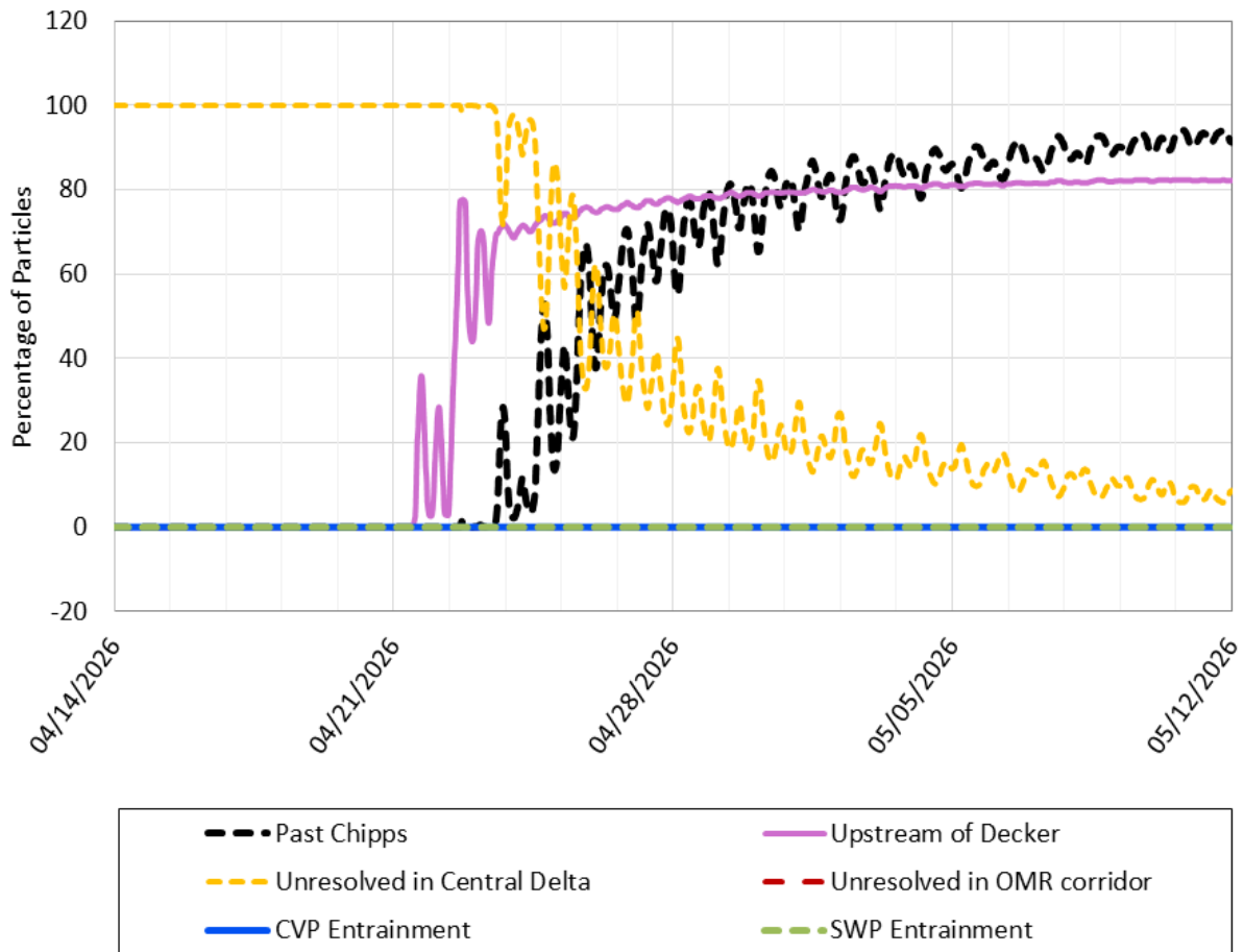
Figure 8. PTM Results for Neutral Particles. OMR Scenario -2,000 cfs. Particles Injected 04/21/2026 at DSM2 Node 350 (Cache Slough)
