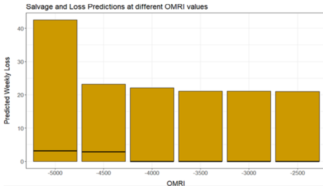
Figure 6. Salvage and Loss Predictions at Different OMRI Values
