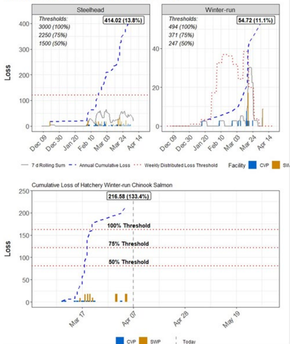
Figure 3. WY 2025 Loss for Steelhead and Winter-run Chinook Salmon
