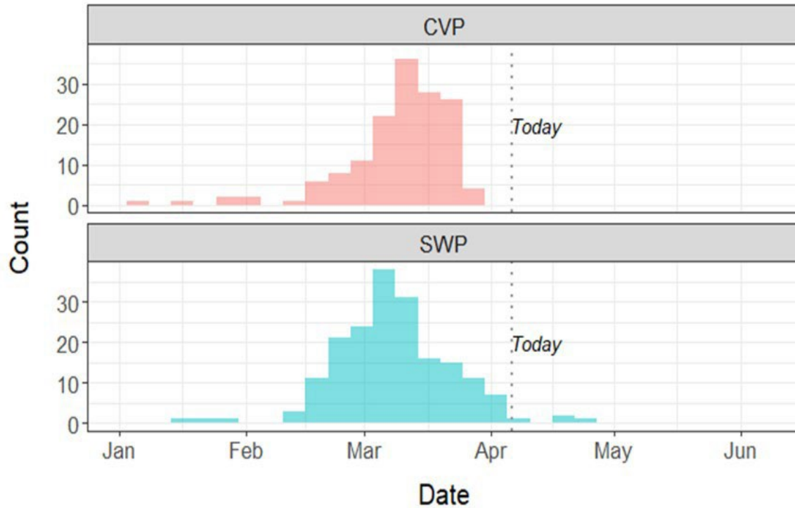
Figure 2. Distribution of genetically confirmed winter-run salvaged at the Central Valley Project (CVP) and State water Project (SWP) from 2011-2024.
