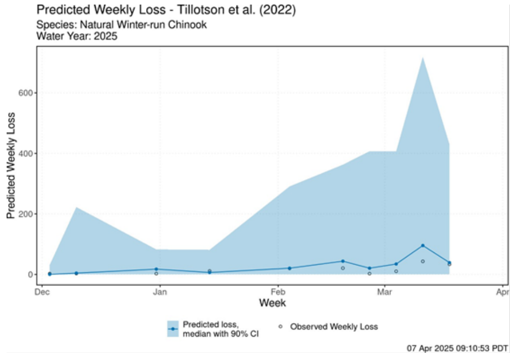
Figure 5. Predicted weekly winter-run Chinook salmon loss through the Tillotson et al (2022) model.
