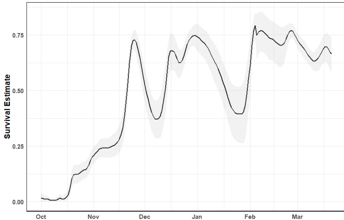
Figure 1. Temporal variation in overall survival estimates for outmigrating juvenile winter-run Chinook Salmon in the Delta with 80% credible intervals (shaded region) from October to April 11.
