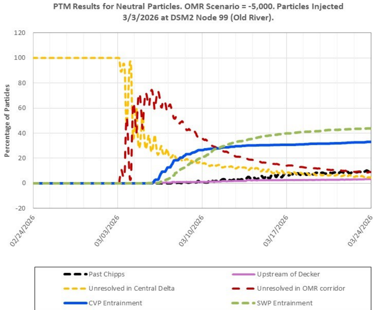
Figure 20: PTM Results for Neutral Particles at Old River, OMR Scenario -5,000
