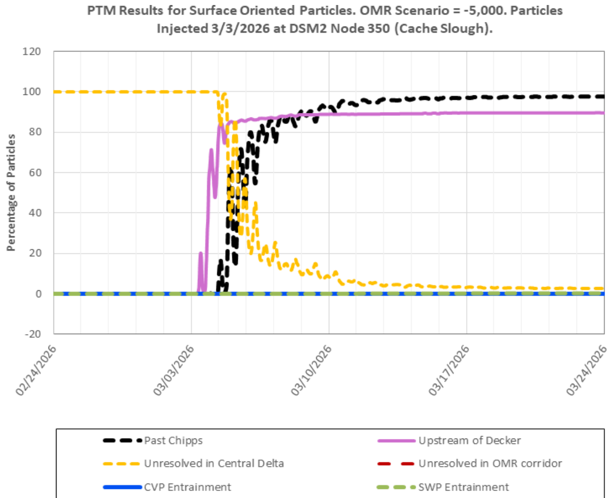
Figure 28: PTM Results for Surface Oriented Particles at Cache Slough Confluence, OMR Scenario -5,000
