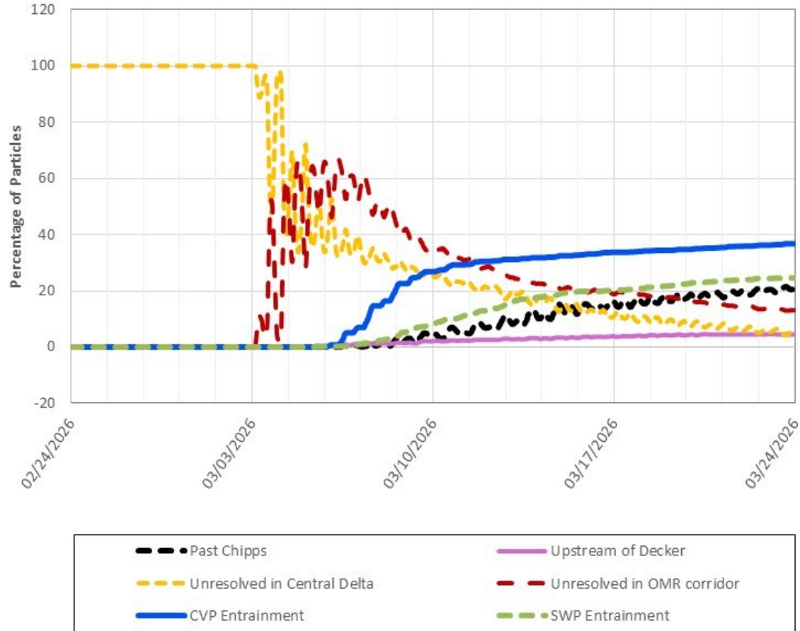
PTM Results for Surface Oriented Particles. OMR Scenario = -3,500. Particles Injected 3/3/2026 at DSM2 Node 99 (Old River).
