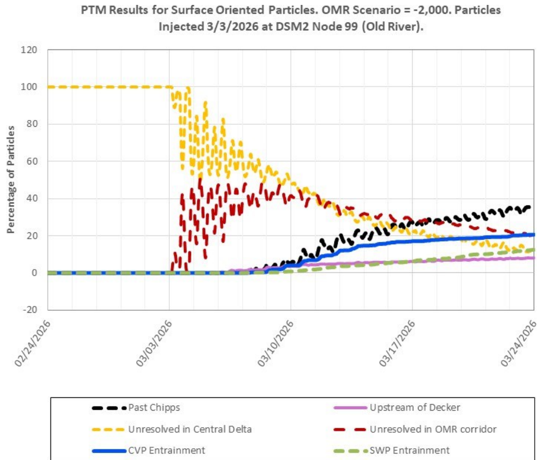
Figure 38: PTM Results for Surface Oriented Particles at Old River, OMR Scenario -2,000
