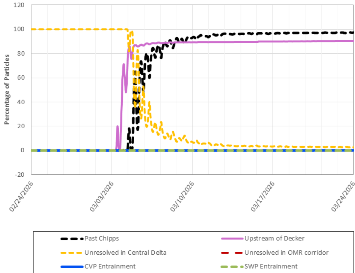
PTM Results for Surface Oriented Particles. OMR Scenario = -2,000. Particles Injected 3/3/2026 at DSM2 Node 350 (Cache Slough).
