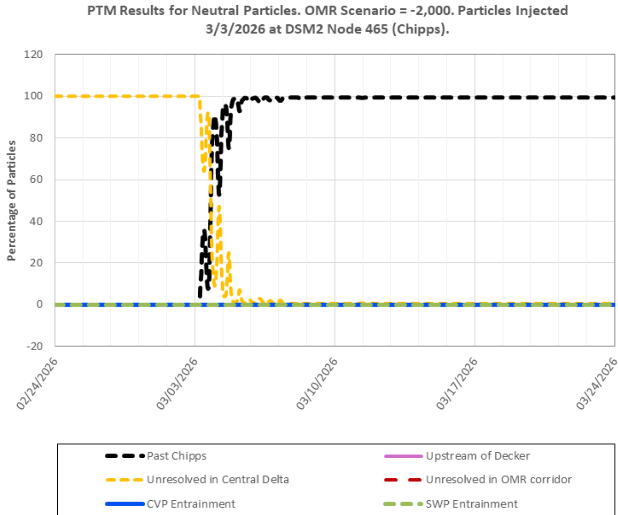
Figure 10: PTM Results for Neutral Particles at Chippis Island, OMR Scenario -2,000
