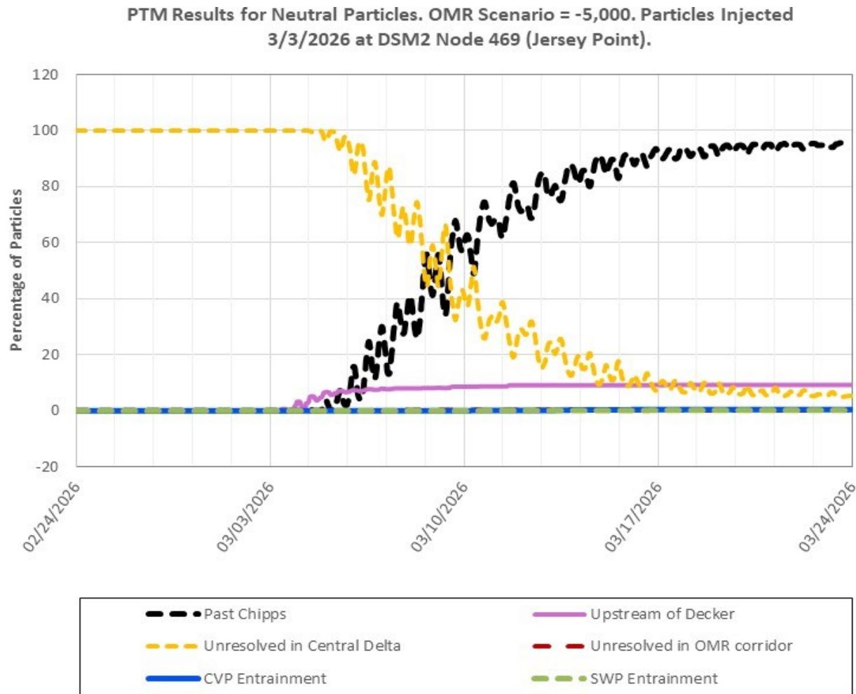
Figure 16: PTM Results for Neutral Particles at Jersey Point, OMR Scenario -5,000
