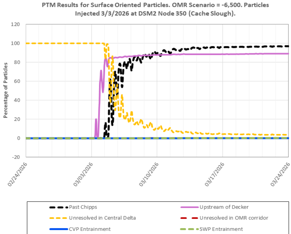
Figure 27: PTM Results for Surface Oriented Particles at Cache Slough Confluence, OMR Scenario -6,500
