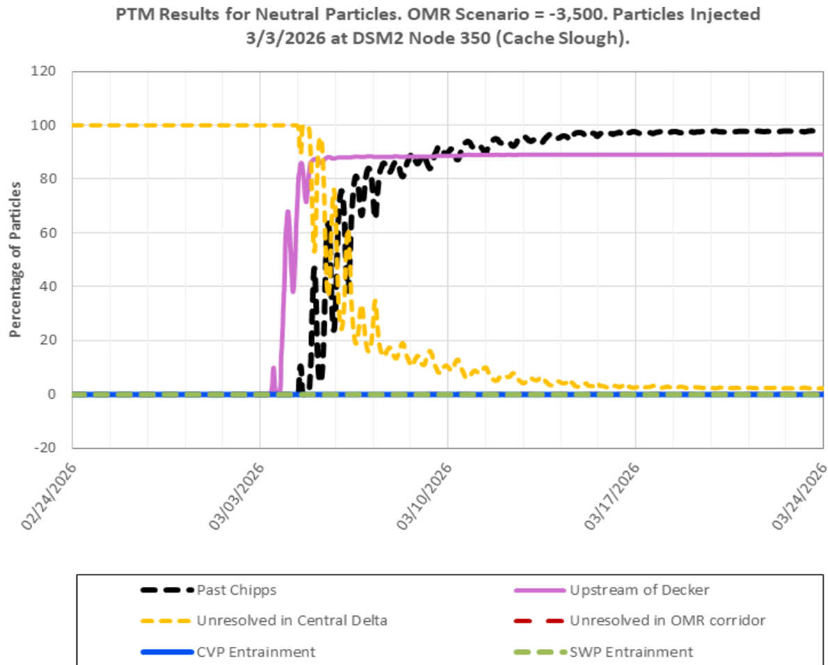
Figure 13: PTM Results for Neutral Particles at Cache Slough Confluence, OMR Scenario -3,500
