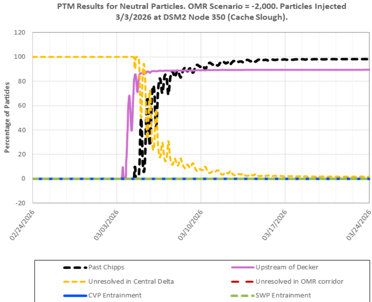
Figure 14: PTM Results for Neutral Particles at Cache Slough Confluence, OMR Scenario -2,000
