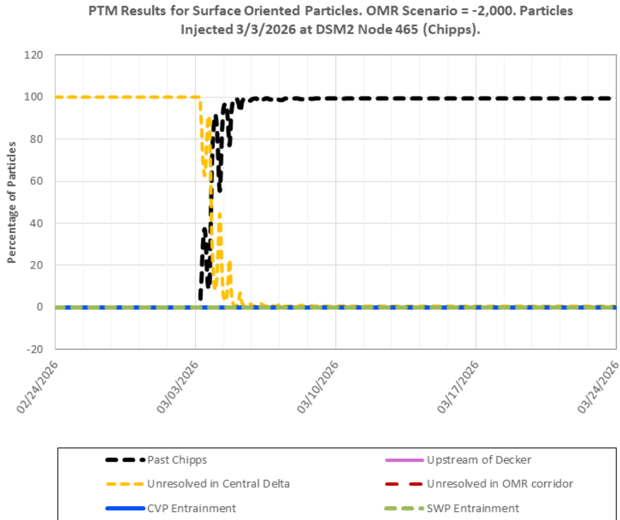
Figure 26: PTM Results for Surface Oriented Particles at Chippis Island, OMR Scenario -2,000
