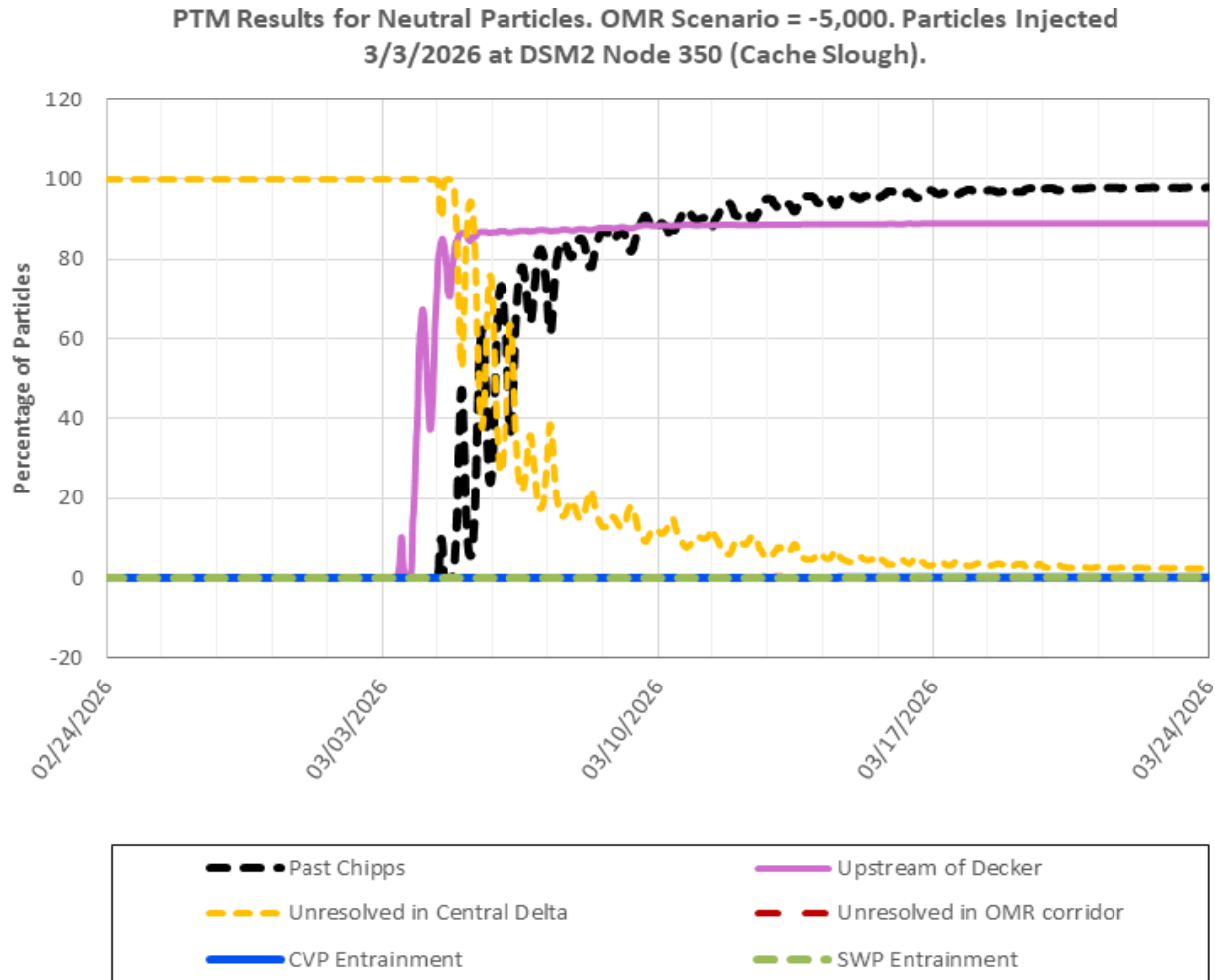
Figure 12: PTM Results for Neutral Particles at Cache Slough Confluence, OMR Scenario -5,000
