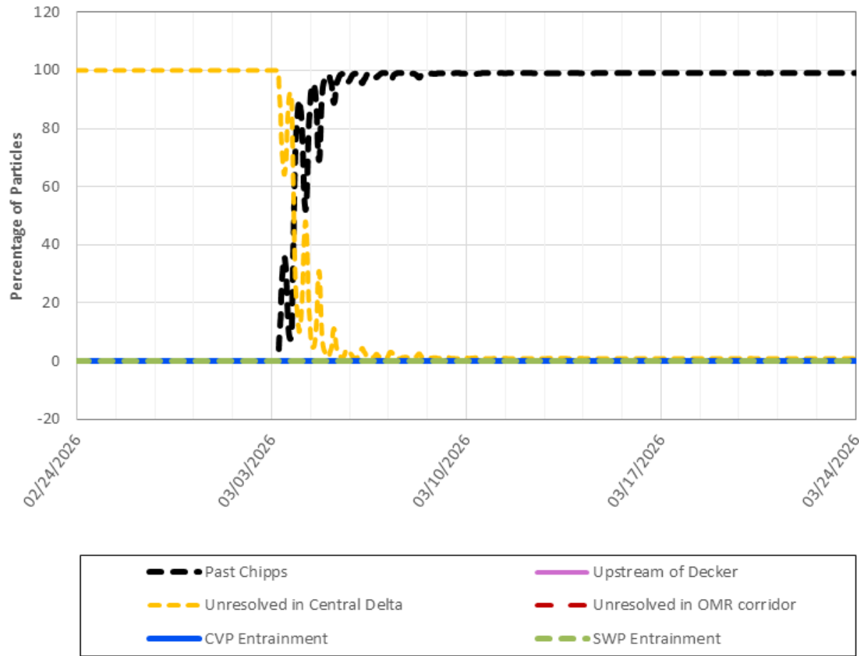
PTM Results for Neutral Particles. OMR Scenario = -6,500. Particles Injected 3/3/2026 at DSM2 Node 465 (Chippis).
