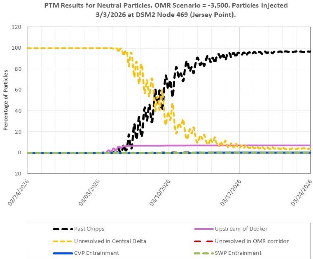
Figure 17: PTM Results for Neutral Particles at Jersey Point, OMR Scenario -3,500
