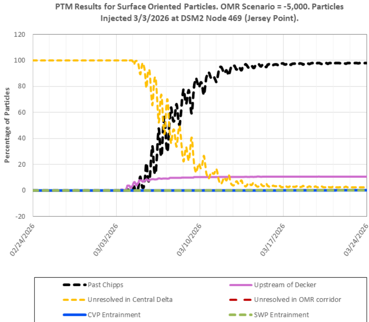
Figure 32: PTM Results for Surface Oriented Particles at Jersey Point, OMR Scenario -5,000
