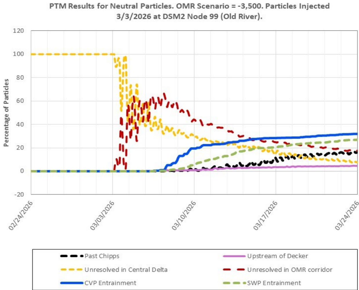
Figure 21: PTM Results for Neutral Particles at Old River, OMR Scenario -3,500
