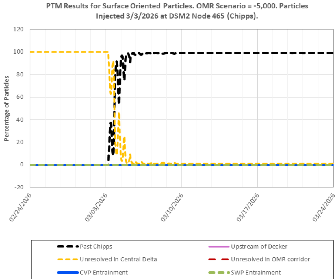
Figure 24: PTM Results for Surface Oriented Particles at Chipps Island, OMR Scenario -5,000
