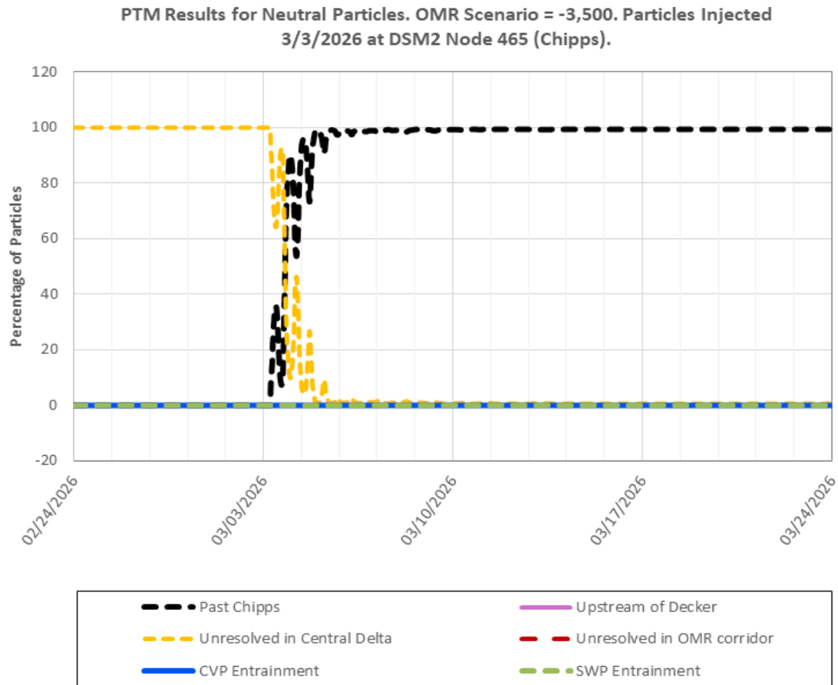
Figure 9: PTM Results for Neutral Particles at Chippis Island, OMR Scenario -3,500
