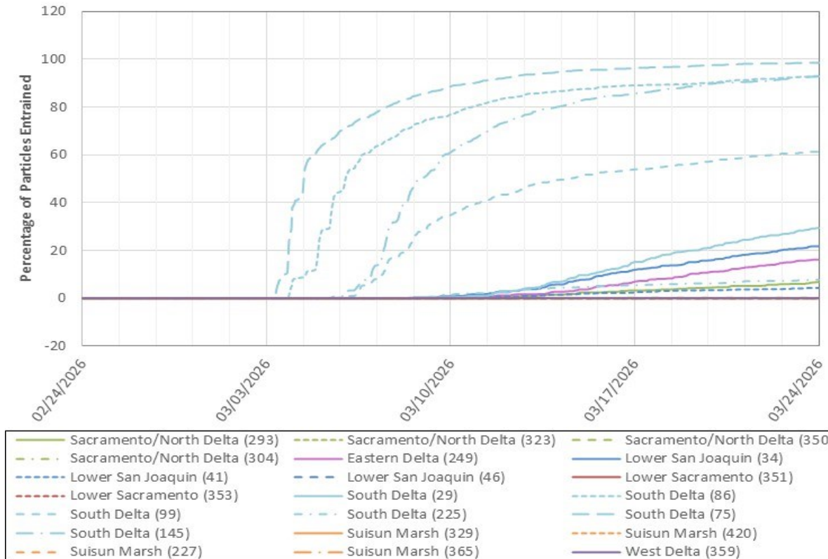
Average PTM Results by Injection Region for Position Oriented Particles Entrained at CVP and SWP. OMR Scenario = -3,500. Particles Injected 3/3/2026.
