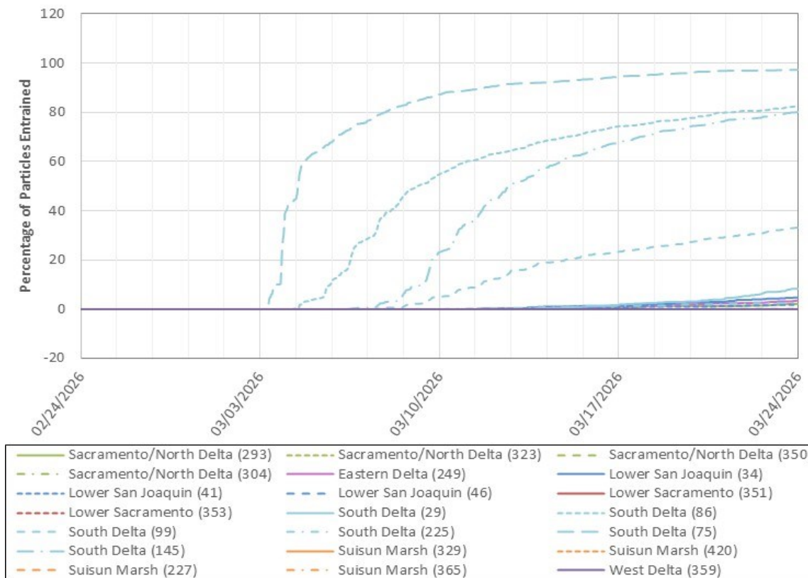
Average PTM Results by Injection Region for Position Oriented Particles Entrained at CVP and SWP. OMR Scenario = -2,000. Particles Injected 3/3/2026.
