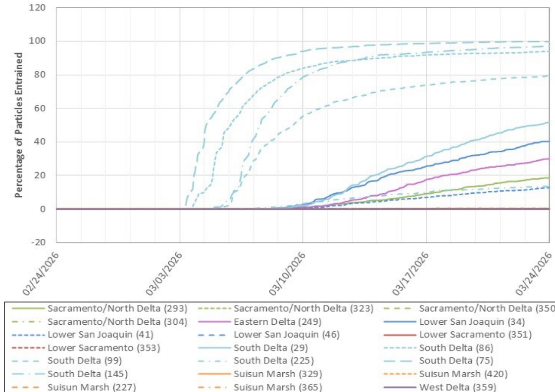
Average PTM Results by Injection Region for Position Oriented Particles Entrained at CVP and SWP. OMR Scenario = -5,000. Particles Injected 3/3/2026.
