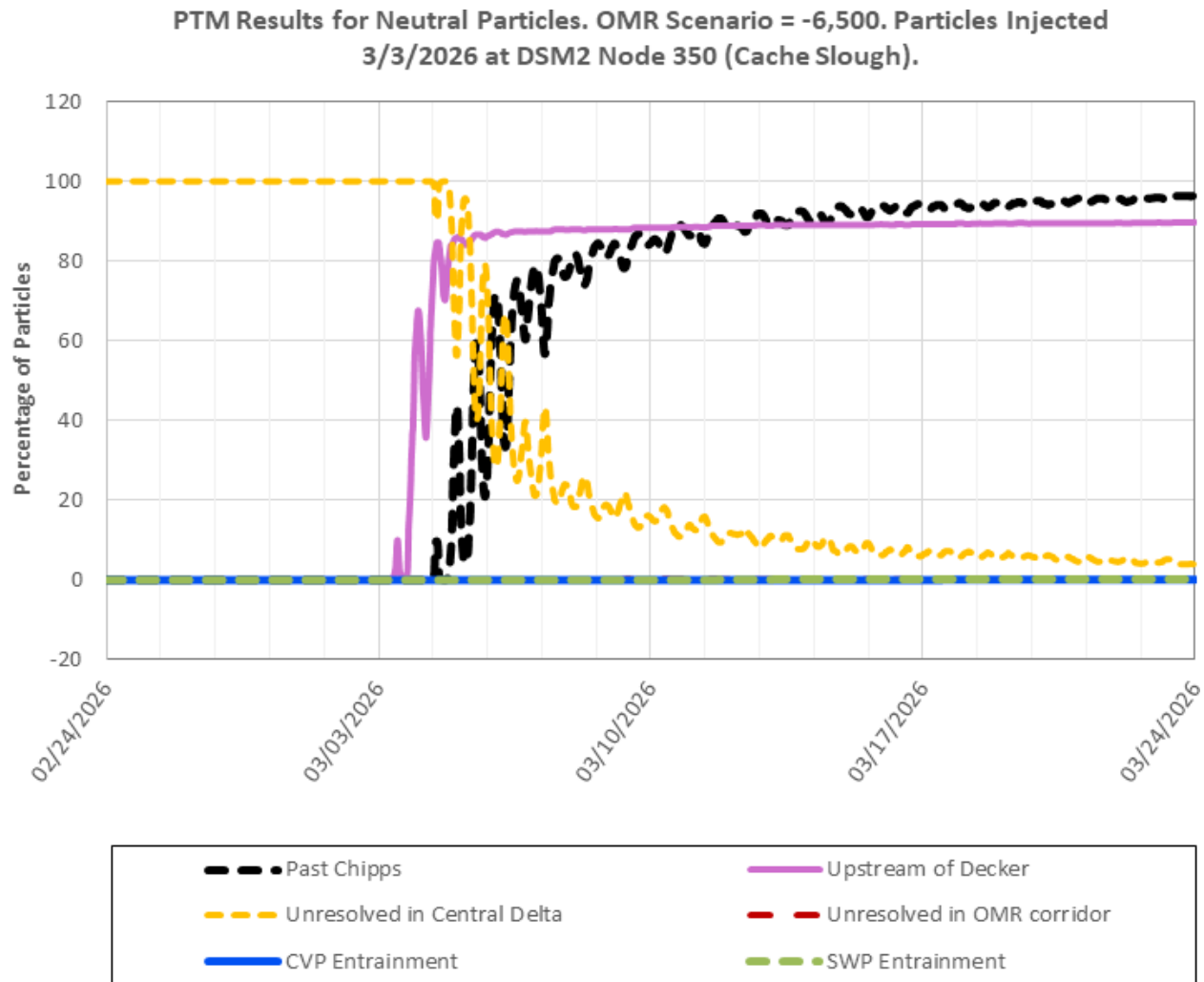
Figure 11: PTM Results for Neutral Particles at Cache Slough Confluence, OMR Scenario -6,500
