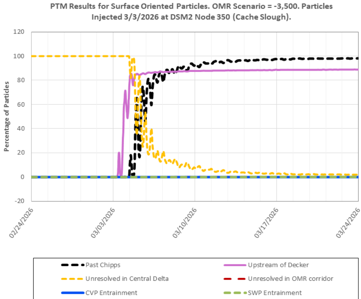
Figure 29: PTM Results for Surface Oriented Particles at Cache Slough Confluence, OMR Scenario -3,500
