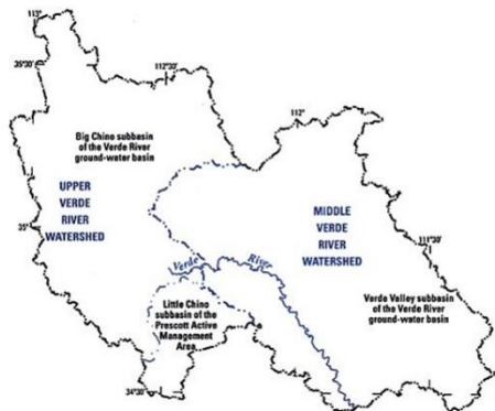
Figure 2: Upper Verde River watershed central Arizona. The Big Chino and Little Chino subbasins contribute to the upper most section of the Verde River. The Verde Valley sub basin contributes to below Hell Canyon. Credit Arizona Department of Water Resources (2009).
