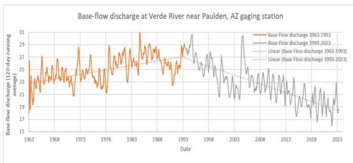
Figure 4 Baseflow decline in the Upper Verde River since 1993. Data taken from the USGS stream gauge at Paulden, Arizona. Credit Joel Unema, USGS URL: https://waterdata.usgs.gov/nwis/monthly?
