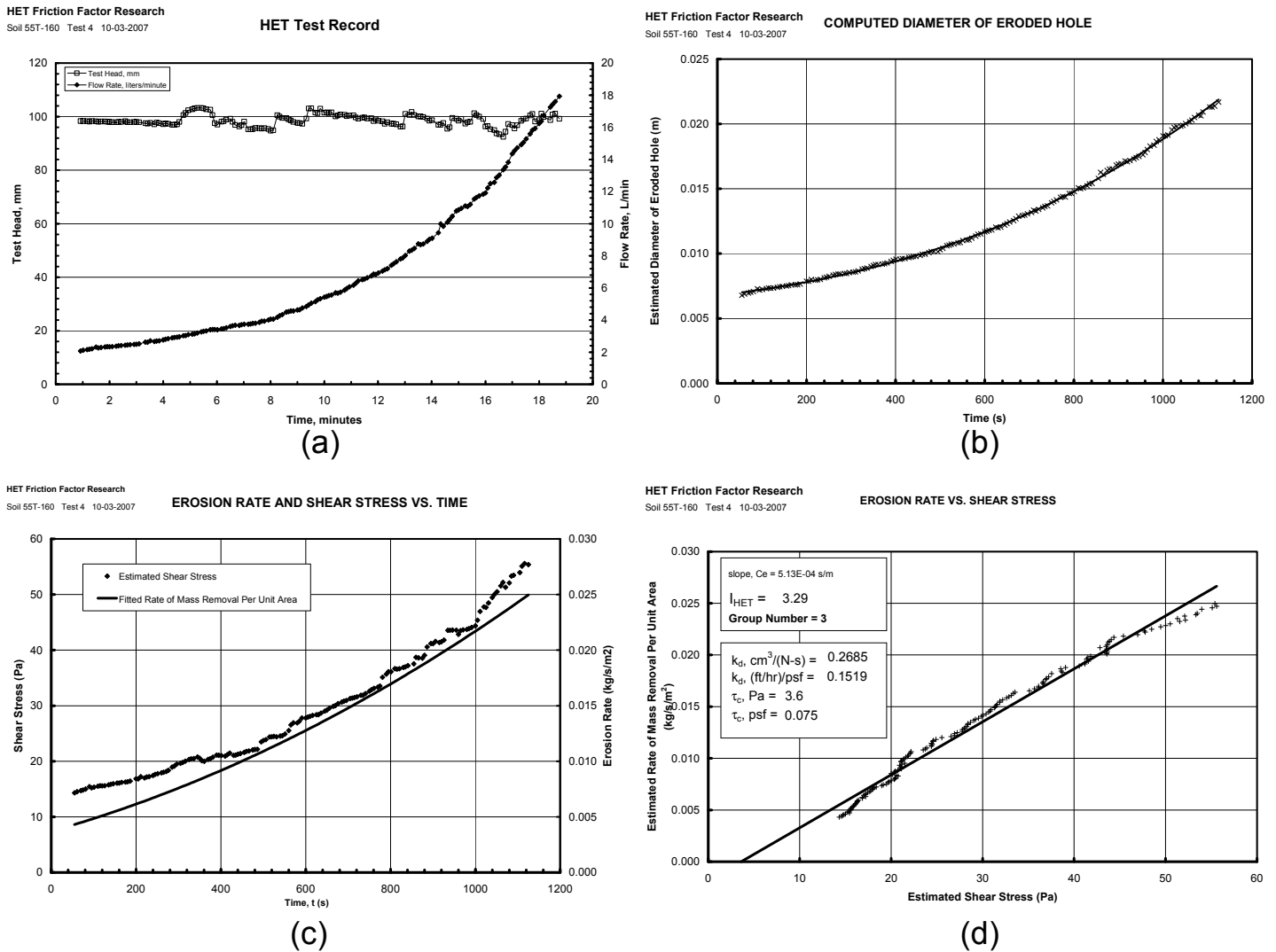
Figure 5. —An HET conducted at a test head that caused immediate progressive erosion. Flow was turbulent throughout this test ( Re = 6,250 to 17,000 ).
